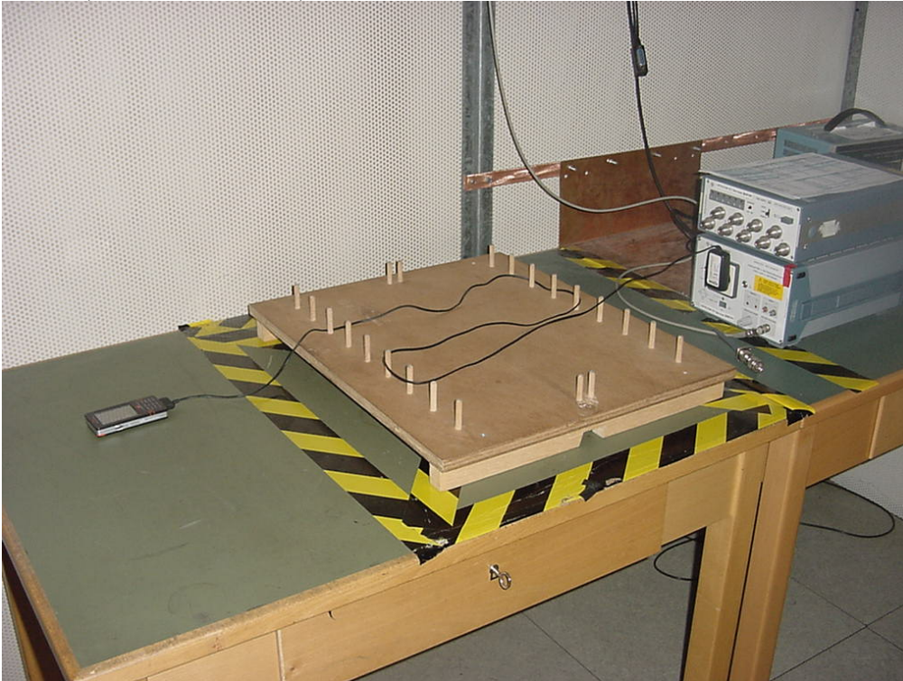
Photo 3 (Conducted Emissions):
