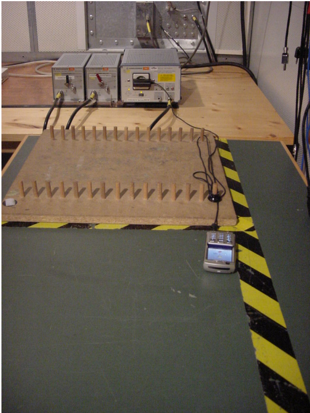
Photo 3: Conducted Emissions
