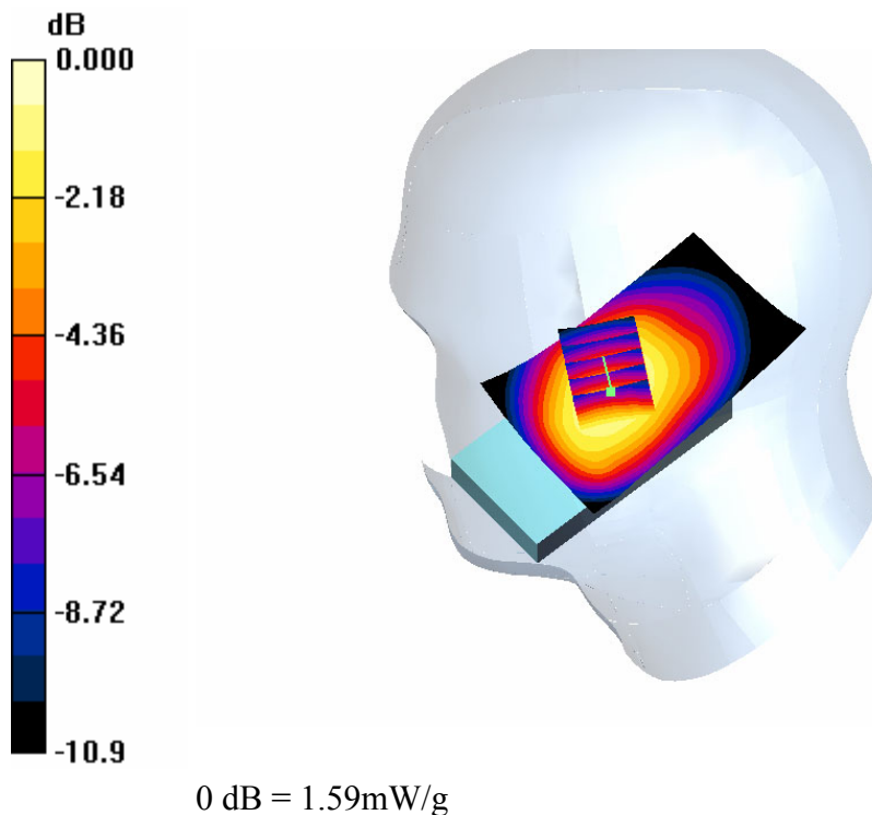
(a) Distribution of maximum SAR in GSM900 mode giving the maximum 10g averaged SAR. Measured against the right hand side phantom for the cheek phone position.
