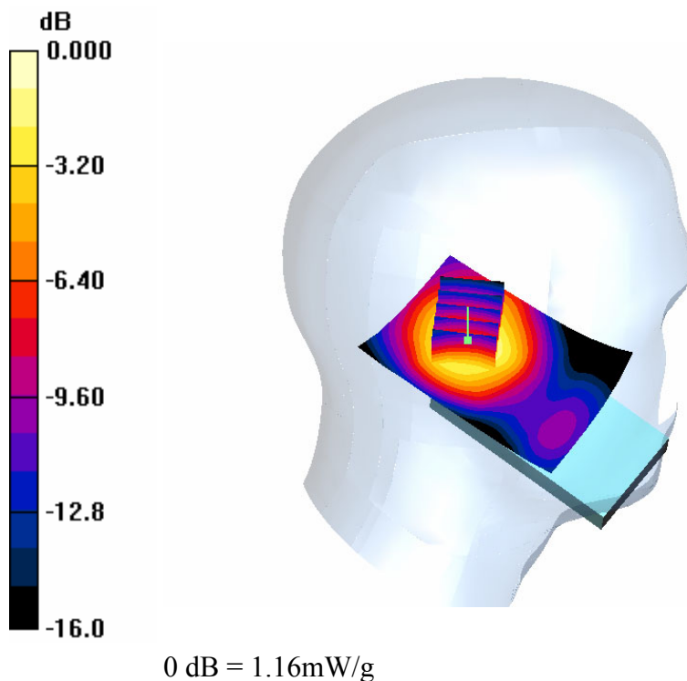
(k) Distribution of maximum SAR in UMTS mode giving the maximum 10g averaged SAR. Measured against the left hand side phantom for the tilt phone position.
