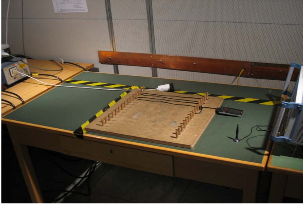
Photo 4: Conducted Emissions
