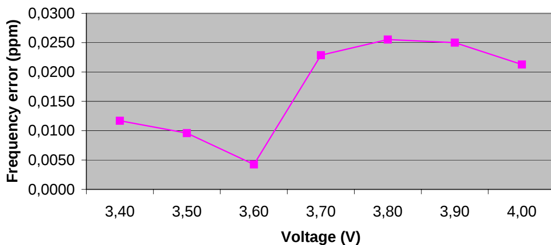
Frequency Error vs. Voltage
