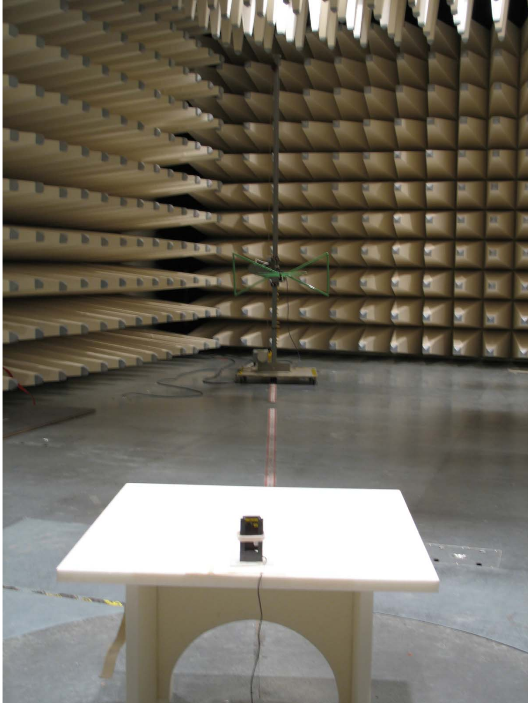
Photo 2: Radiated Emissions
