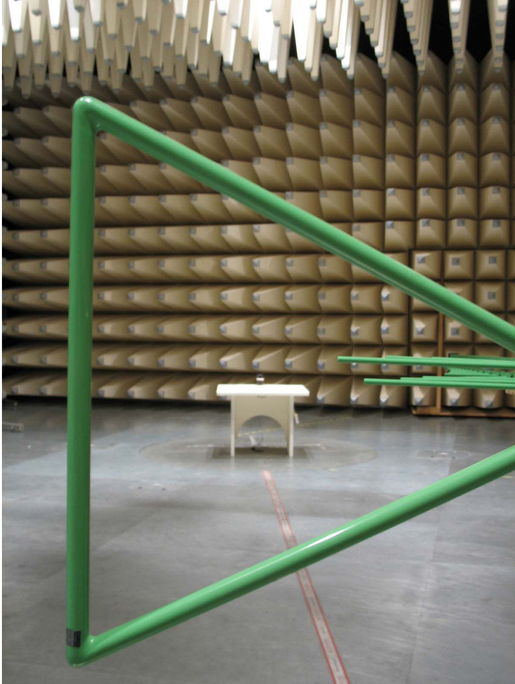
Photo 3: Radiated Emissions
