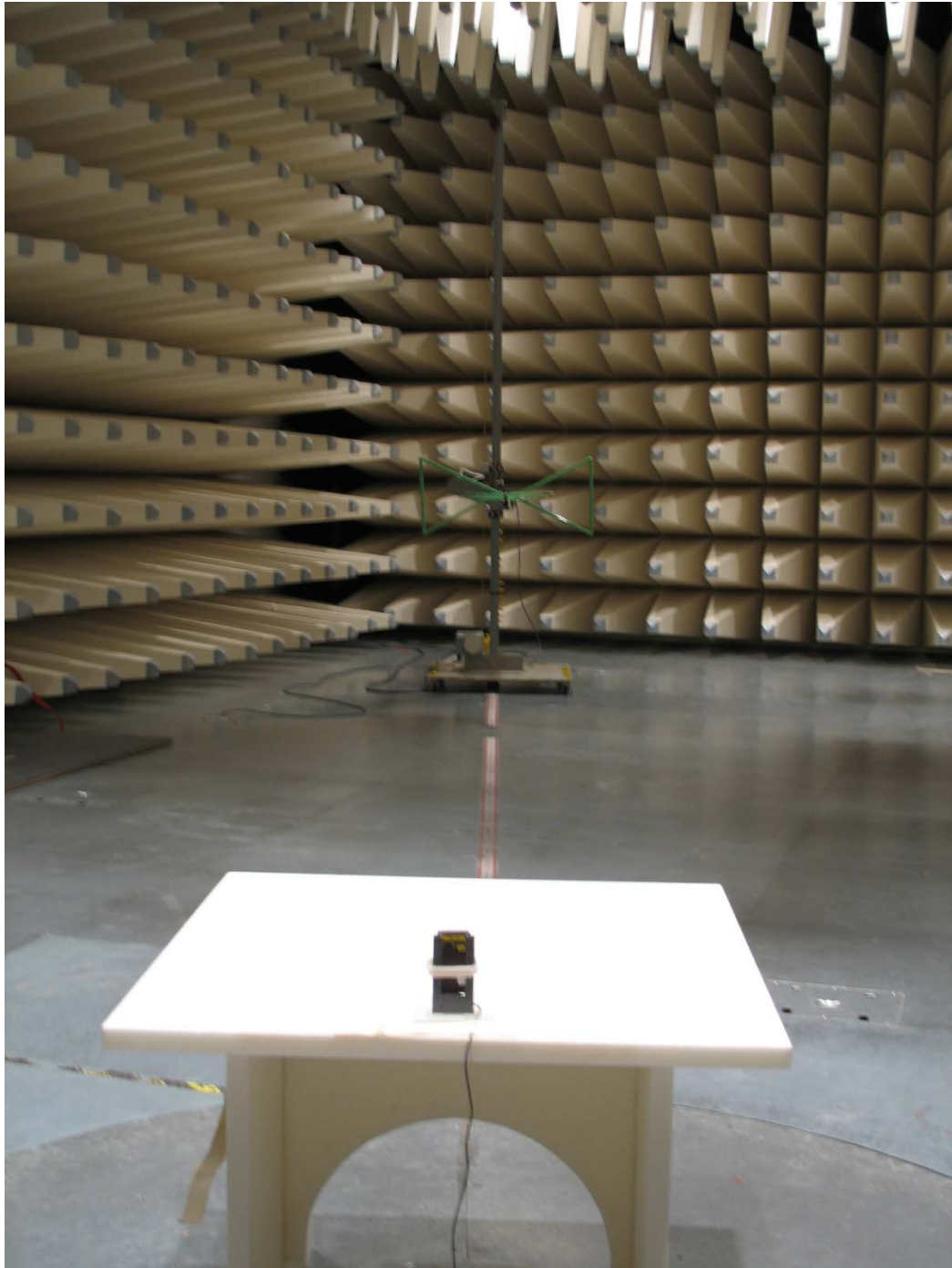
Photo 2: Radiated Emissions
