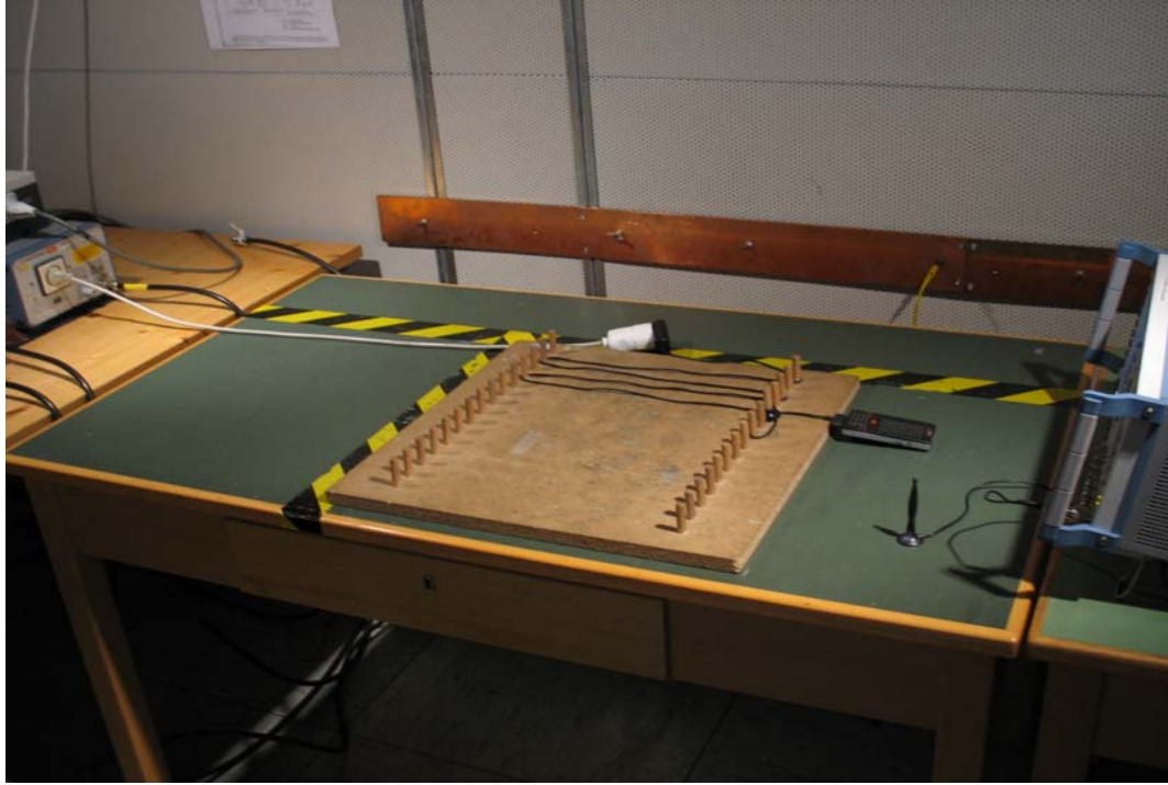
Photo 4: Conducted Emissions
