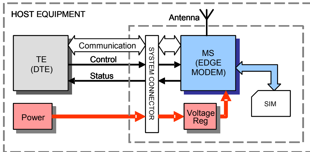
Figure 2-2Figure 2-2 Interface between Daughter Card and Application
