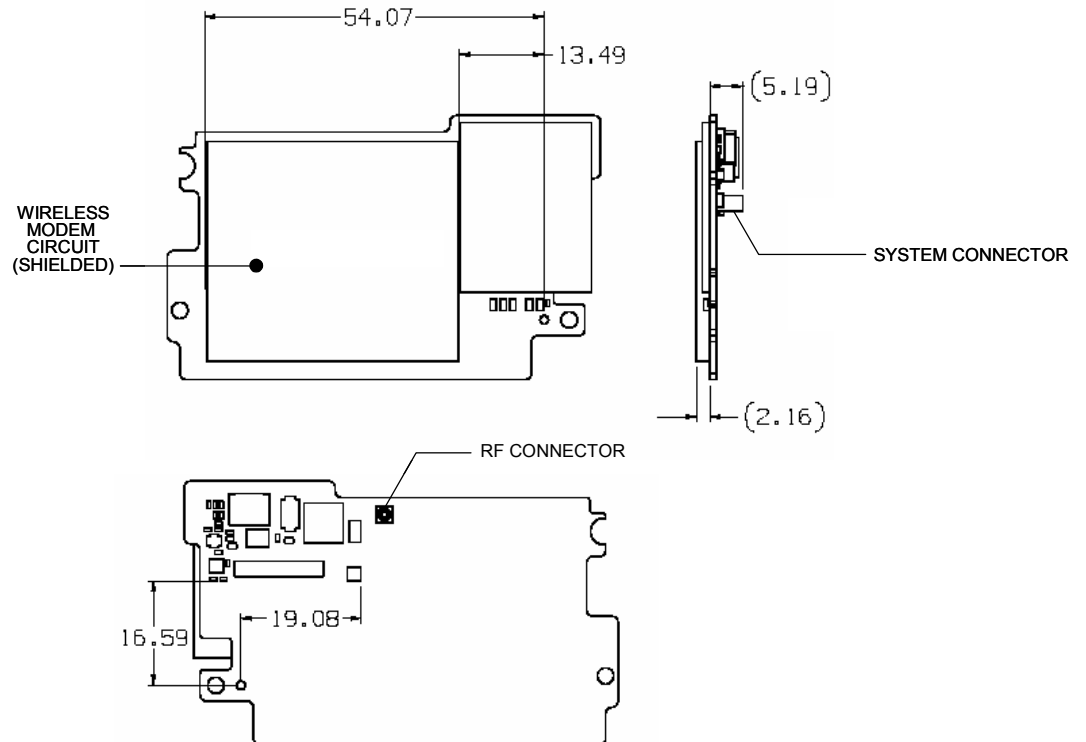
Figure 3-1 Layout Detail (reference only)
