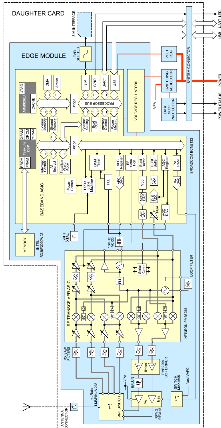
Figure 2-3 EDGE Daughter Card Functional Block Diagram
