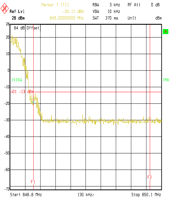
Title: Transmitter Radiated Band Edges Top Band Comment A: 70868JD05 Sony Ericsson Mobiles GC89 FCC Part 22 Date: 14.APR.2005 19:08:03
