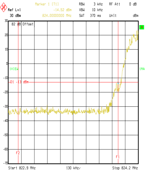
Title: Transmitter Radiated Band Edges Bottom Band Comment A: 70868JD05 Sony Ericsson Mobiles GC89 FCC Part 22 Date: 14.APR.2005 19:11:40
