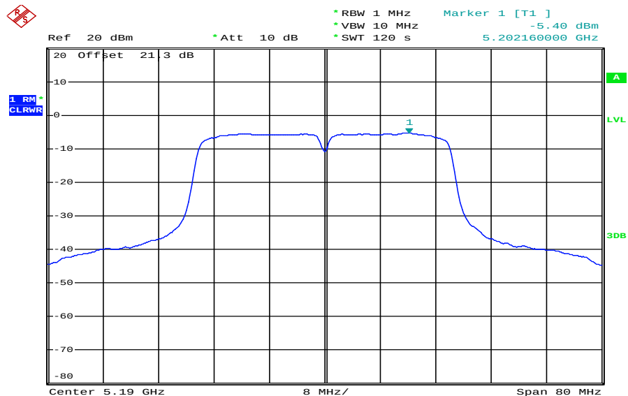
Plot 1: 5190 MHz
