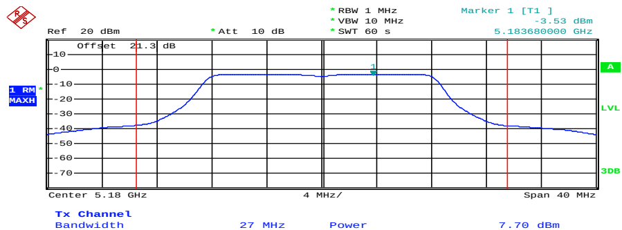
Plot 1: 5180 MHz
