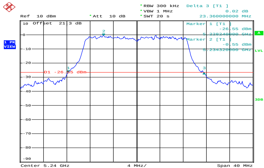
Plot 2: 5240 MHz
