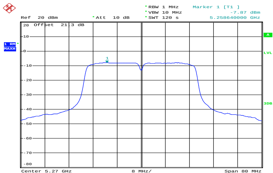
Plot 3: 5270 MHz
