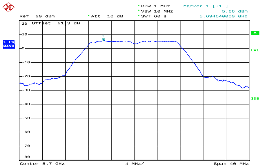
Plot 7: 5700 MHz
