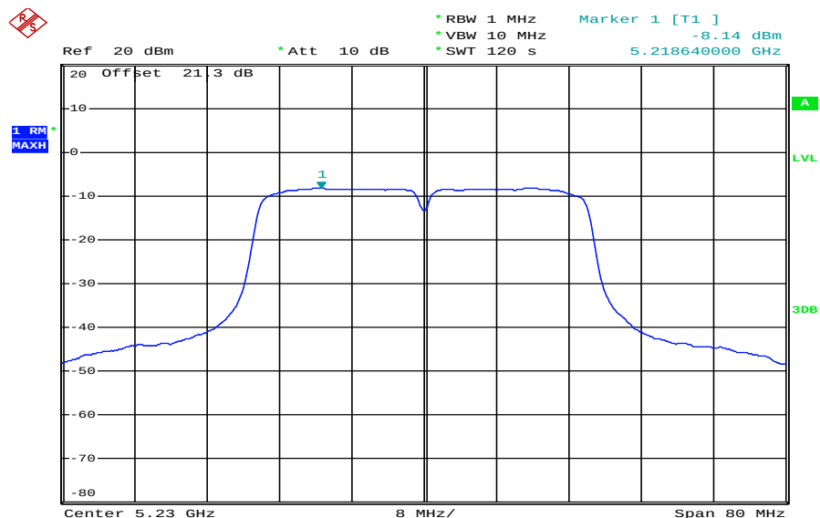
Plot 2: 5230 MHz
