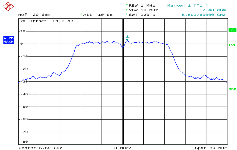
Plot 6: 5590 MHz
