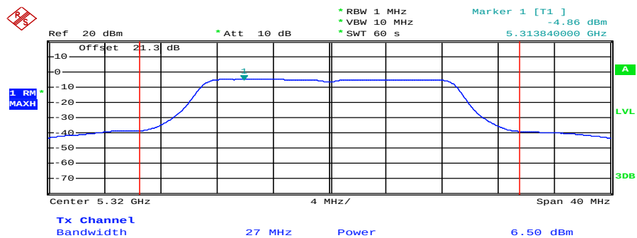
Plot 4: 5320 MHz
