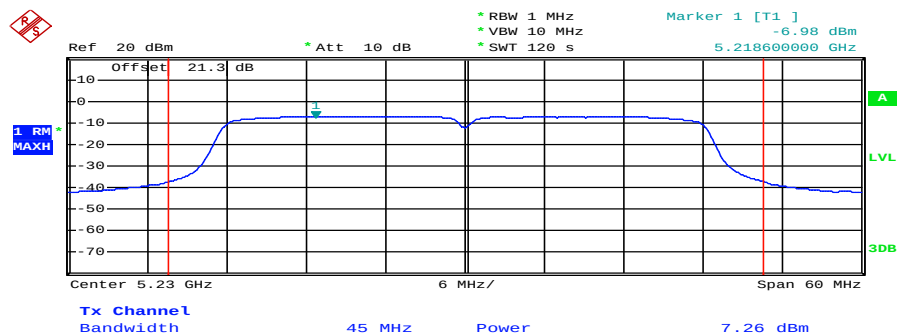
Plot 2: 5230 MHz
