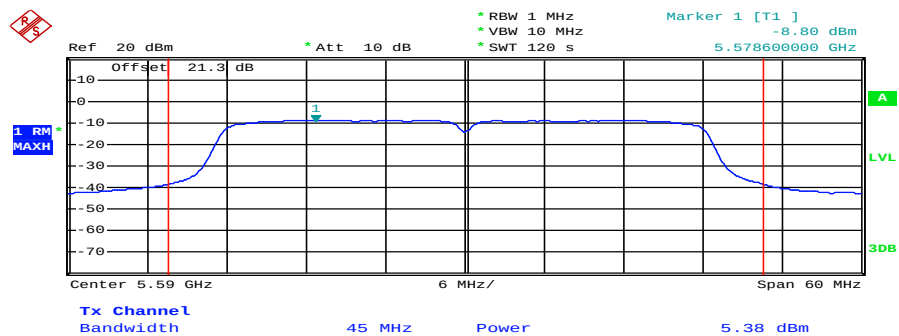
Plot 6: 5590 MHz
