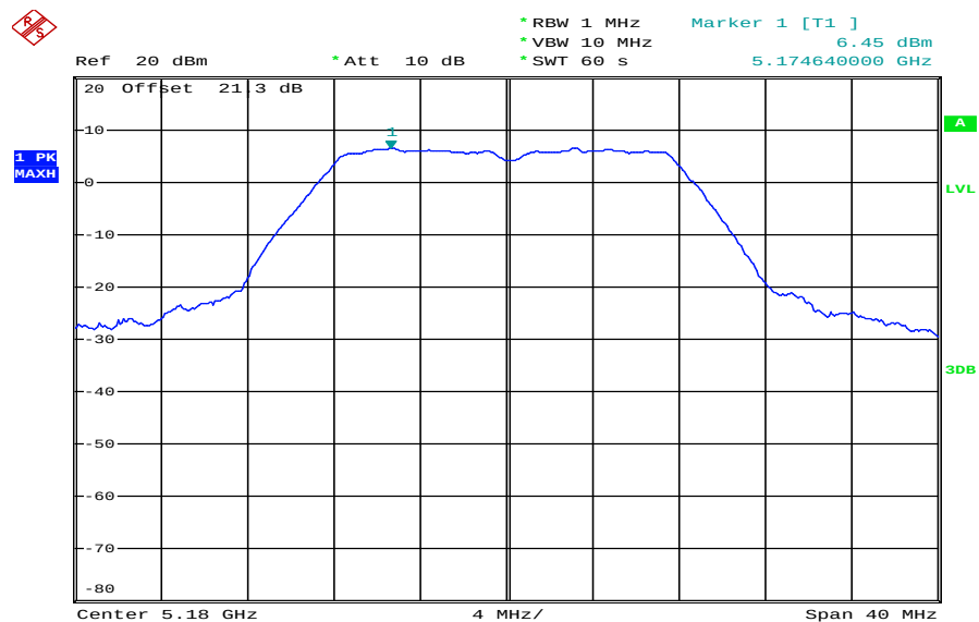
Plot 1: 5180 MHz
