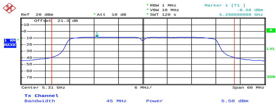
Plot 4: 5310 MHz
