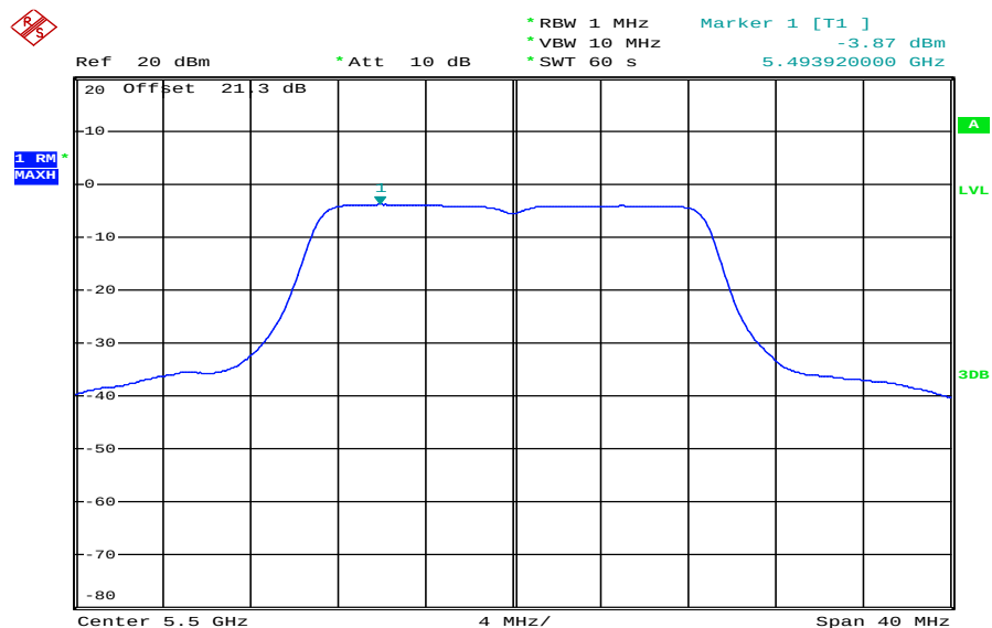
Plot 5: 5500 MHz
