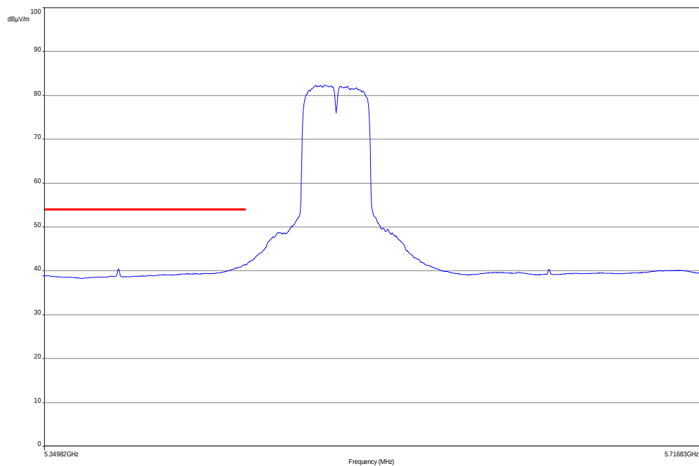
Plot 6: lower band edge, vertical & horizontal polarization (n HT 40 mode), channel 100
