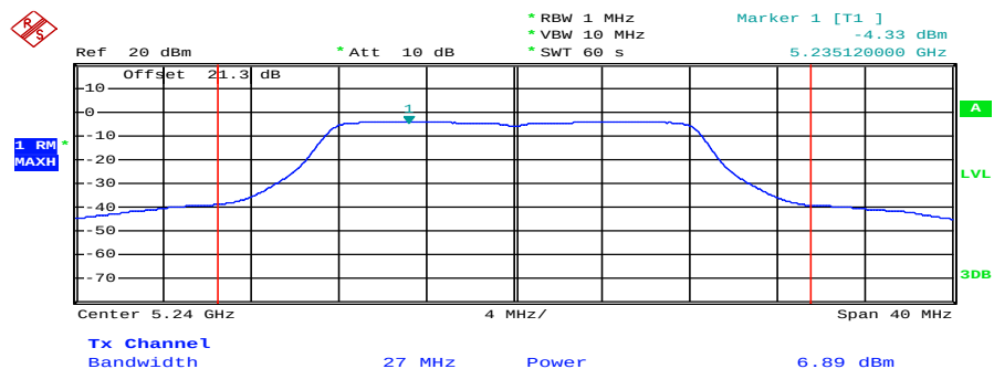
Plot 2: 5240 MHz
