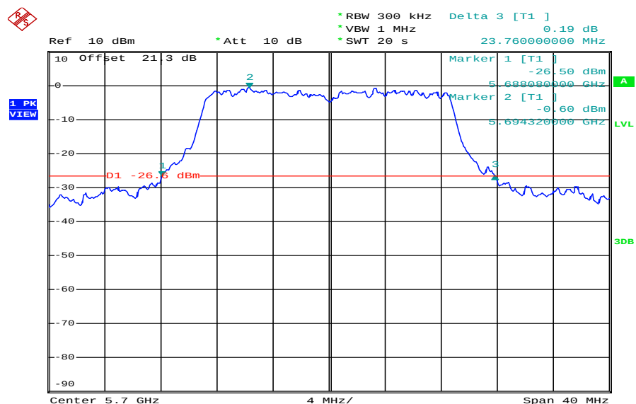
Plot 7: 5700 MHz
