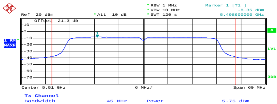
Plot 5: 5510 MHz
