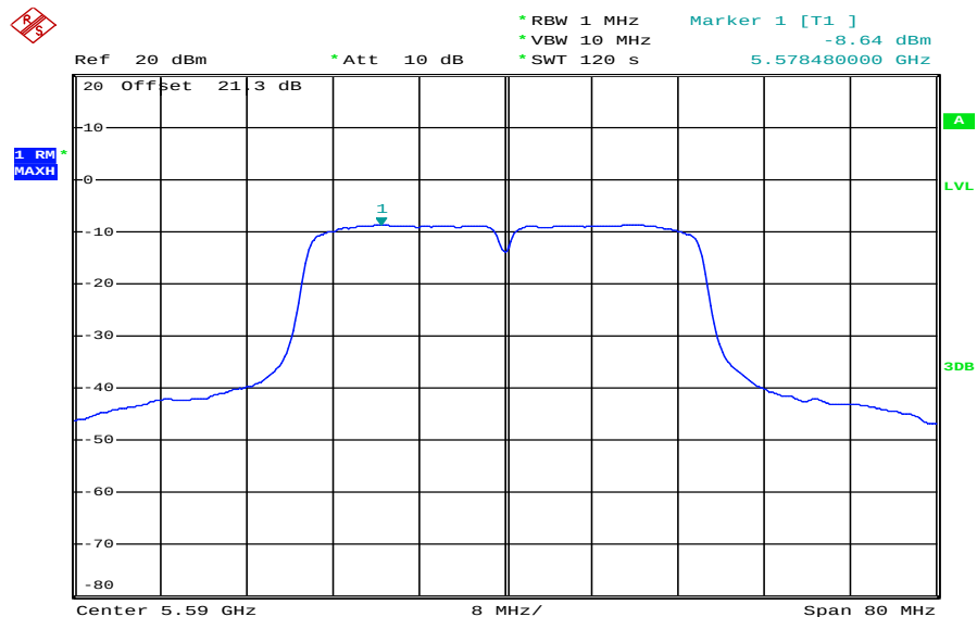
Plot 6: 5590 MHz
