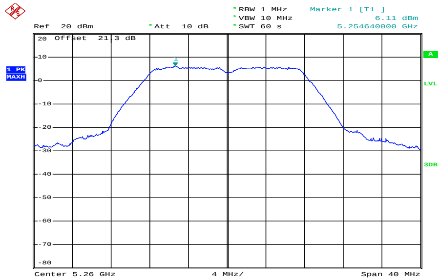
Plot 3: 5260 MHz
