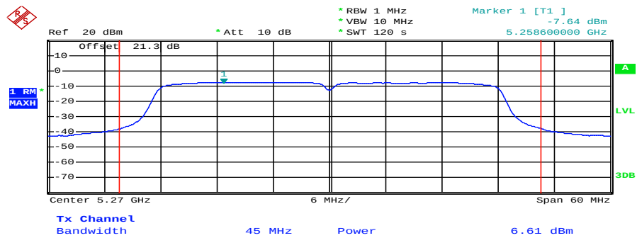
Plot 3: 5270 MHz
