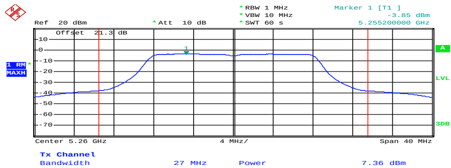
Plot 3: 5260 MHz
