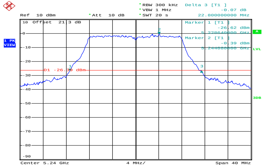
Plot 2: 5240 MHz
