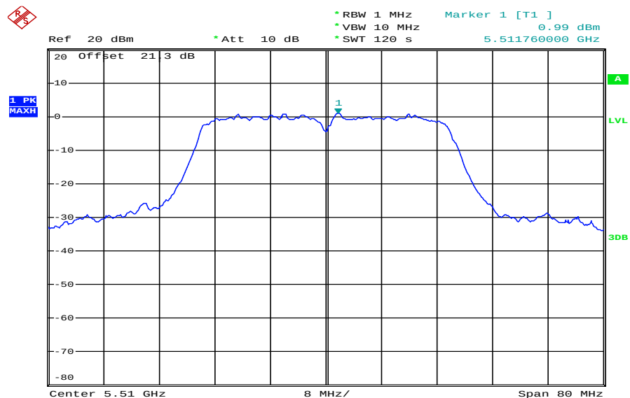
Plot 5: 5510 MHz
