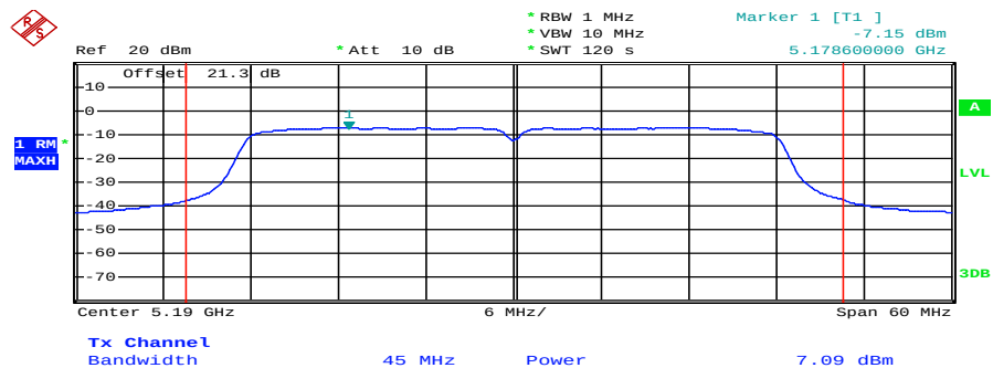
Plot 1: 5190 MHz
