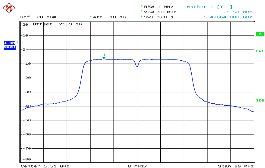
Plot 5: 5510 MHz
