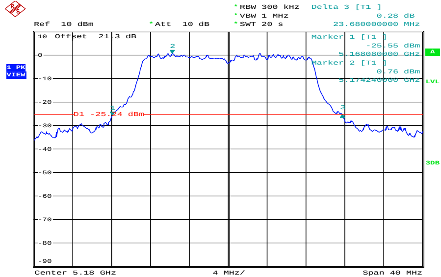
Plot 1: 5180 MHz
