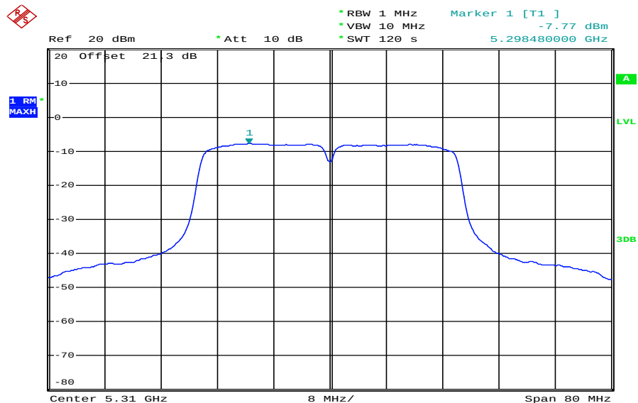
Plot 4: 5310 MHz
