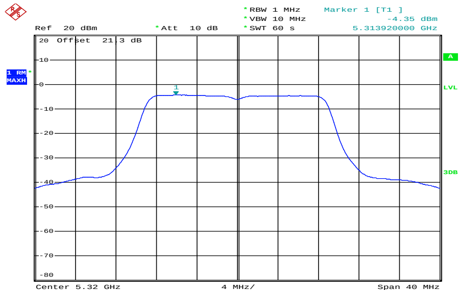
Plot 4: 5320 MHz
