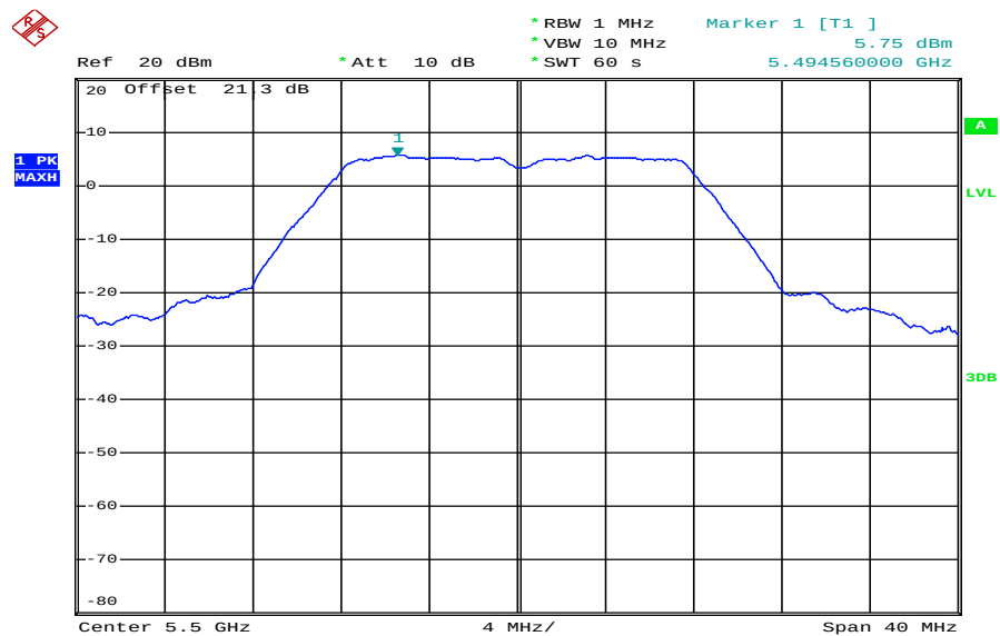
Plot 5: 5500 MHz
