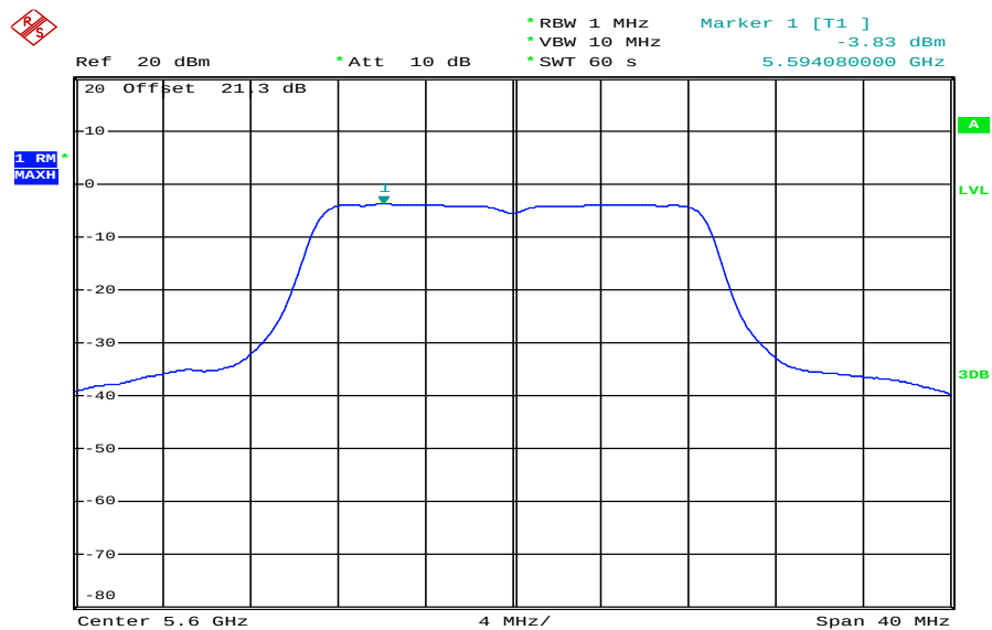
Plot 6: 5600 MHz
