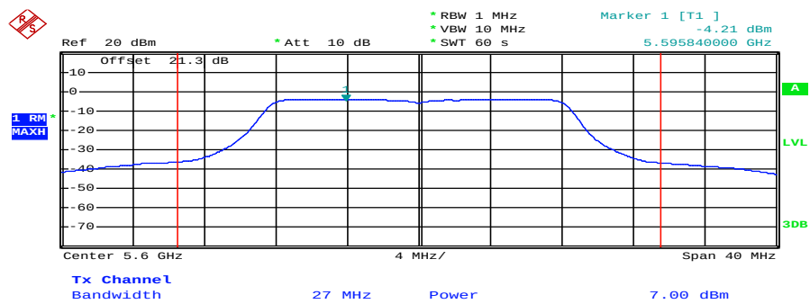
Plot 6: 5600 MHz
