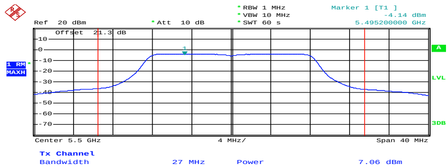
Plot 5: 5500 MHz
