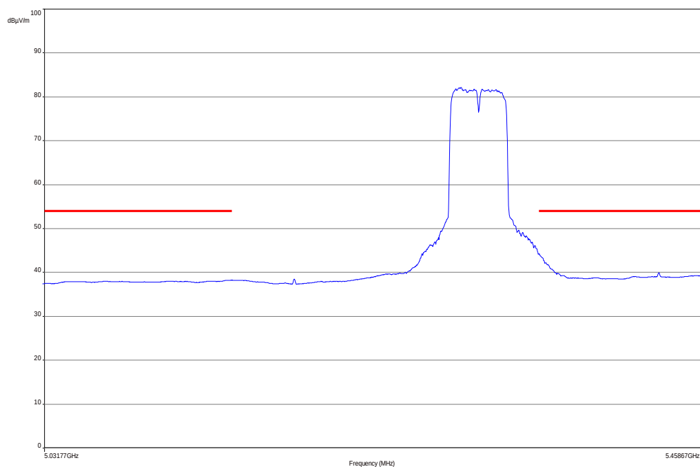
Plot 5: upper band edge, vertical & horizontal polarization (n HT 40 mode), channel 60
