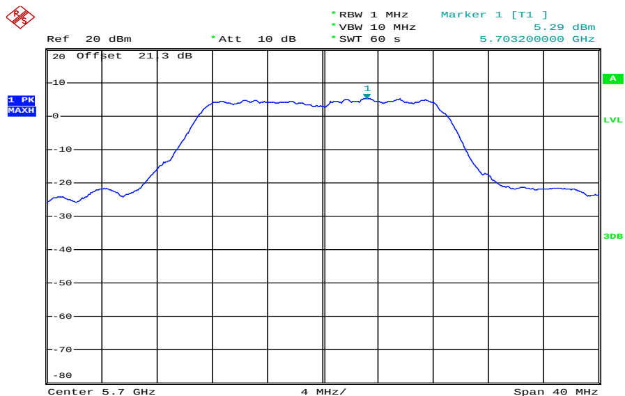
Plot 7: 5700 MHz
