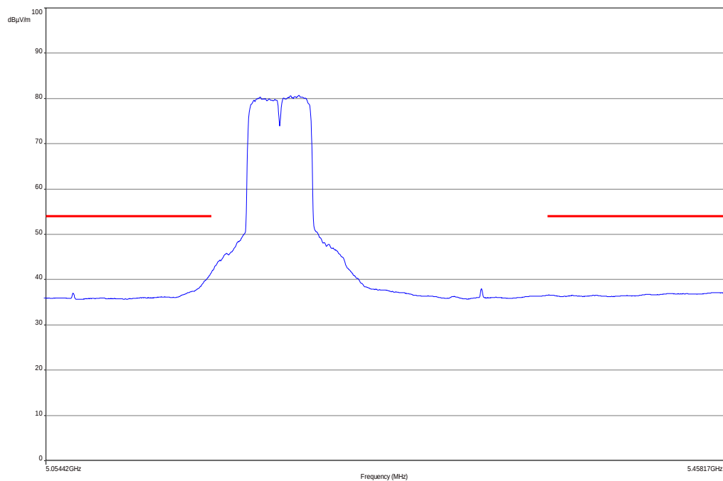
Plot 4: lower band edge, vertical & horizontal polarization (n HT 40 mode), channel 36
