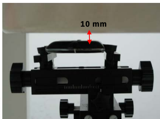
Fig.10 EUT Back to flat phantom
