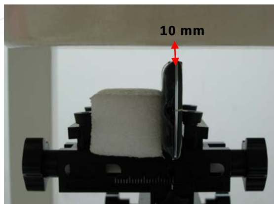
Fig.13 EUT Right to flat phantom
