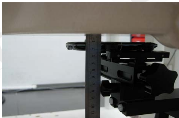
Fig.9 EUT Front to flat phantom
