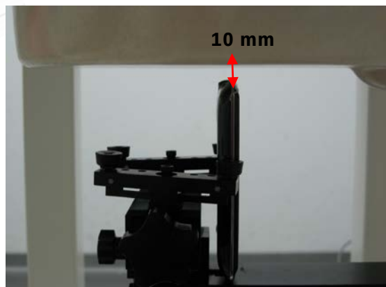
Fig.15 EUT Top to flat phantom
