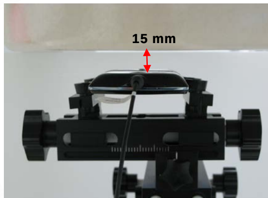
Fig.8 EUT Back side with Headset to flat phantom
