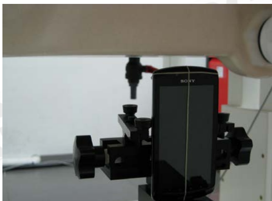
Fig.15 EUT Top to flat phantom
