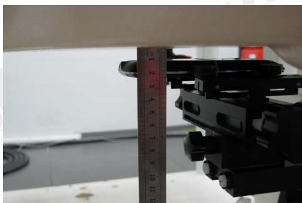
Fig.10 EUT Back to flat phantom
