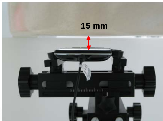
Fig.7 EUT Front side with Headset to flat phantom
