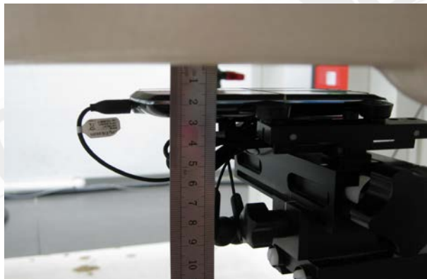
Fig.7 EUT Front side with Headset to flat phantom
