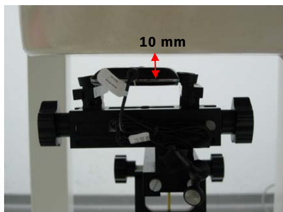
Fig.11 EUT Back side with Headset to flat phantom
