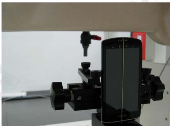
Fig.12 EUT Bottom to flat phantom
