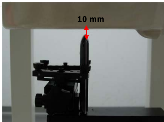
Fig.12 EUT Bottom to flat phantom
