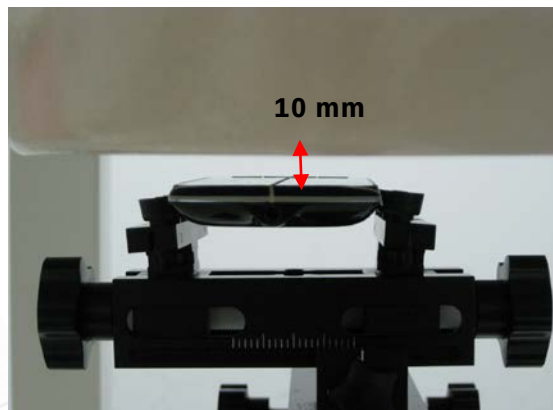
Fig.9 EUT Front to flat phantom
