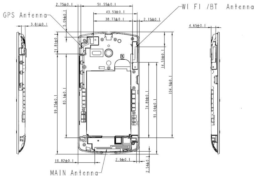
Fig.21 Antenna position of EUT
