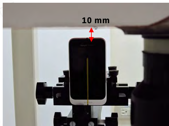
Fig.12 EUT Top to flat phantom
