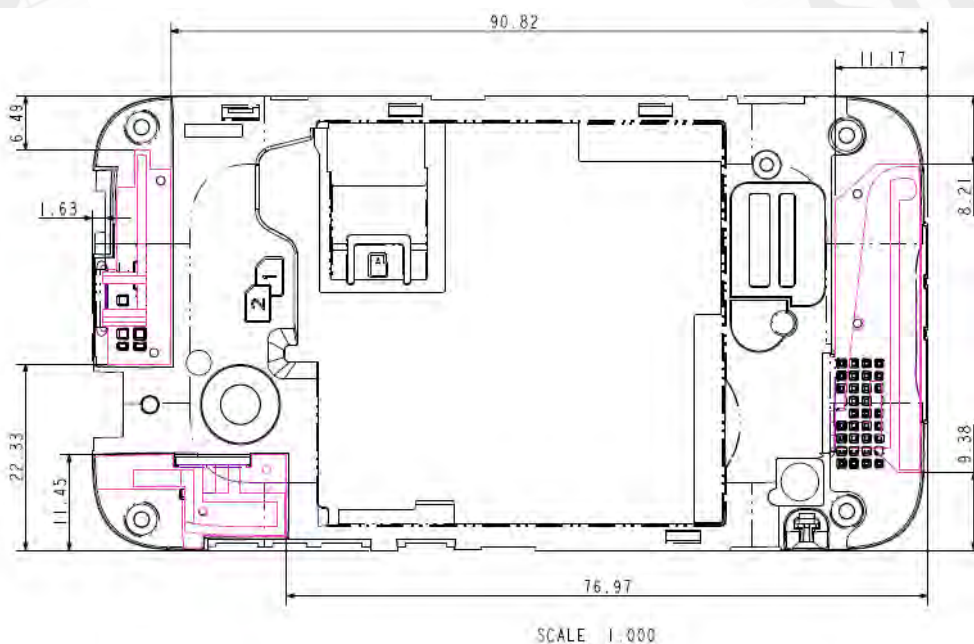
Fig.23 Antenna position of EUT
