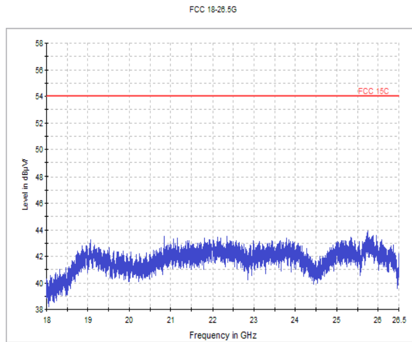
Fig.81. Radiated emission: \pi/4 DQPSK, 18 GHz - 26 GHz
