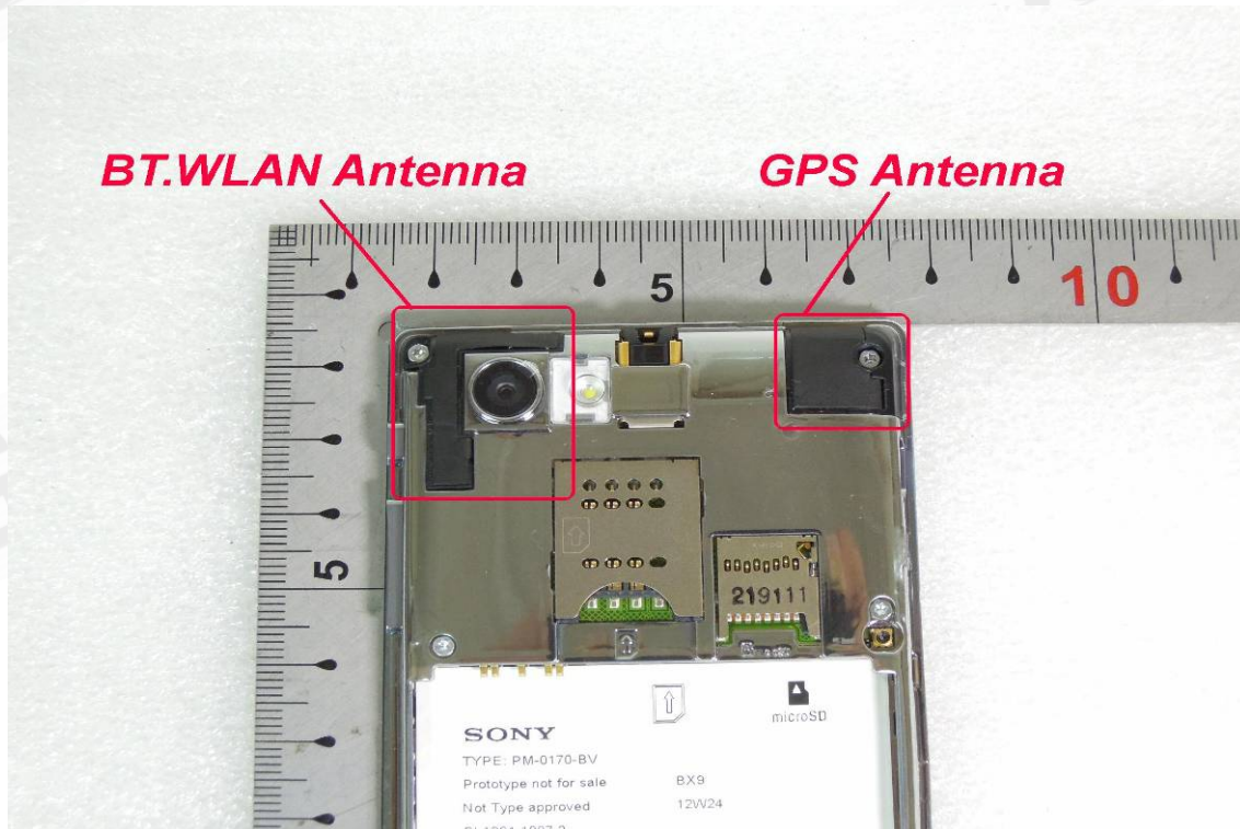
BT/WLAN/GPS Antenna
