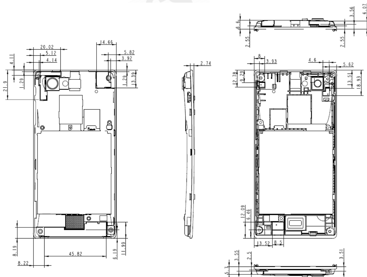
Fig.21 Antenna position of EUT
