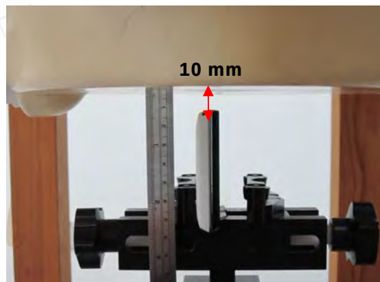
Fig.15 EUT left to flat phantom
