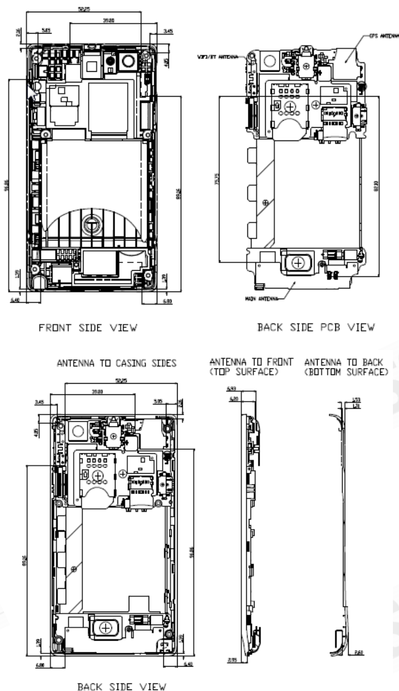
Fig.23 Antenna position of EUT
