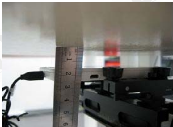
Fig.7 EUT front to flat phantom
