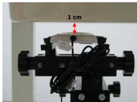
Fig.11 EUT back to flat phantom with headset
