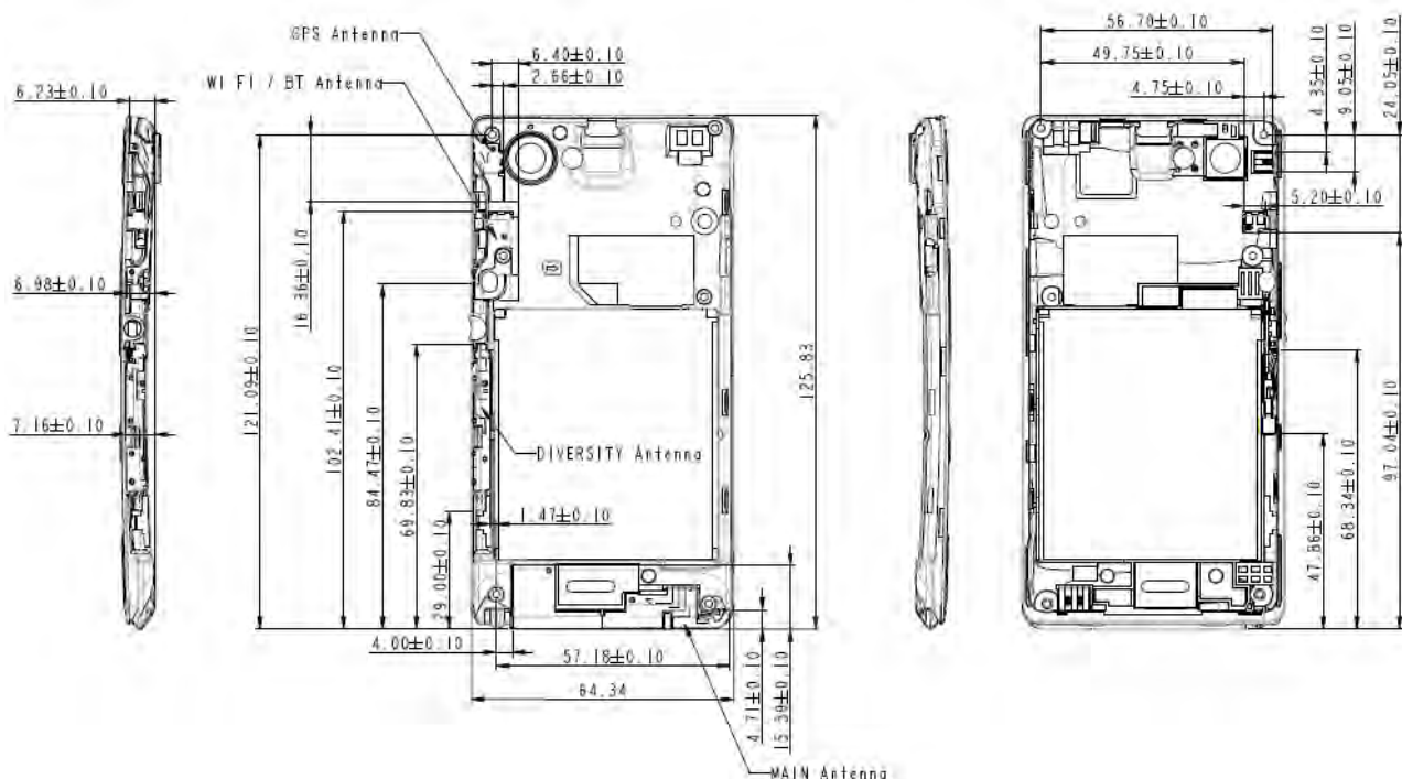
Fig.21 Antenna position of EUT
