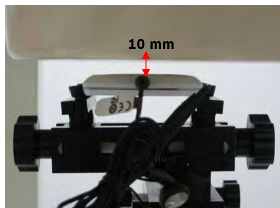
Fig.11 EUT back side with headset (MH410C) to flat phantom
