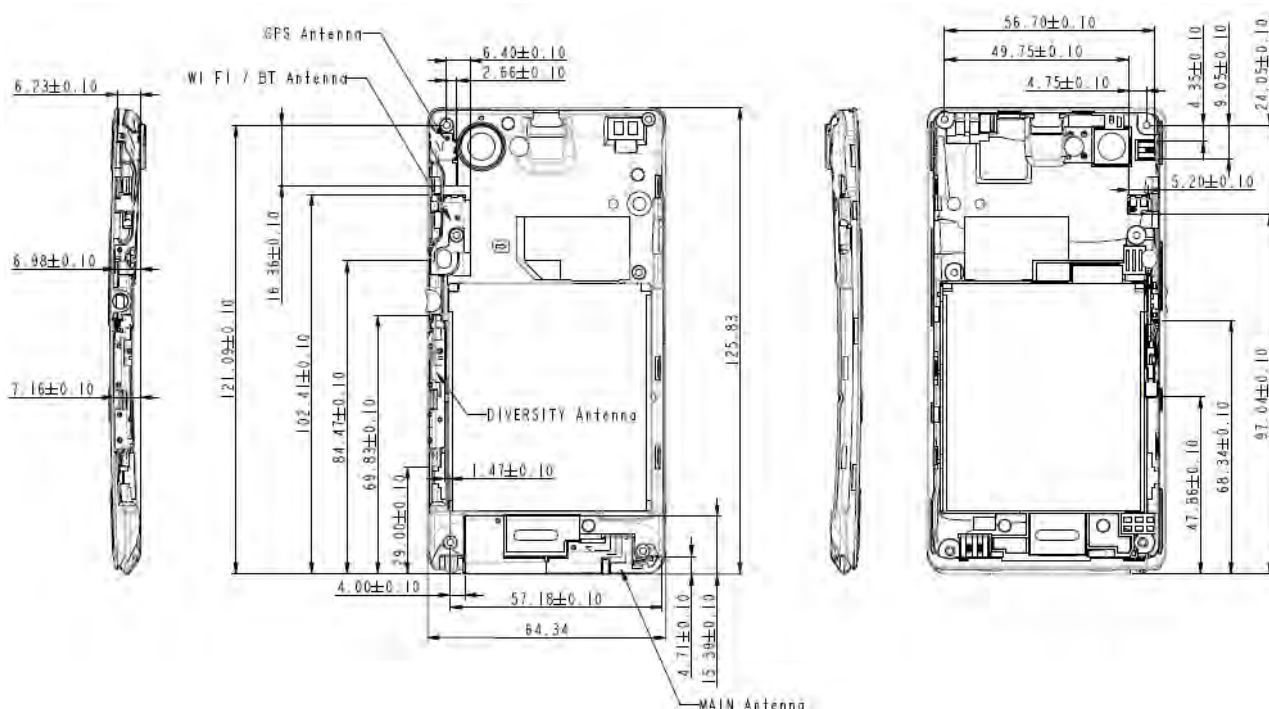
Fig.20 Antenna position of EUT
