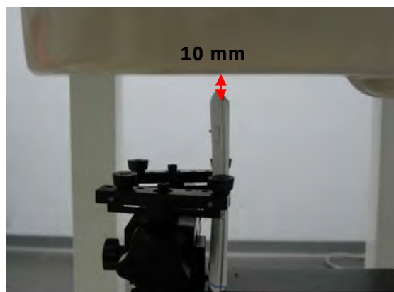
Fig.11 EUT bottom to flat phantom
