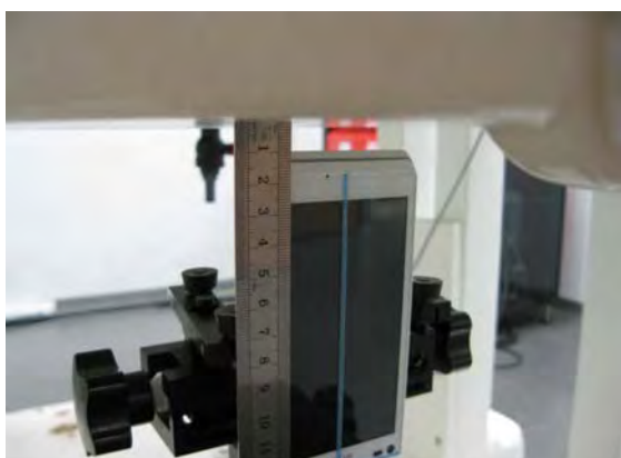
Fig.11 EUT bottom to flat phantom
