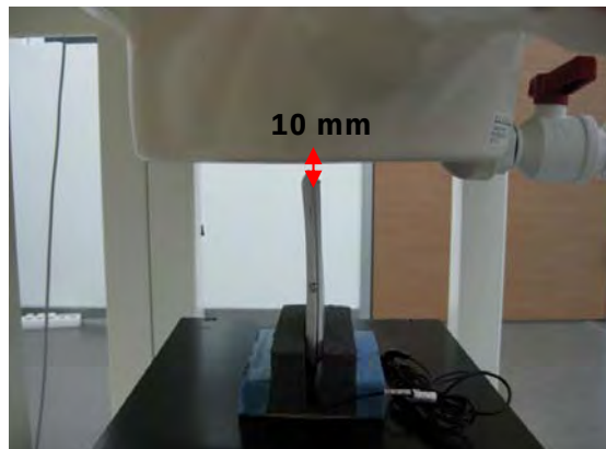
Fig.12 EUT bottom with headset (MH410C) to flat phantom
