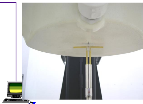
Fig 8.3.2 Setup Photo
