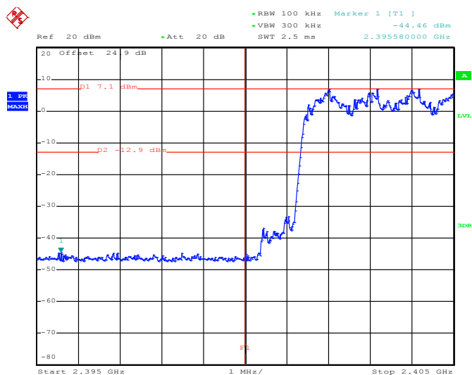
3Mbps Hopping Mode Low Band Edge Plot
