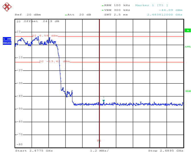
3Mbps Hopping Mode High Band Edge Plot
