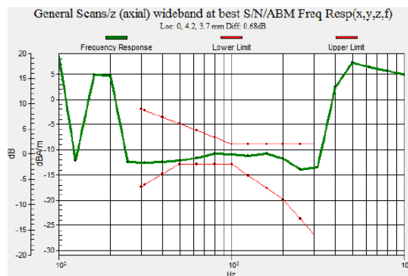
Fig 7.2 GSM1900 Ch661
