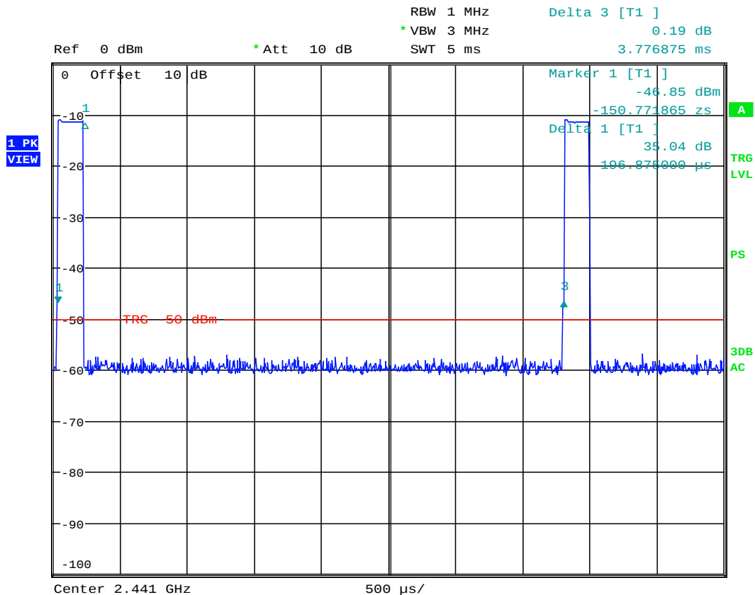
Plot 6-2. Pulse Width Measurement
