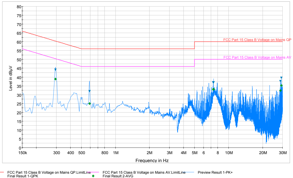
Plot 6-7. Line-Conducted Test Plot (N)
