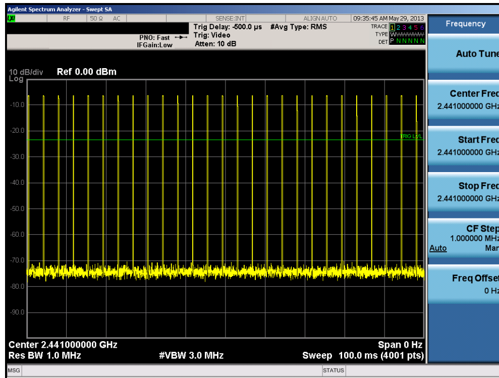
Plot 6-3. Worst Case 100ms Operation
