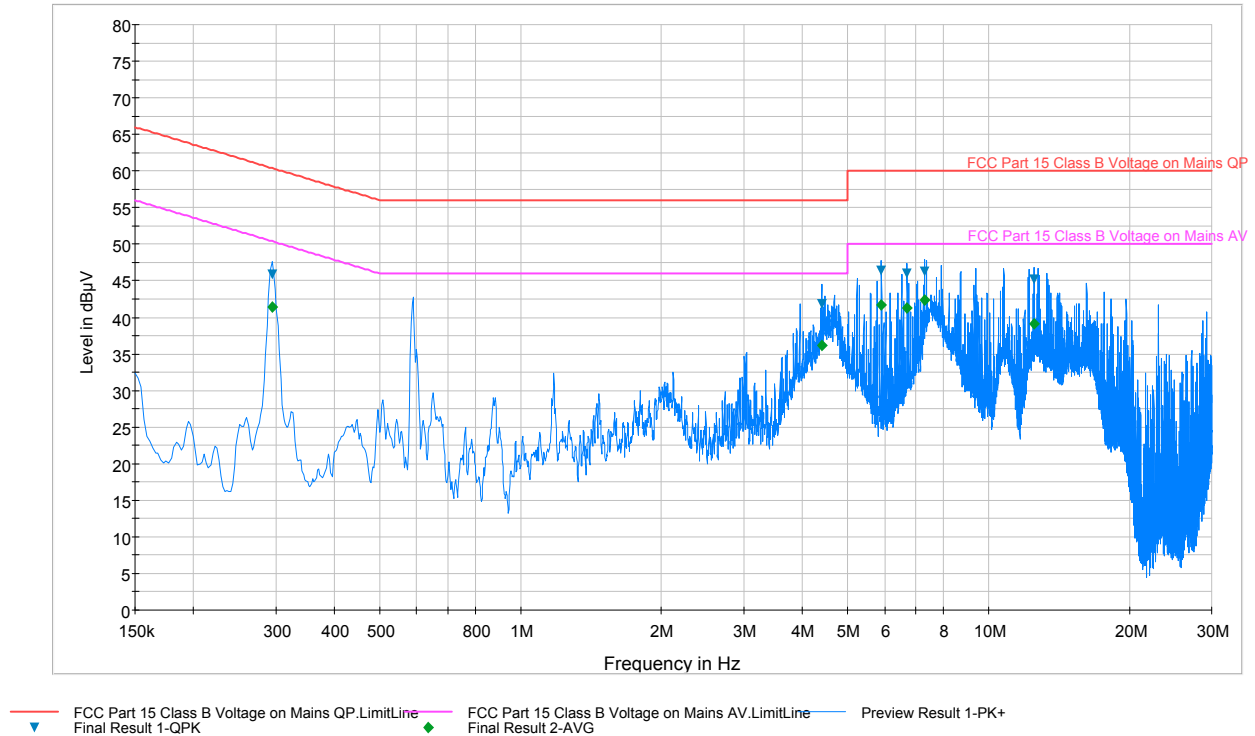
Plot 6-6. Line-Conducted Test Plot (L1)
