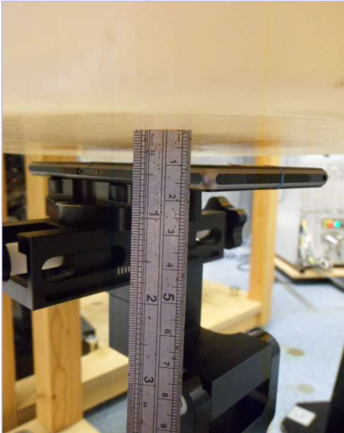
PHT/10014935/006: Front of EUT Facing Phantom at 10mm
