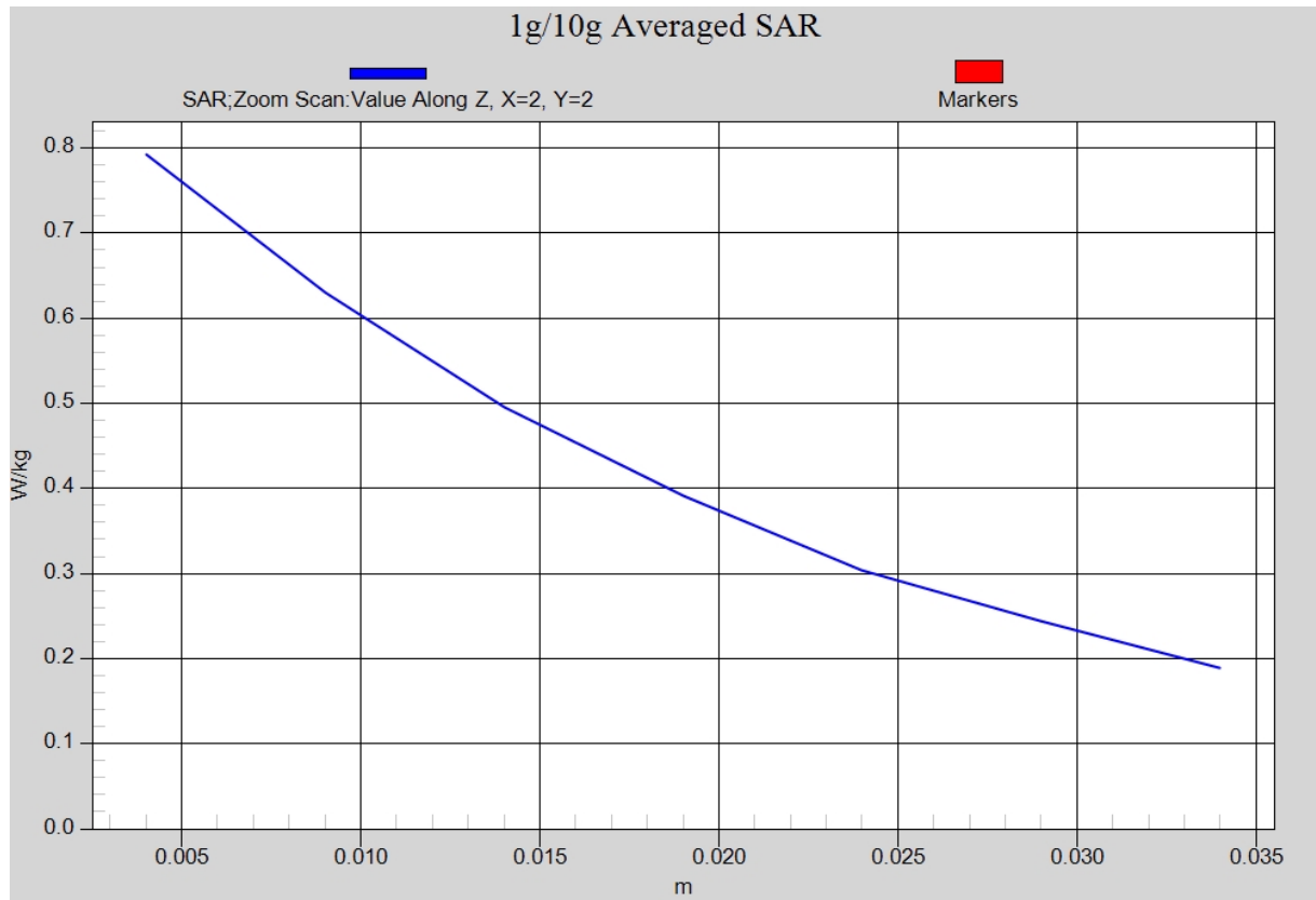
Fig. 8-1 Z-Scan at power reference point (WCDMA850 CH4233)
