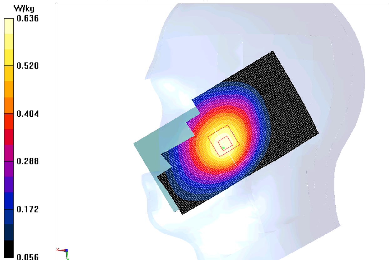
Fig.1 850MHz CH128
