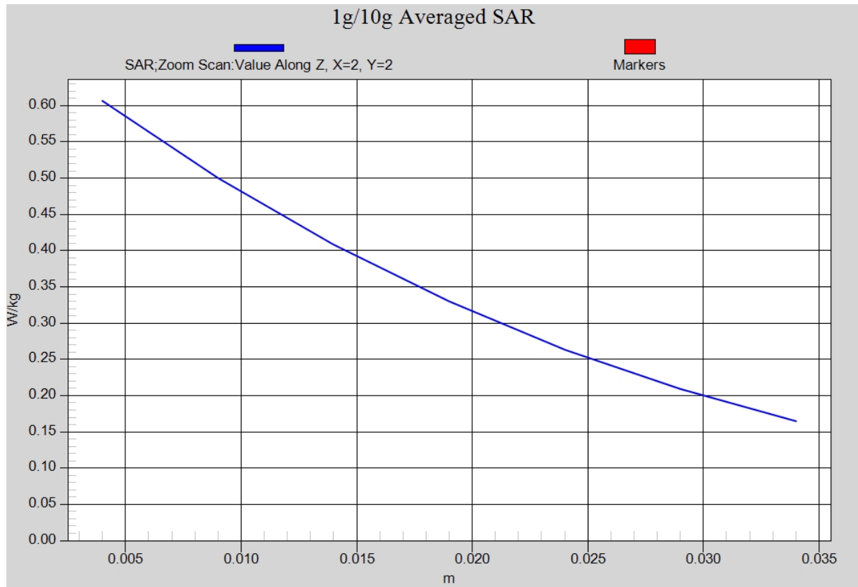
Fig. 7-1 Z-Scan at power reference point (WCDMA 850 CH4182)
