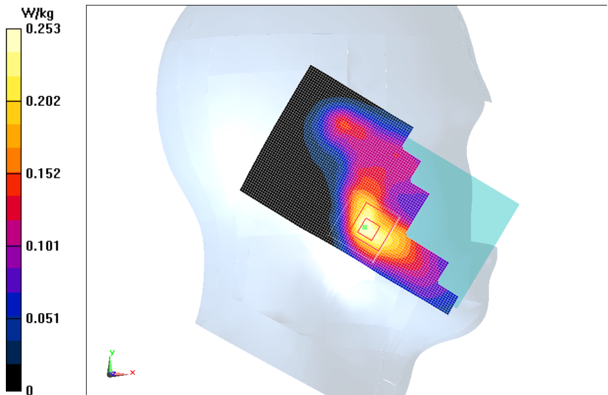
Fig.4 1900 MHz CH512
