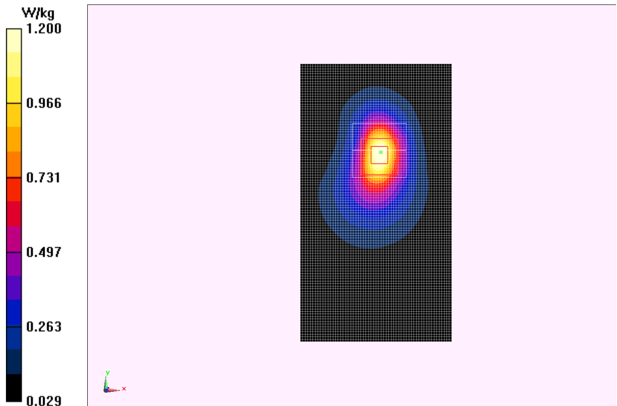
Fig.11 1700 MHz CH1513
