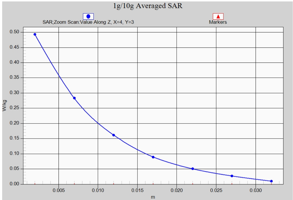
Fig. 23-1 Z-Scan at power reference point (2450 MHz CH1)
