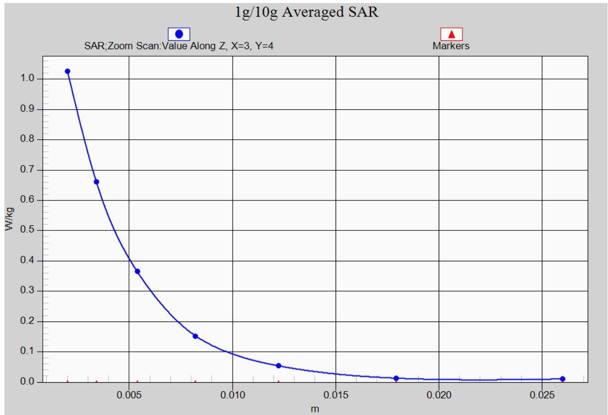
Fig. 29-1 Z-Scan at power reference point (5GHz CH62)
