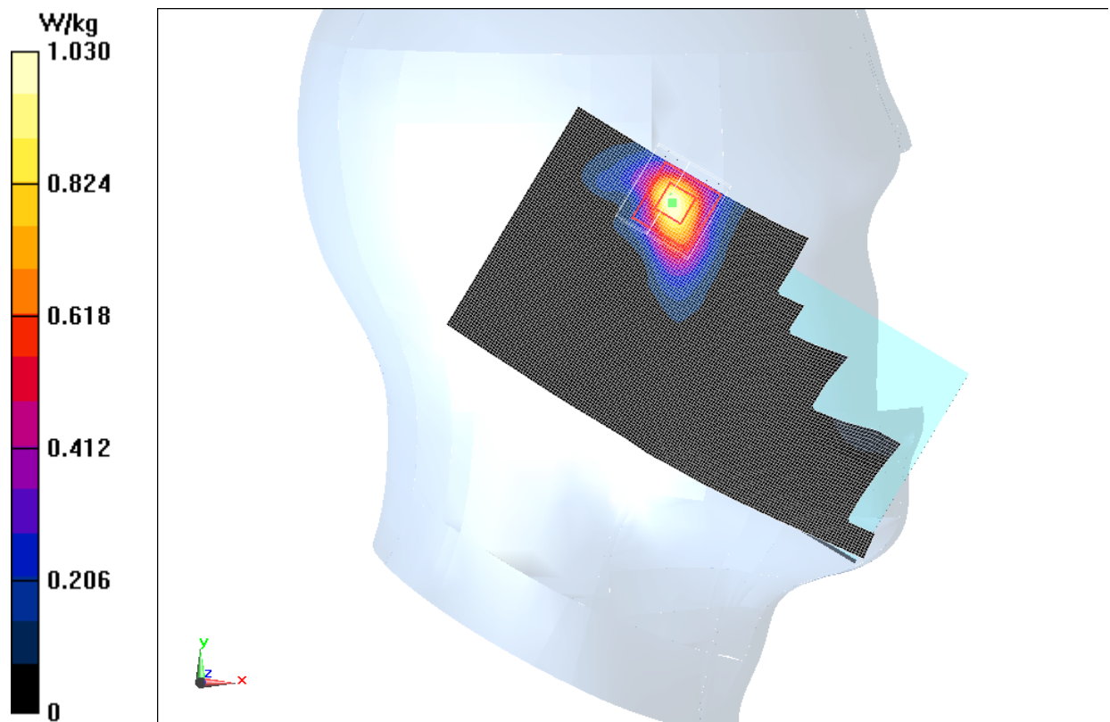
Fig.29 5GHz CH62
