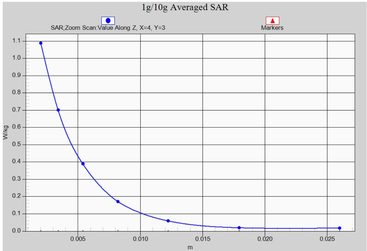
Fig. 31-1 Z-Scan at power reference point (5GHz CH42)
