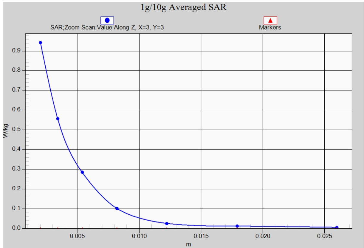
Fig. 30-1 Z-Scan at power reference point (5GHz CH62)
