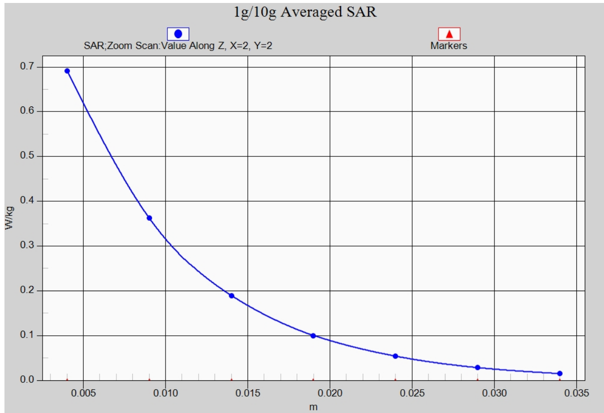
Fig. 22-1 Z-Scan at power reference point (2450 MHz CH6)
