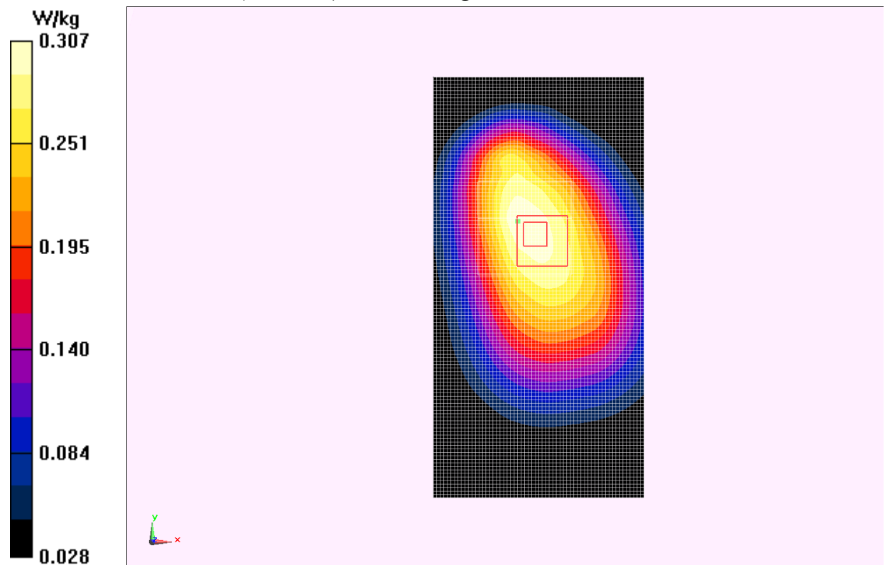
Fig.21 LTE Band17 CH23790
