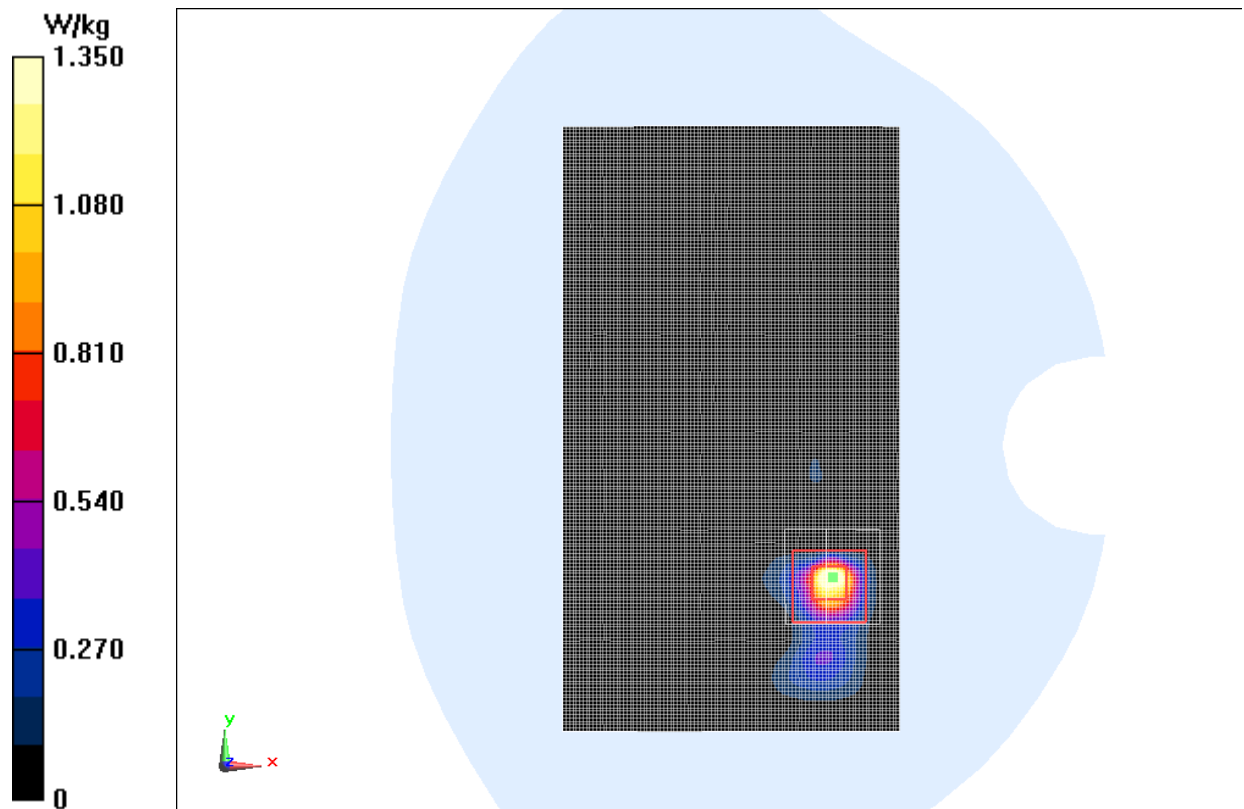
Fig.26-2 5GHz CH149
