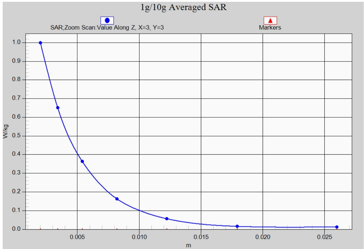
Fig. 25-1 Z-Scan at power reference point (5GHz CH60)
