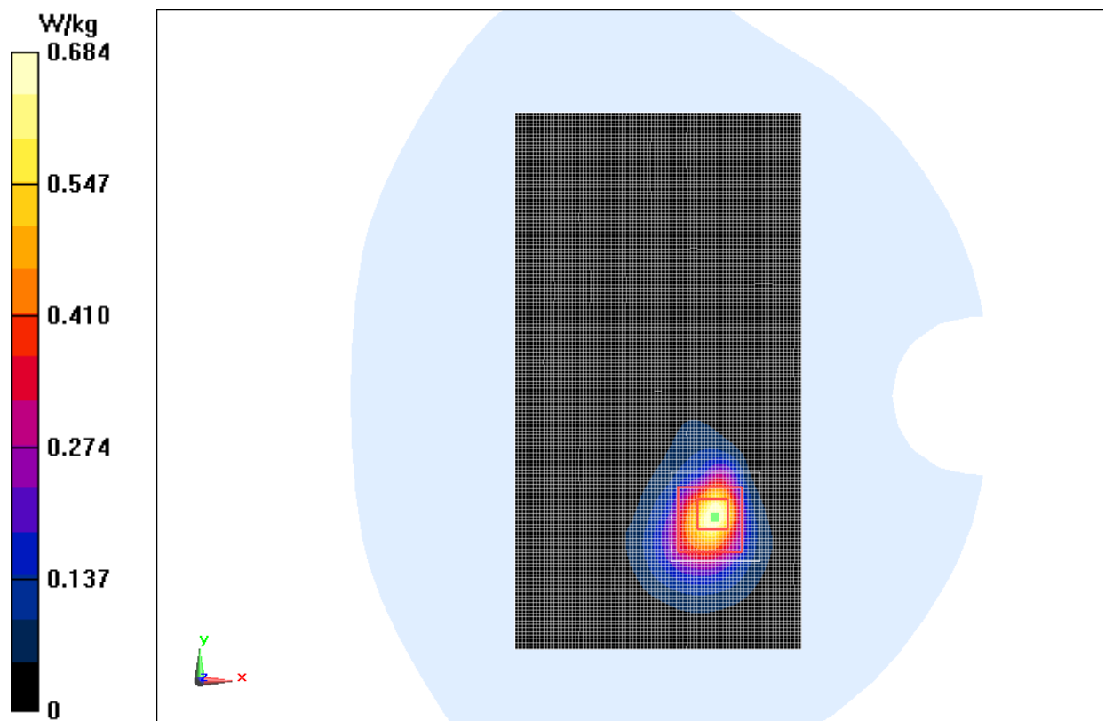
Fig.24 2450 MHz CH6
