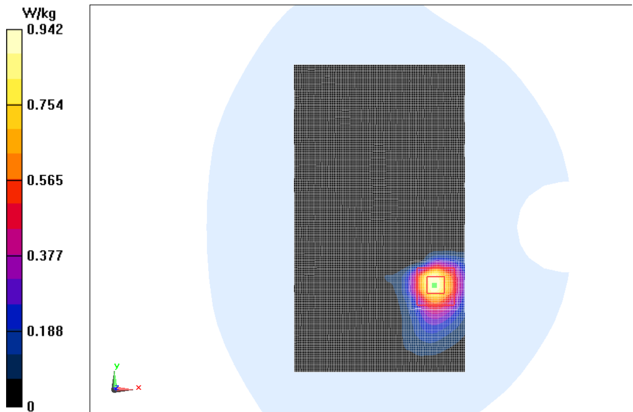
Fig.30 5GHz CH62
