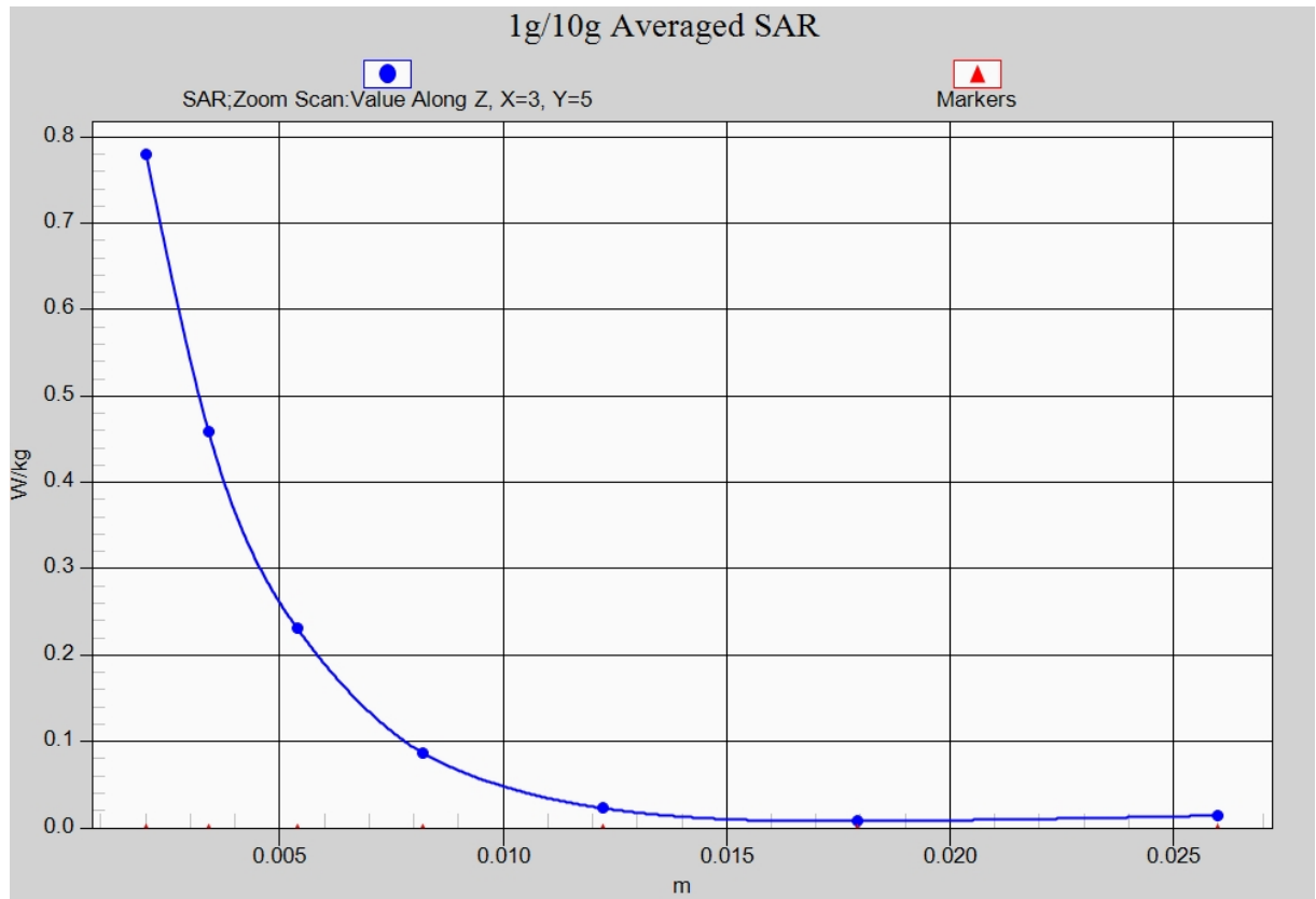
Fig. 28-1 Z-Scan at power reference point (5GHz CH60)
