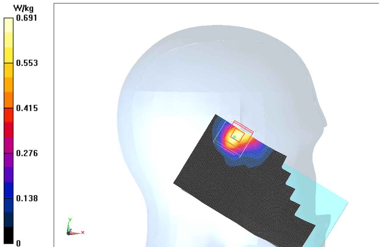
Fig.22 2450 MHz CH6
