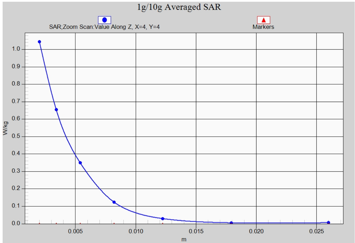
Fig. 26-1 Z-Scan at power reference point (5GHz CH44)
