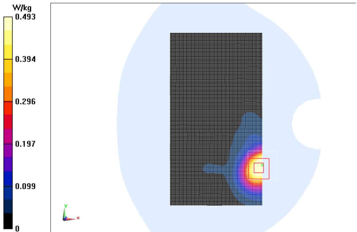
Fig.23 2450 MHz CH1
