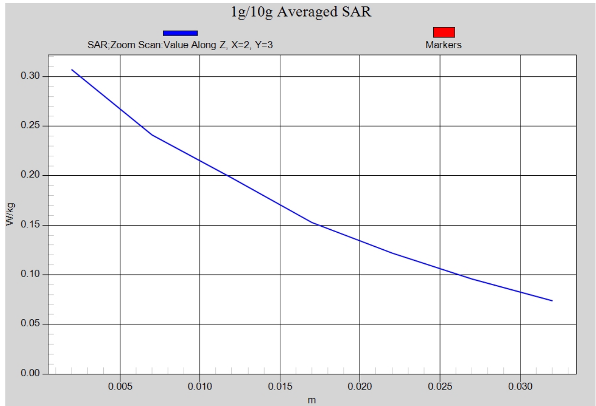
Fig. 21-1 Z-Scan at power reference point (LTE Band17 CH23790)
