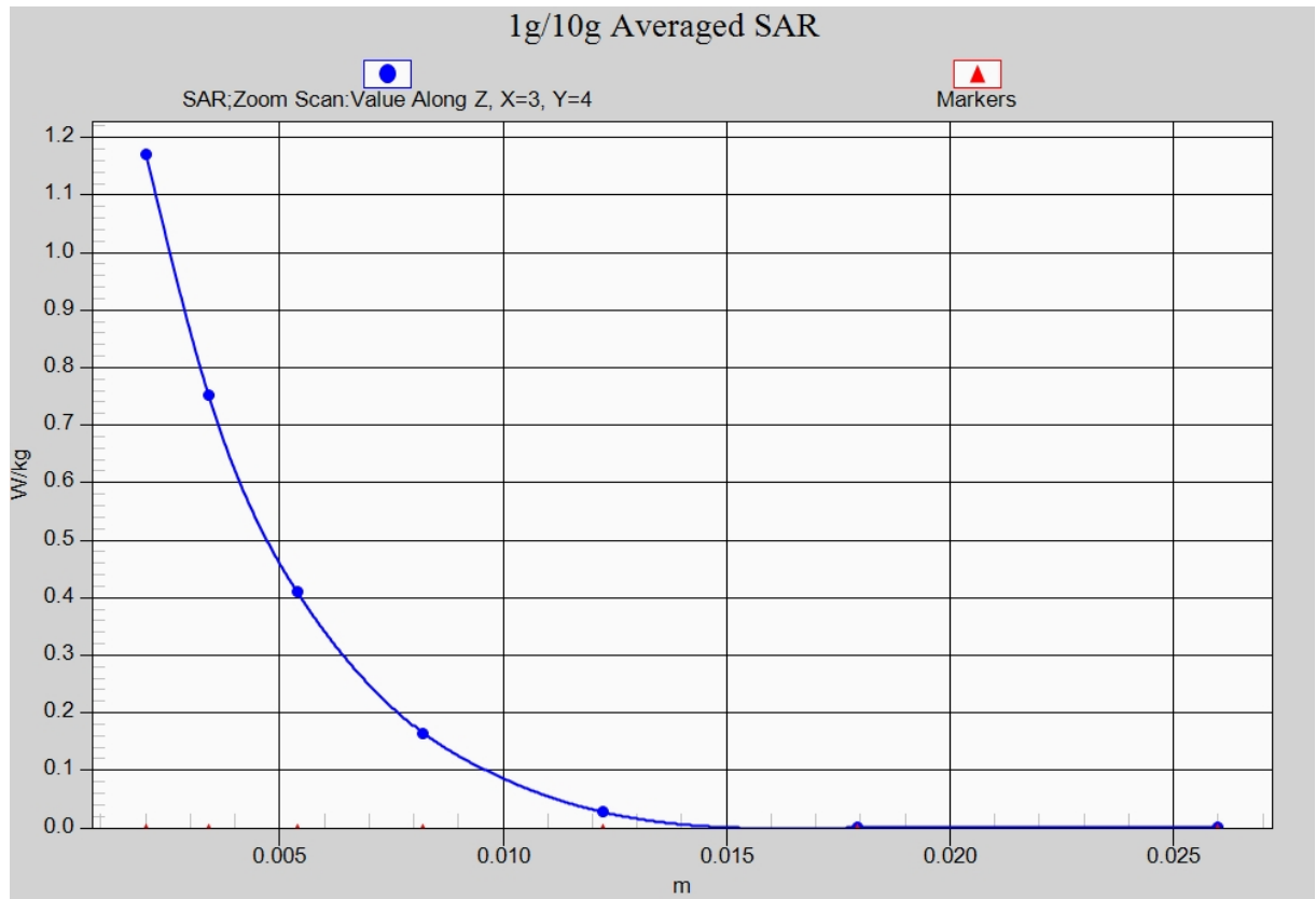
Fig. 27-1 Z-Scan at power reference point (5GHz CH60)
