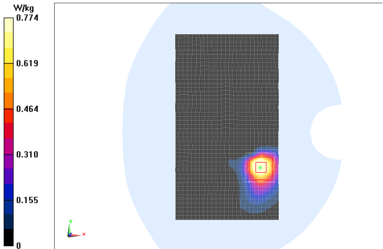
Fig.28 5GHz CH60
