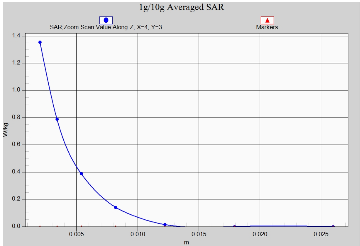
Fig. 26-3 Z-Scan at power reference point (5GHz CH149)
