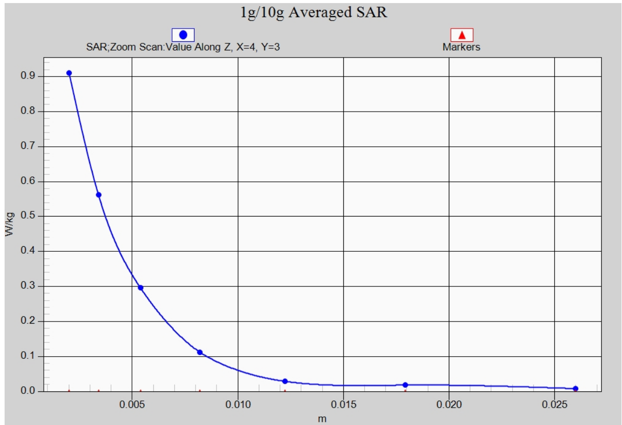
Fig. 32-1 Z-Scan at power reference point (5GHz CH42)
