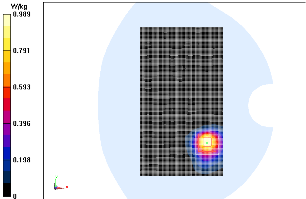
Fig.26 5GHz CH44
