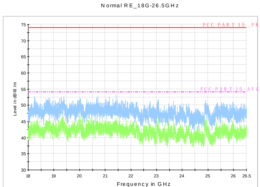
Fig. 115 Radiated emission: 18 GHz – 26.5 GHz
