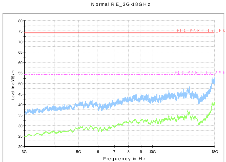
Fig. 90 Radiated Spurious Emission (802.11b, Ch1, 3 GHz-18 GHz)
