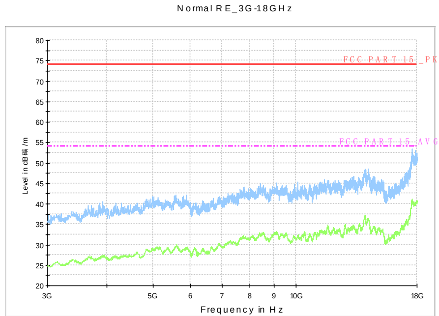
Fig. 96 Radiated Spurious Emission (802.11b, Ch11, 3 GHz-18 GHz)
