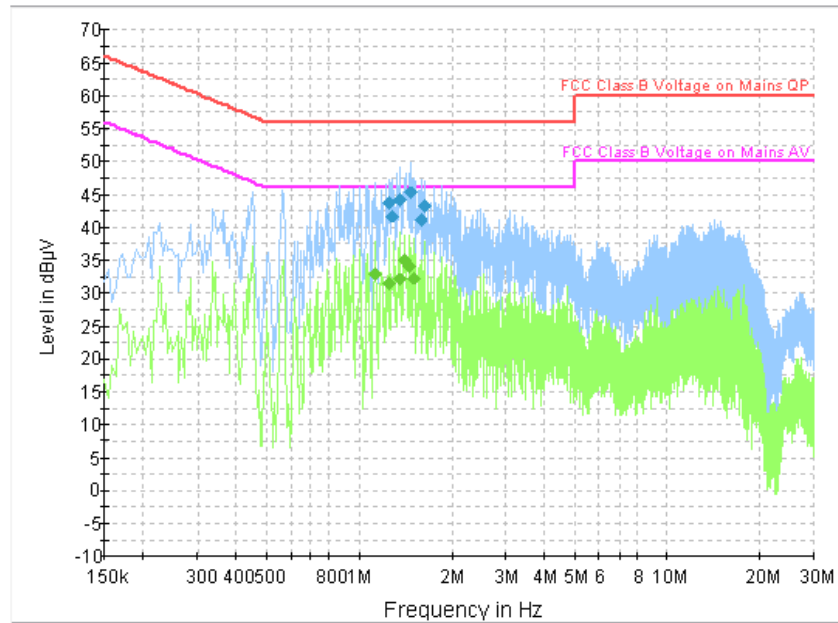
Fig. 117 AC Powerline Conducted Emission-Idle
