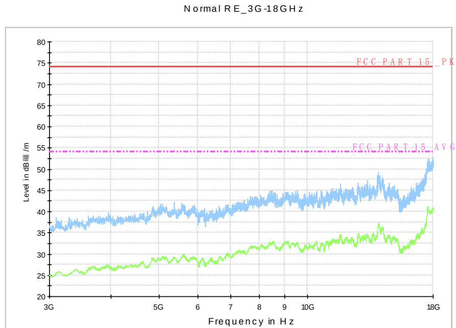
Fig. 108 Radiated Spurious Emission (802.11n-HT20, Ch1, 3 GHz-18 GHz)
