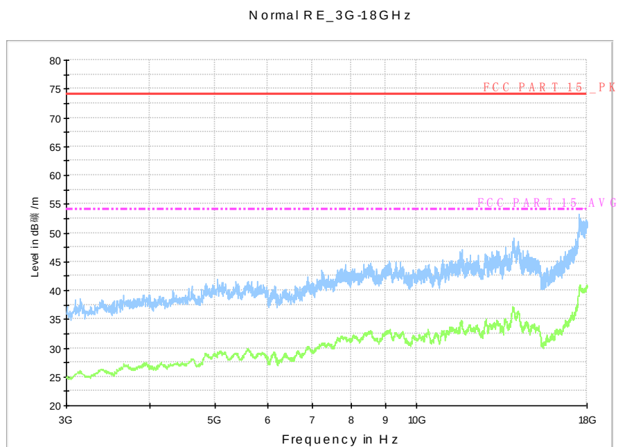
Fig. 102 Radiated Spurious Emission (802.11g, Ch6, 3 GHz-18 GHz)
