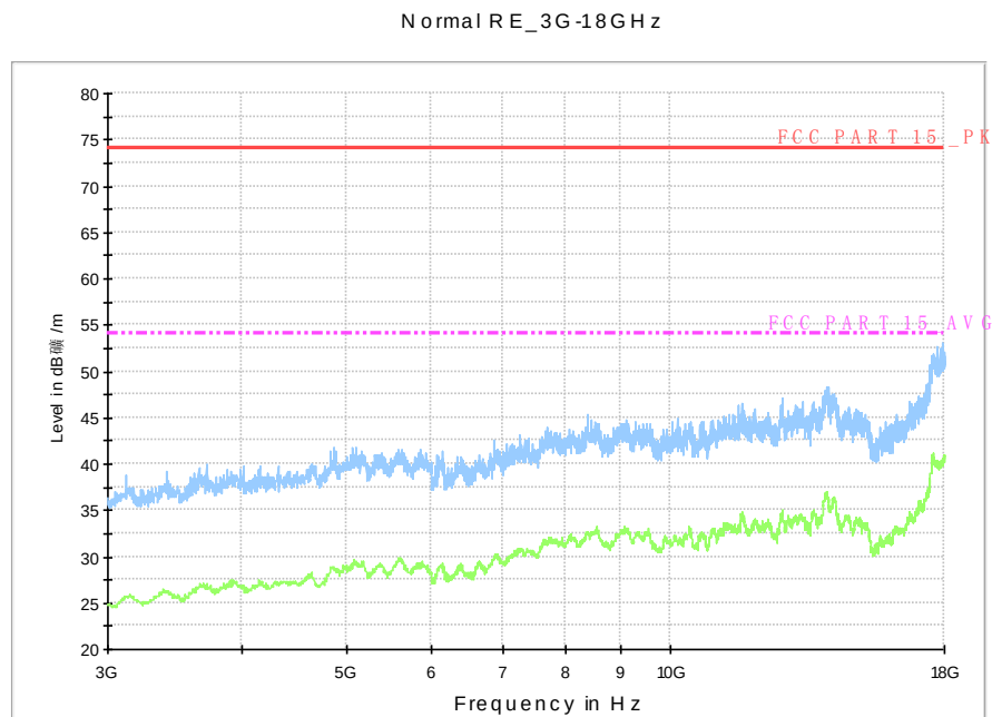
Fig. 105 Radiated Spurious Emission (802.11g, Ch11, 3 GHz-18 GHz)
