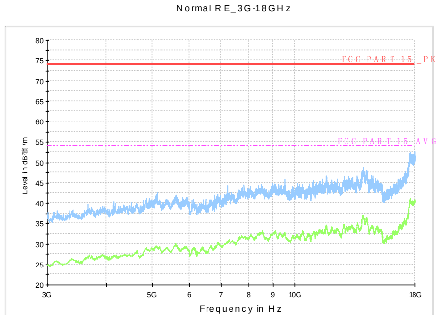
Fig. 114 Radiated Spurious Emission (802.11n-HT20, Ch11, 3 GHz-18 GHz)
