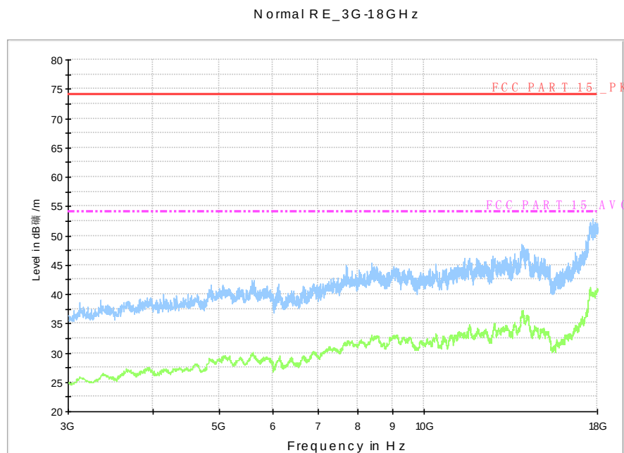
Fig. 111 Radiated Spurious Emission (802.11n-HT20, Ch6, 3 GHz-18 GHz)
