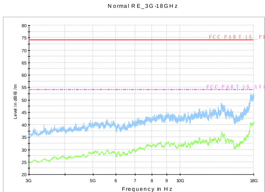
Fig. 99 Radiated Spurious Emission (802.11g, Ch1, 3 GHz-18 GHz)
