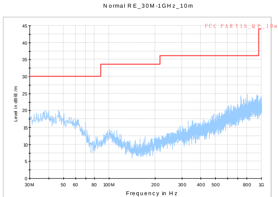
Fig. 109 Radiated Spurious Emission (802.11n-HT20, Ch6, 30 MHz-1 GHz)
