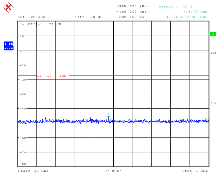
Fig. 40 Conducted Spurious Emission (802.11g, Ch1, Center Frequency)
