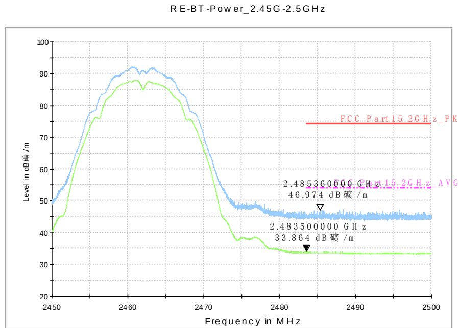
Fig. 94 Radiated Spurious Emission (Power): 802.11b, ch11, 2.45 GHz - 2.5GHz
