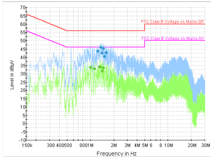
Fig. 116 AC Powerline Conducted Emission-802.11b
