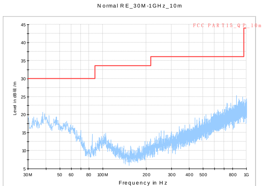
Fig. 100 Radiated Spurious Emission (802.11g, Ch6, 30 MHz-1 GHz)
