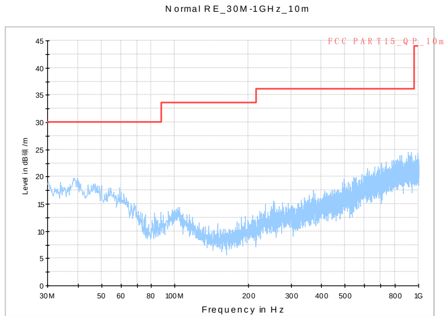
Fig. 91 Radiated Spurious Emission (802.11b, Ch6, 30 MHz-1 GHz)
