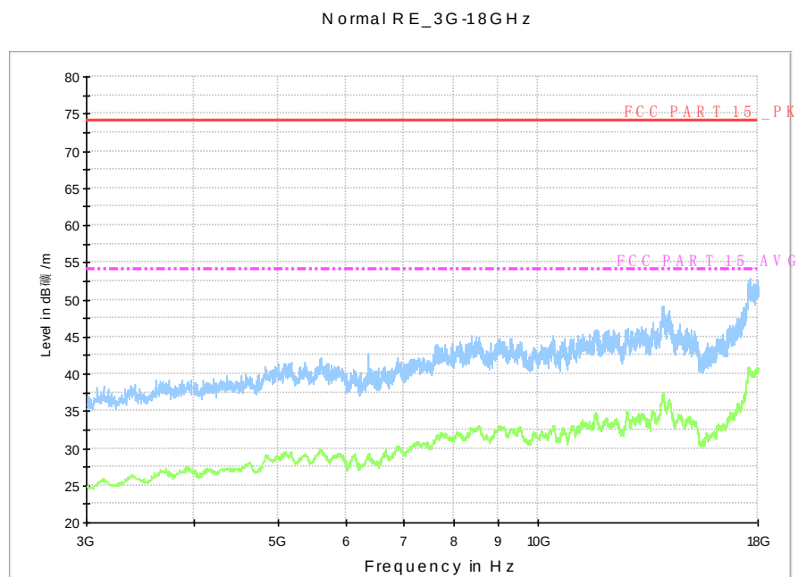
Fig. 93 Radiated Spurious Emission (802.11b, Ch6, 3 GHz-18 GHz)
