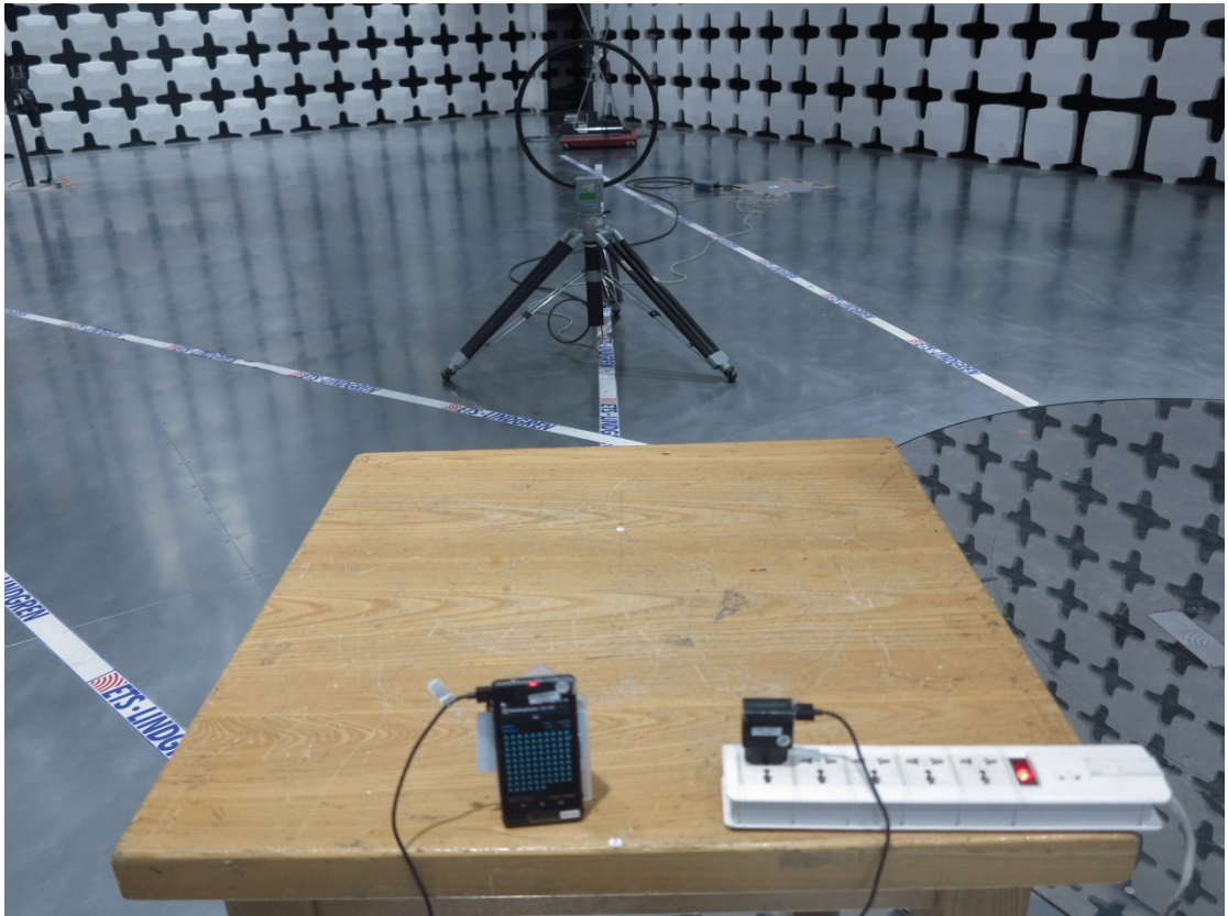
Picture C-1: Field Strength Measurements (Below 30MHz)
