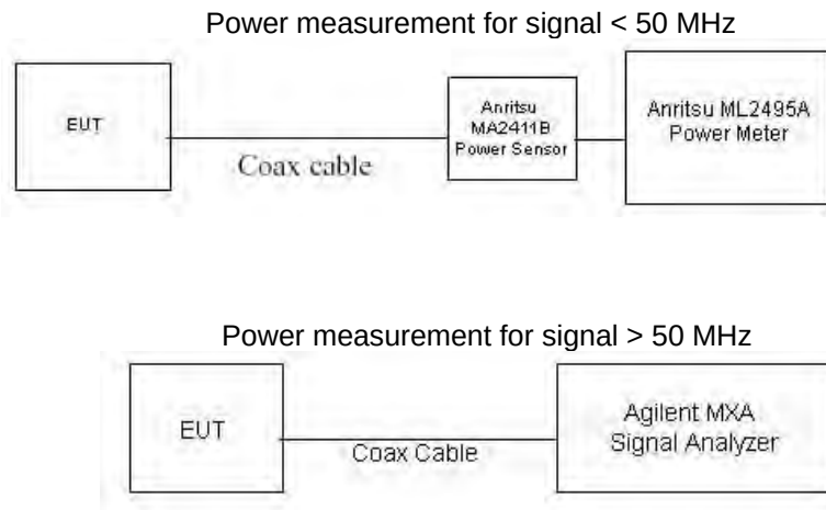
Figure 9-3 Power Measurement Setup
