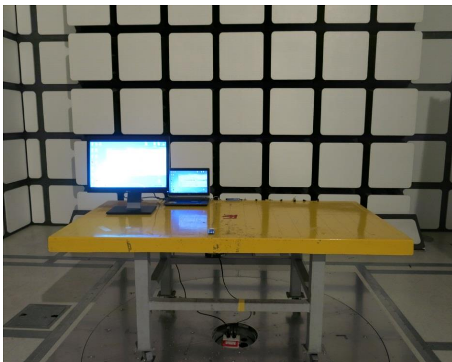
Rear View
