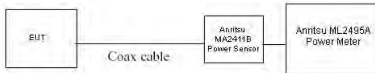
Figure 8-3 Power Measurement Setup for Signal < 50 MHz
