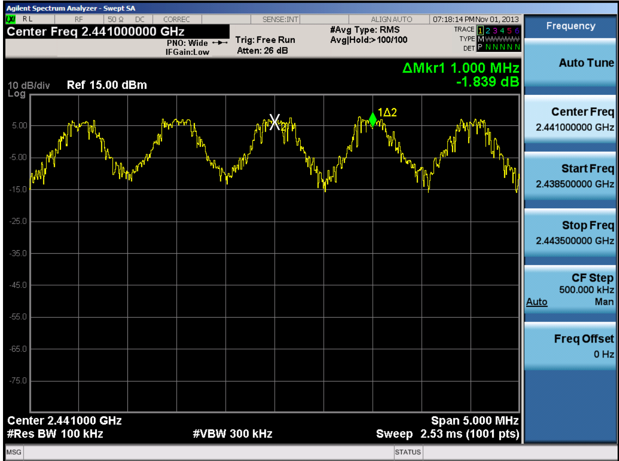
Plot 6-32. Channel Spacing Plot (Bluetooth)
