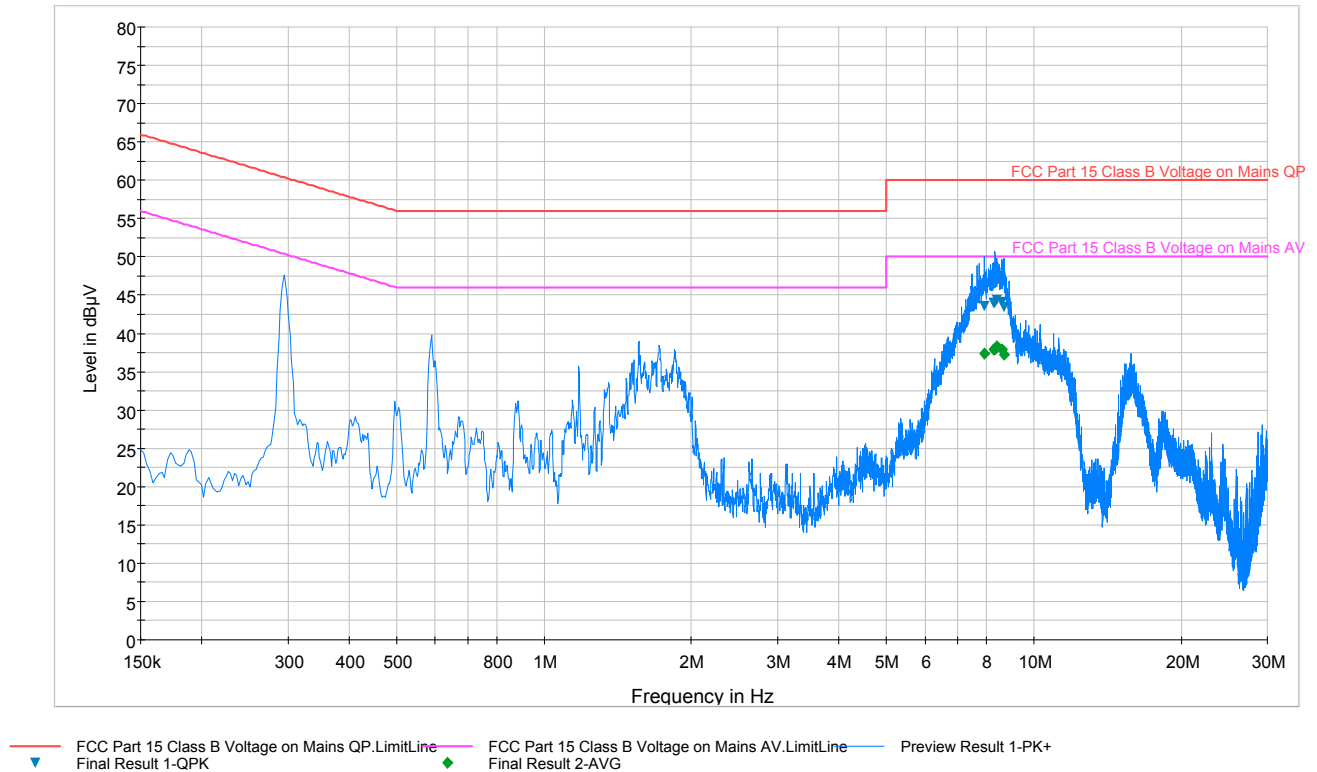
Plot 6-7. Line-Conducted Test Plot (N)
