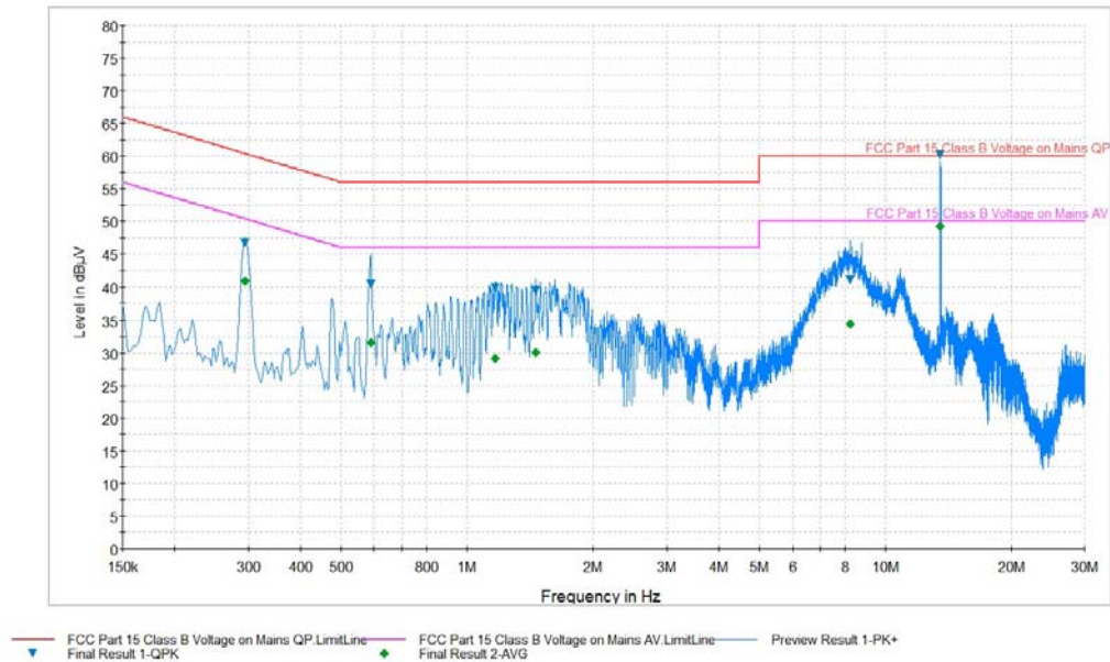
Plot 8-1. Line-Conducted Test Plot (L1)
