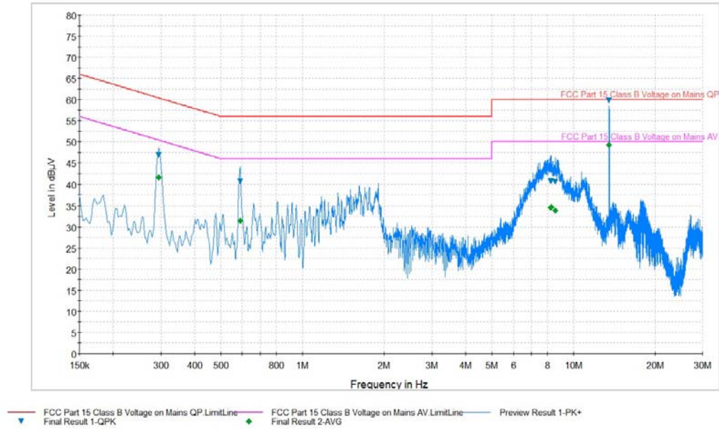
Plot 8-2. Line-Conducted Test Plot (N)
