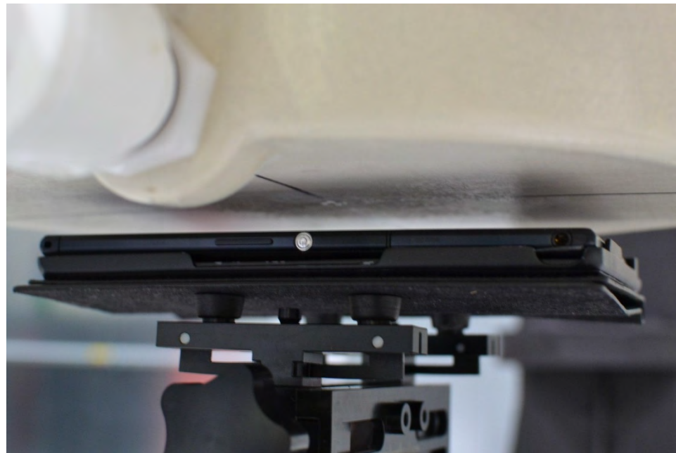
SAR Test Setup Photo 14 – Front Side at 1.5 cm with L-Battery Cover
