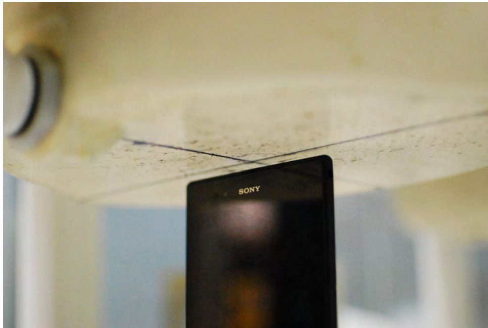
SAR Test Setup Photo 22 – Top Edge at 0.3 cm
