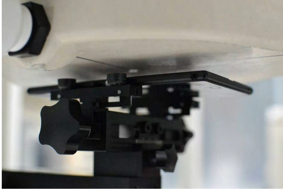
SAR Test Setup Photo 13 – Front Side at 1.5 cm
