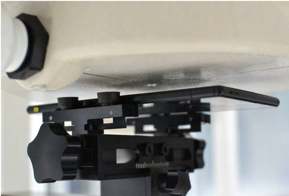
SAR Test Setup Photo 10 – Back Side at 1.5 cm
