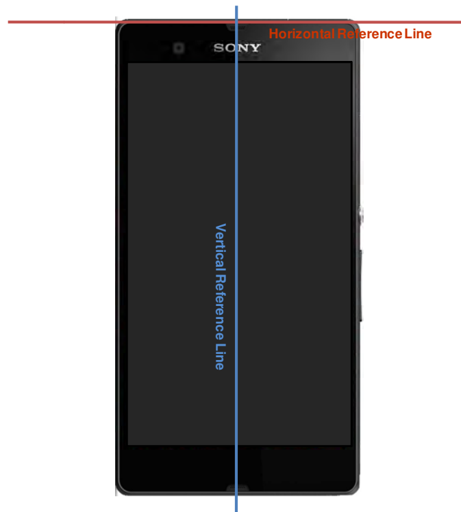
SAR Test Setup Photo 24 – DUT Reference Lines
