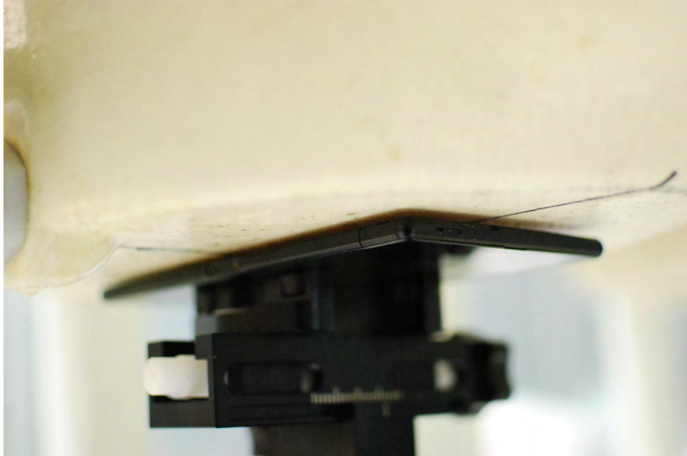
SAR Test Setup Photo 19 – Back Side at 0.3 cm
