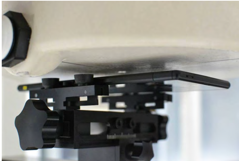
SAR Test Setup Photo 8 – Back Side at 1.0 cm
