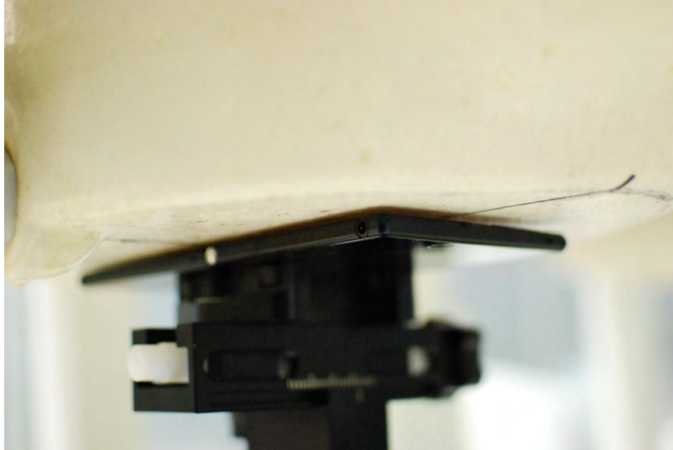
SAR Test Setup Photo 21 – Front Side at 0.3 cm
