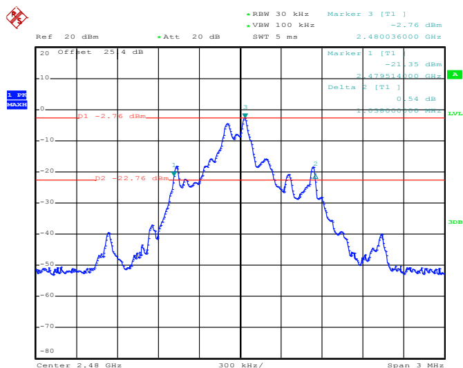
20 dB Bandwidth Plot on 2480MHz
