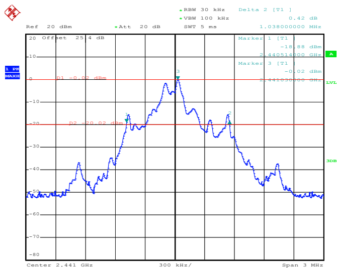
20 dB Bandwidth Plot on 2441MHz
