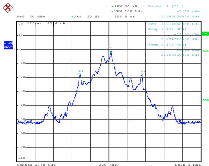
99% Bandwidth Plot on 2480MHz
