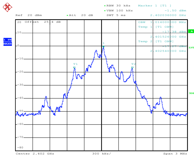
99% Bandwidth Plot on 2402MHz
