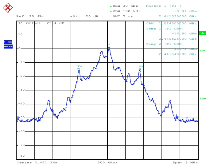
99% Bandwidth Plot on 2441MHz
