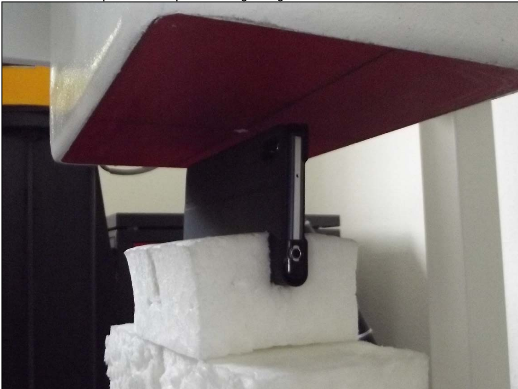
Photo 26: Test position hotspot mode right edge side 10mm distance with WPC cover
