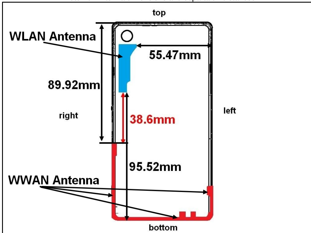
Photo 16: Antenna dimensions and separation distances
