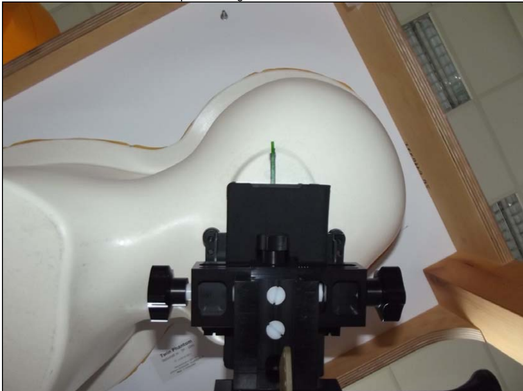
Photo 22: Test position right hand touched with WPC cover
