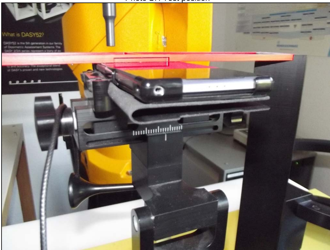
Photo 17: Test position
