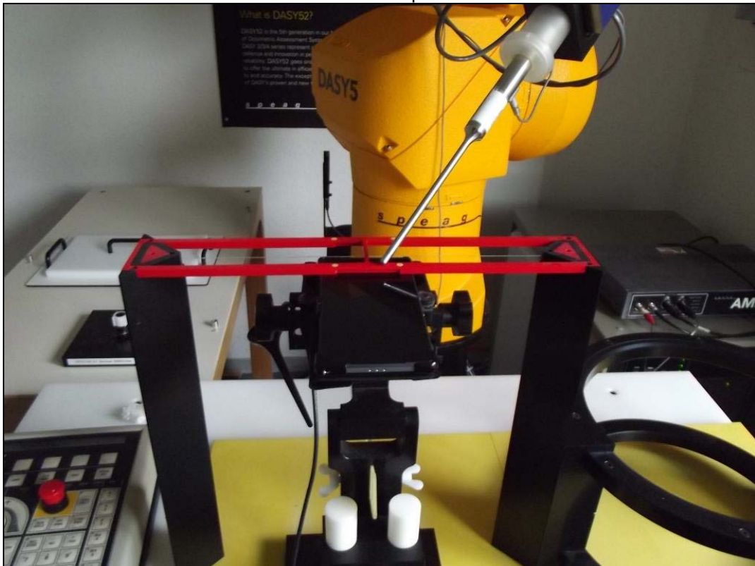
Photo 17: Test position
