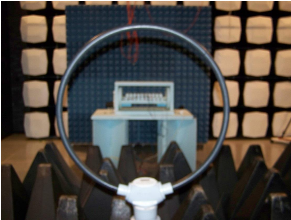
Photograph 1: magnetic field measurements
