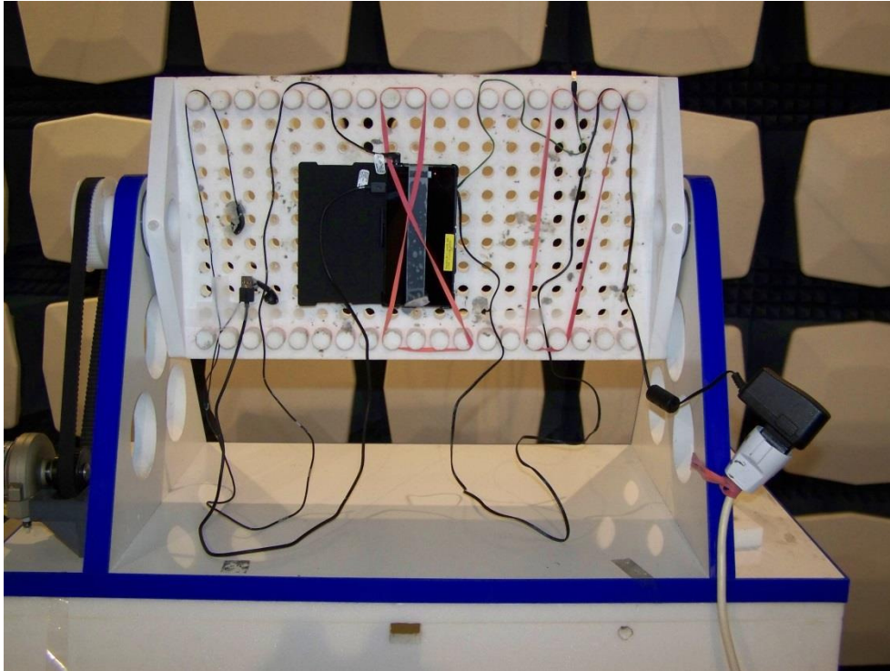
Photograph 5: measurements above 1GHz, detailed view
