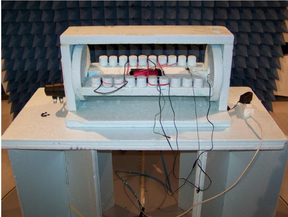
Photograph 3: measurements below 1GHz, detailed view
