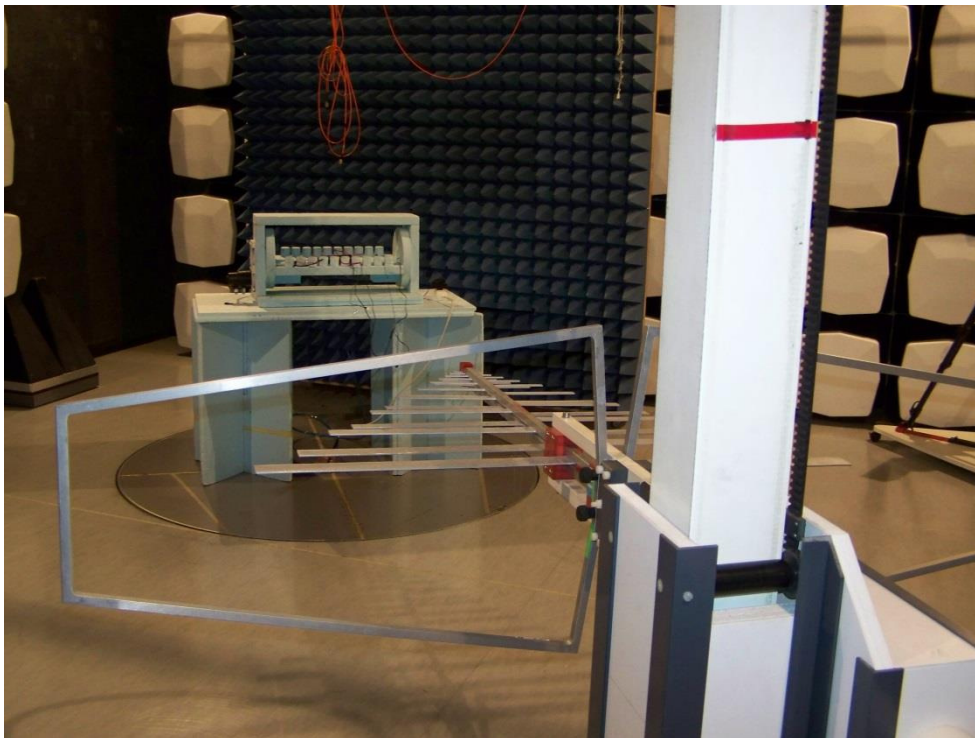
Photograph 2: measurements below 1GHz, overall view
