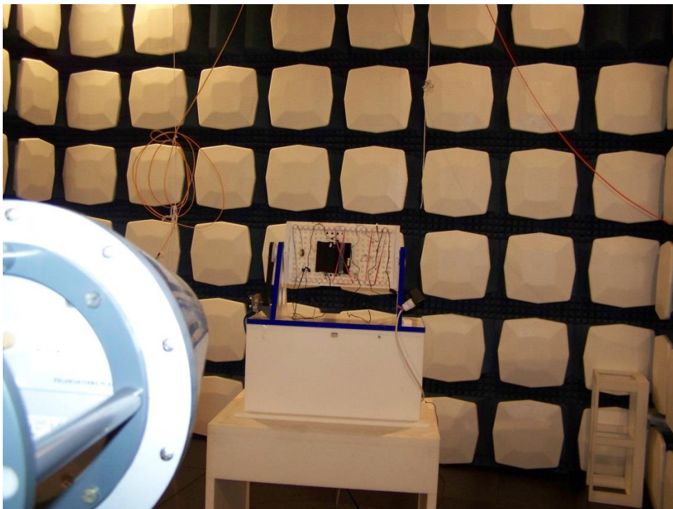
Photograph 4: measurements above 1GHz, overall view
