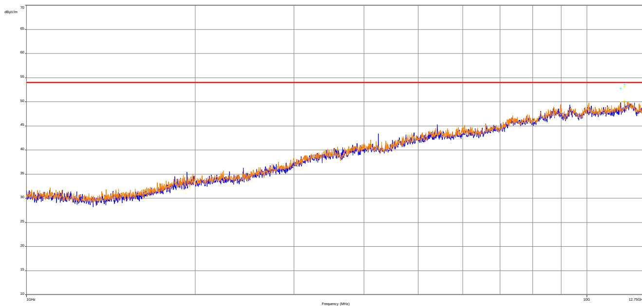
Plot 3: Receiver mode 1 GHz to 12.75 GHz
