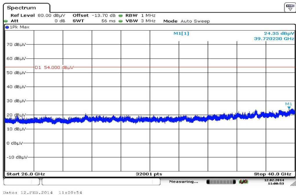
Plot 6: Receiver mode 26 GHz to 40 GHz
