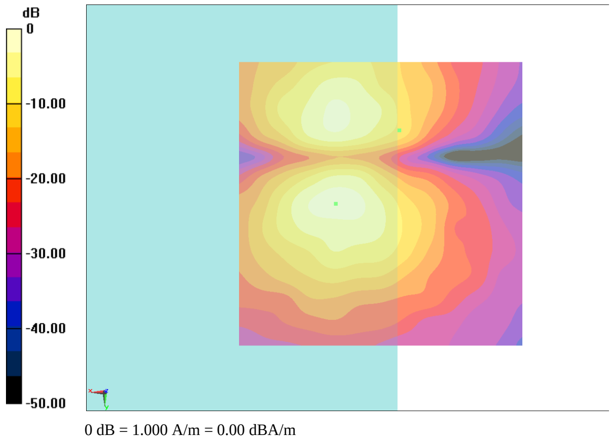
Fig B.1 T-Coil CDMA 835_Channel 777
