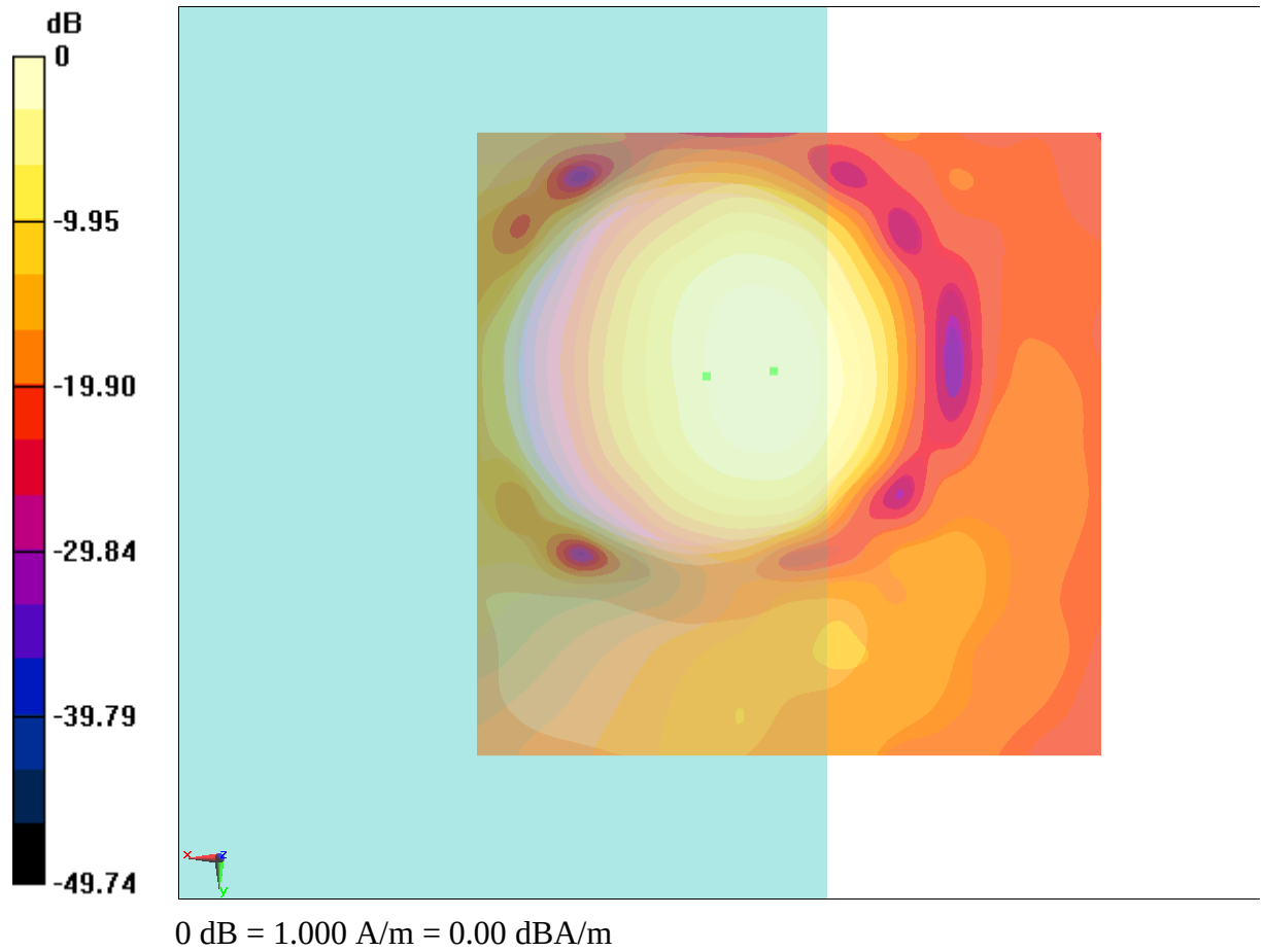
Fig B.10 T-Coil CDMA 1880_Channel 600
