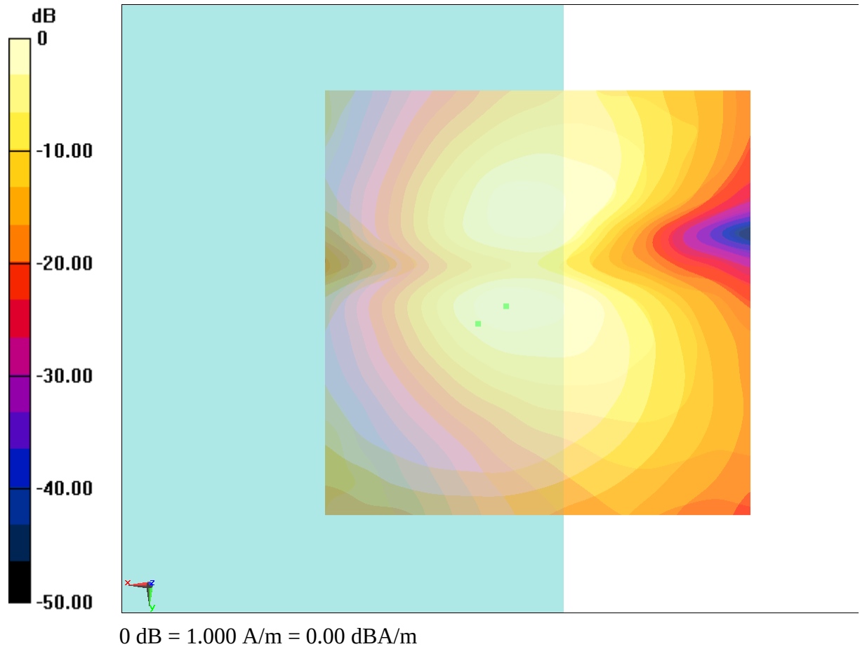
Fig B.11 T-Coil CDMA 1880_Channel 25
