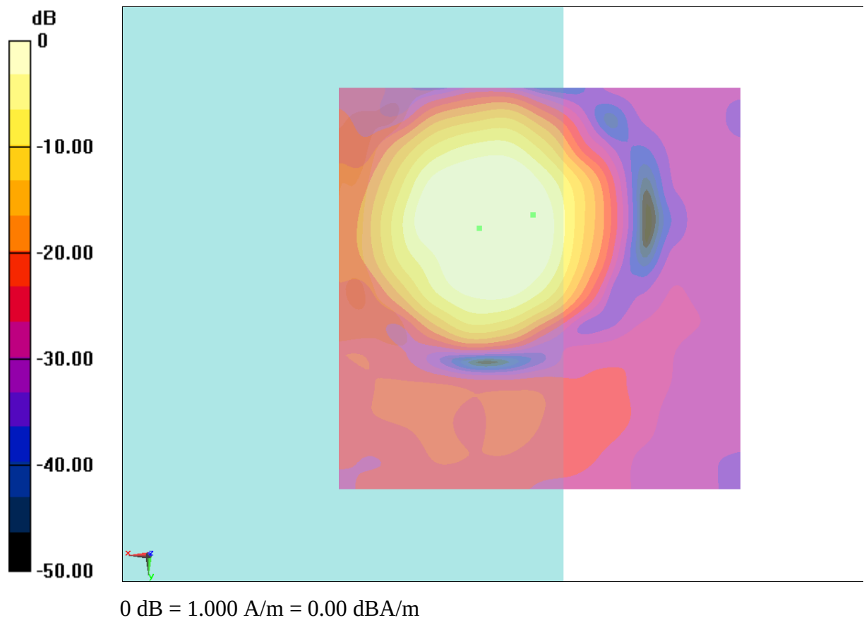
Fig B.2 T-Coil CDMA 835_Channel 777
