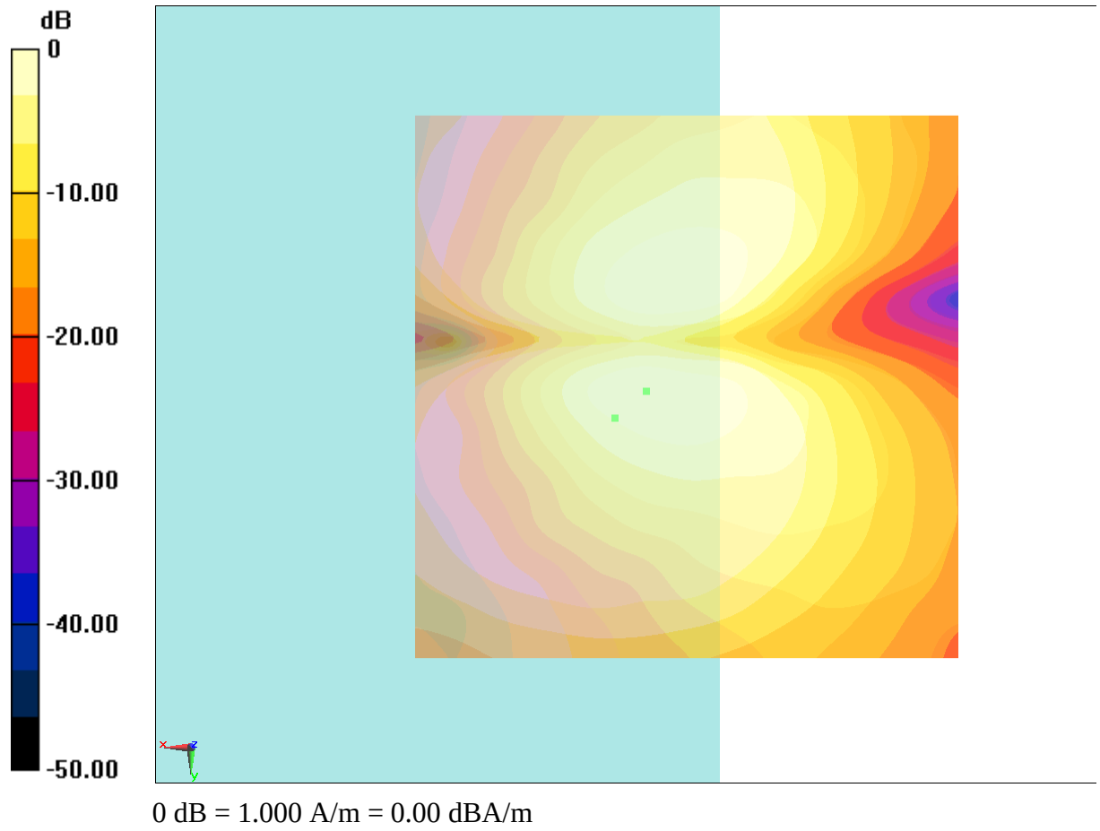
Fig B.7 T-Coil CDMA 1880_Channel 1175
