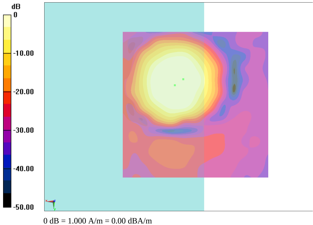
Fig B.6 T-Coil CDMA 835_Channel 1013
