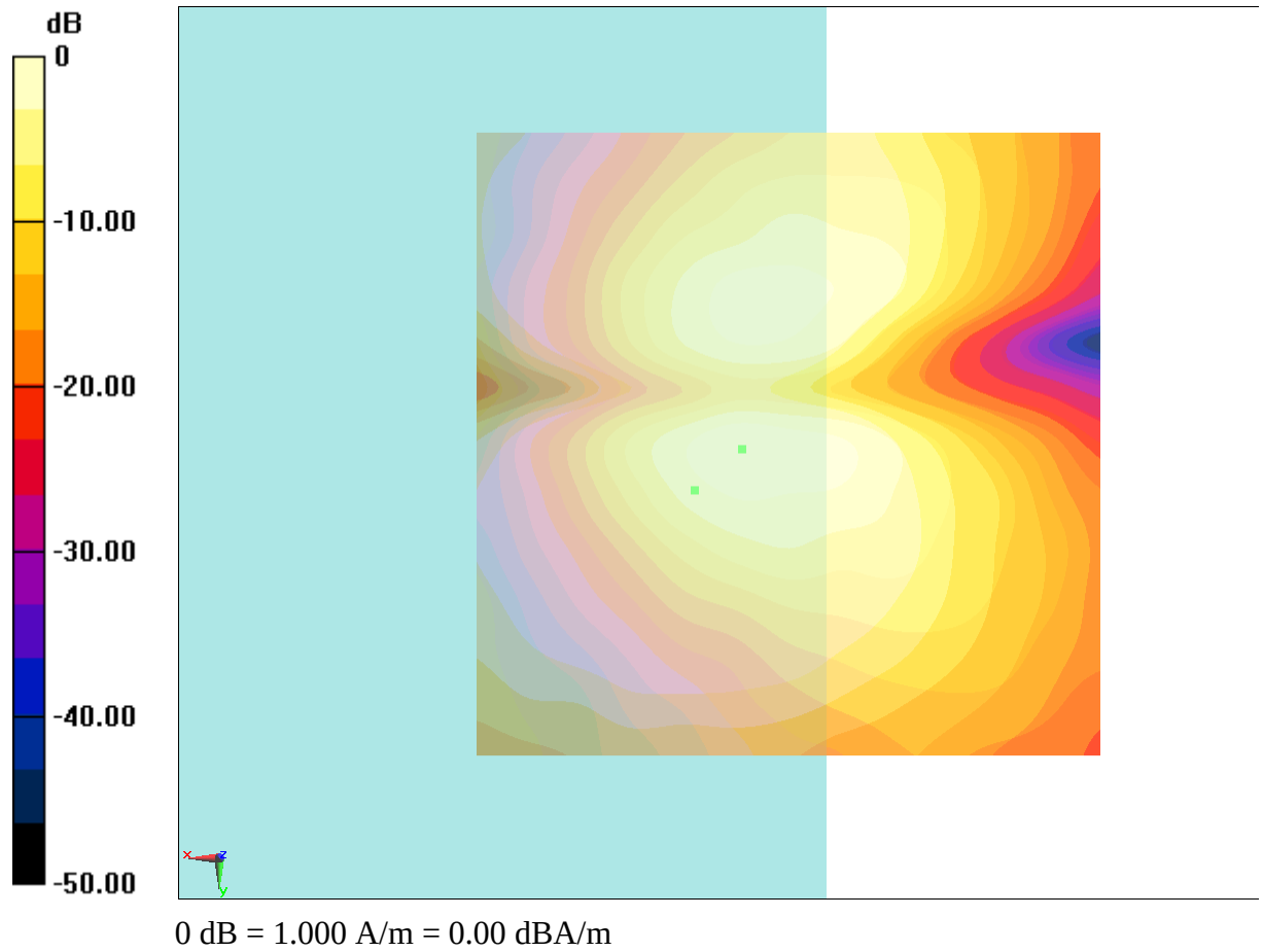
Fig B.9 T-Coil CDMA 1880_Channel 600
