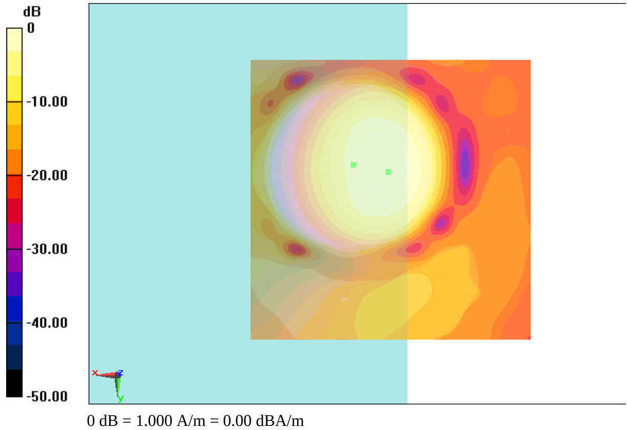
Fig B.8 T-Coil CDMA 1880_Channel 1175
