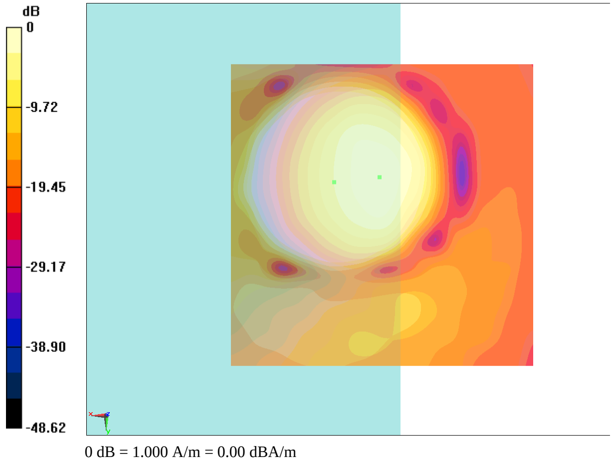
Fig B.12 T-Coil CDMA 1880_Channel 25
