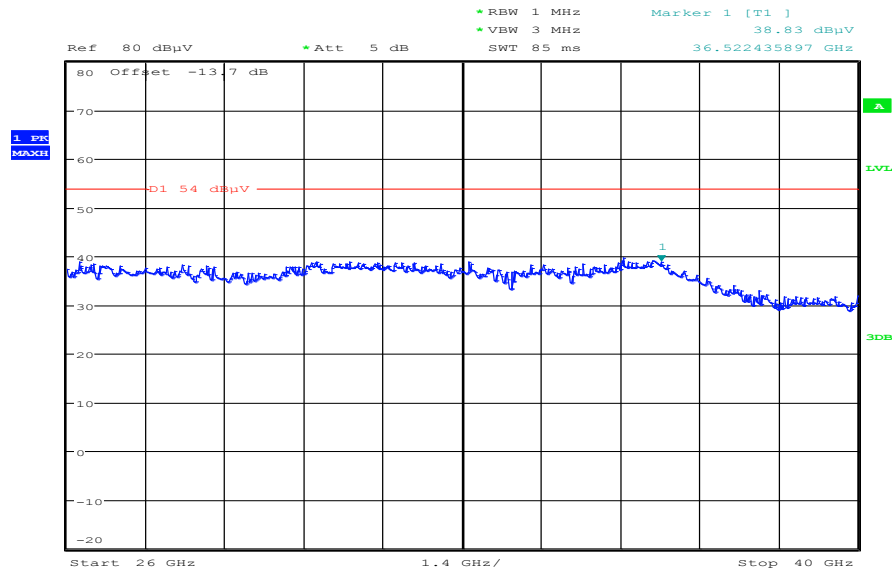
Plot 12: Highest channel, 26 GHz to 40 GHz, vertical & horizontal polarization
