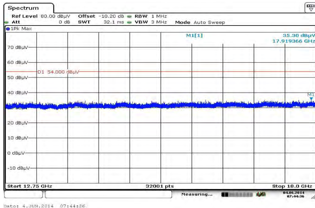
Plot 10: Highest channel, 12.75 GHz to 18 GHz, vertical & horizontal polarization
