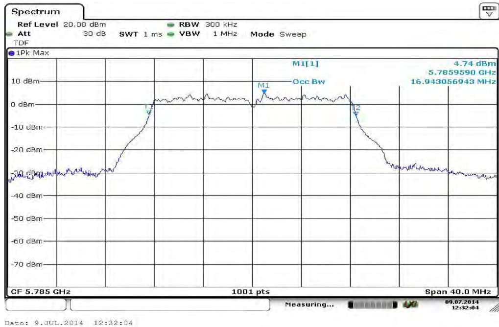
Plot 2: 5785 MHz
