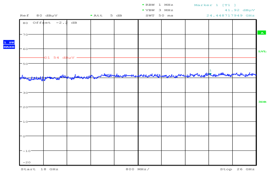
Plot 17: Highest channel, 18 GHz to 26 GHz, vertical & horizontal polarization
