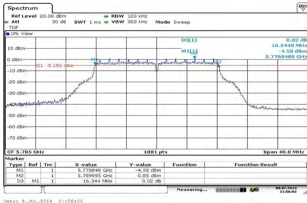
Plot 2: 5785 MHz
