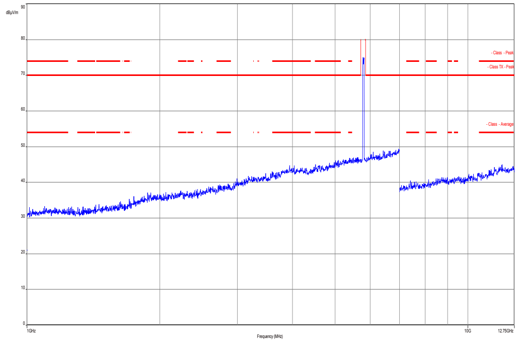
Plot 8: Highest channel, 1 GHz to 12.75 GHz, vertical & horizontal polarization
