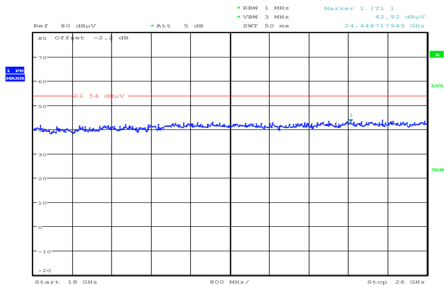
Plot 11: Middle channel, 18 GHz to 26 GHz, vertical & horizontal polarization
