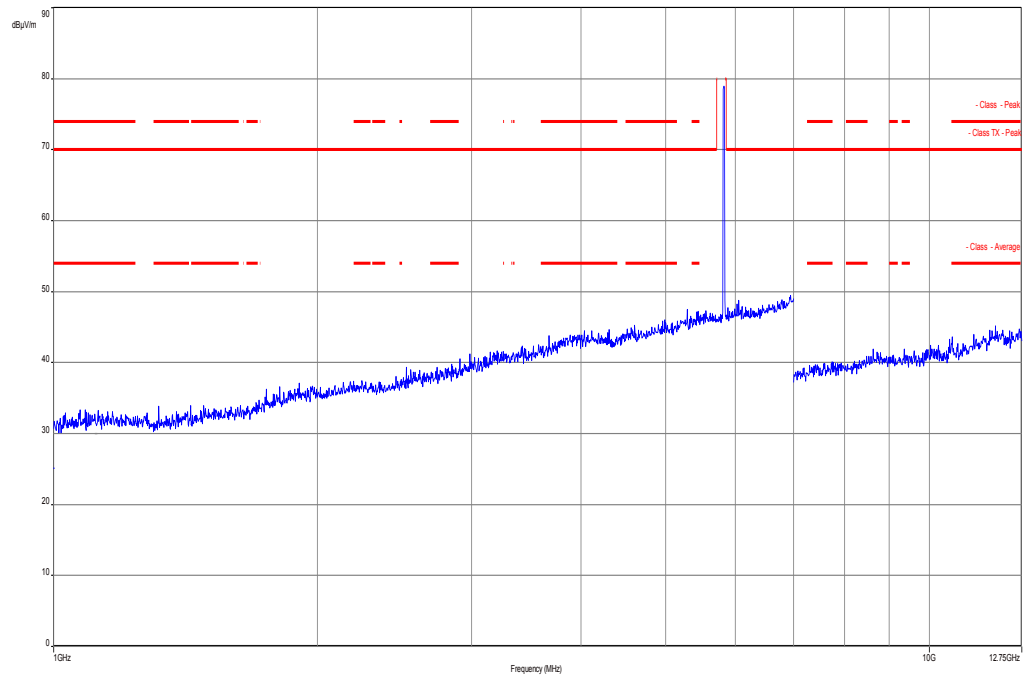
Plot 14: Highest channel, 1 GHz to 12.75 GHz, vertical & horizontal polarization
