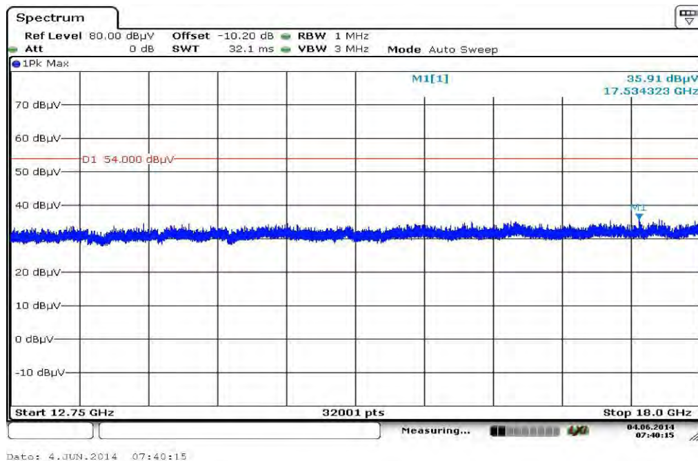
Plot 10: Middle channel, 12.75 GHz to 18 GHz, vertical & horizontal polarization
