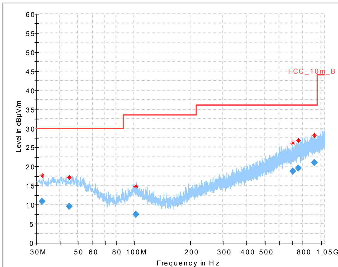
Plot 7: Middle channel, 30 MHz to 1 GHz, vertical & horizontal polarization
