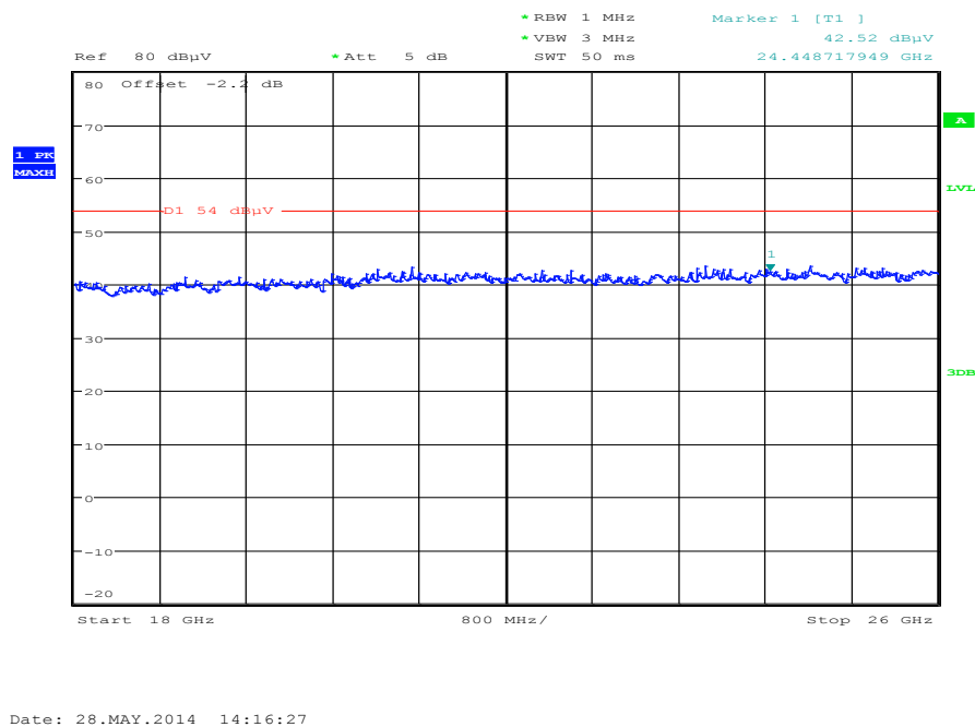
Plot 5: Lowest channel, 18 GHz to 26 GHz, vertical & horizontal polarization
