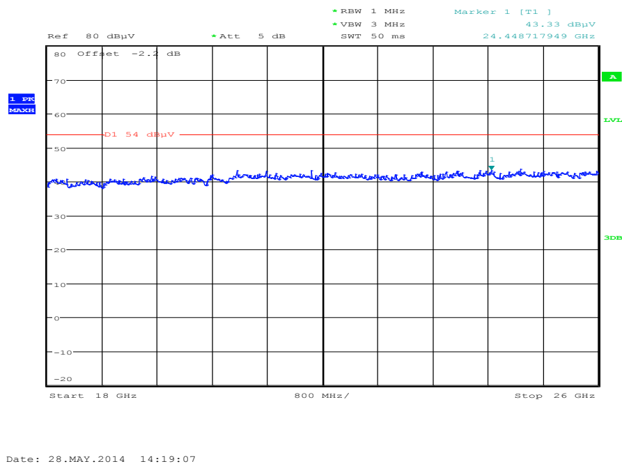
Plot 17: Highest channel, 18 GHz to 26 GHz, vertical & horizontal polarization
