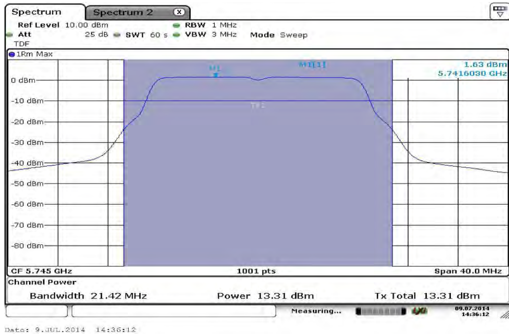
Plot 1: 5745 MHz
