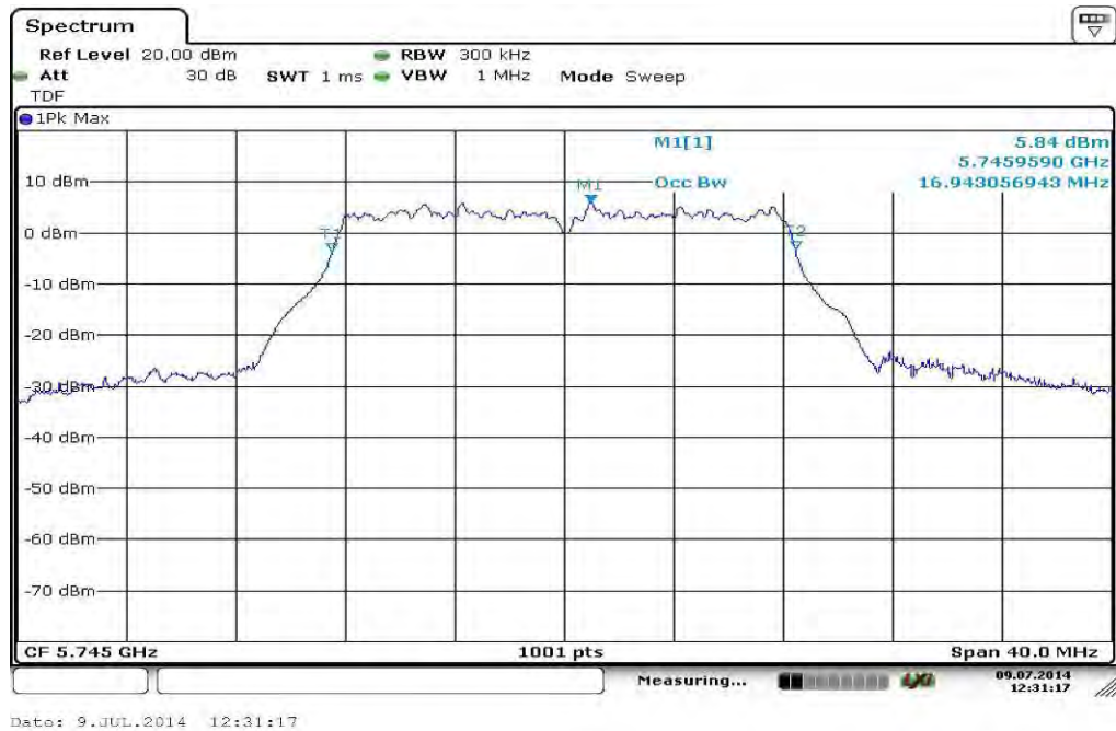
Plot 1: 5745 MHz
