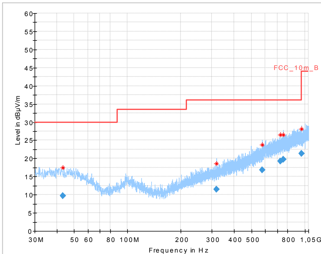
Plot 13: Highest channel, 30 MHz to 1 GHz, vertical & horizontal polarization
