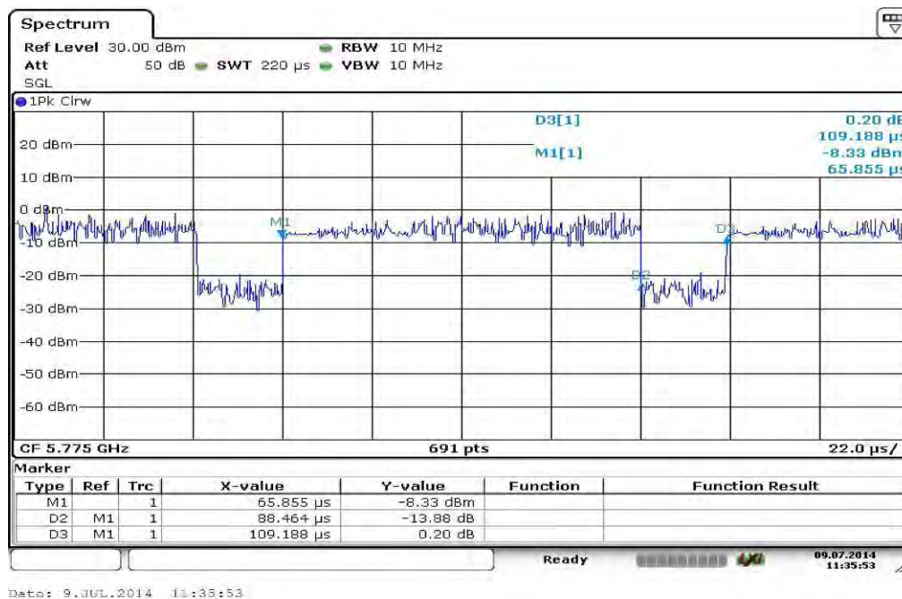
Plot 4: duty cycle of the transmitter – OFDM / ac – mode HT80
