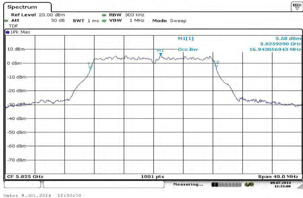
Plot 3: 5825 MHz
