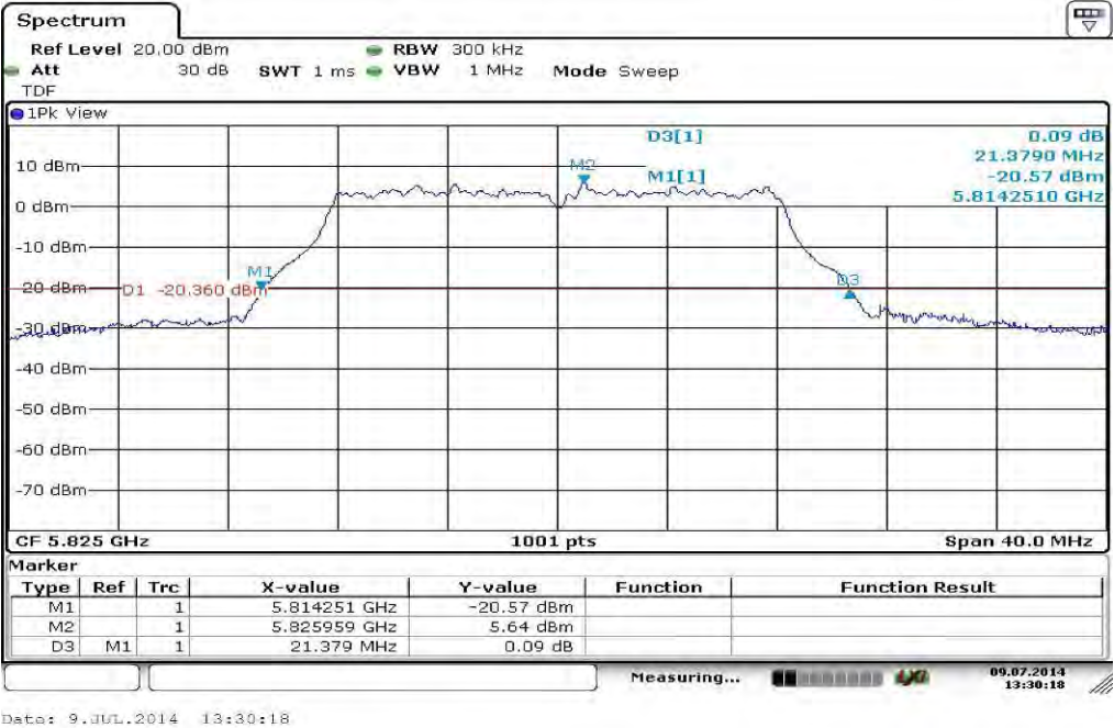
Plot 3: 5825 MHz
