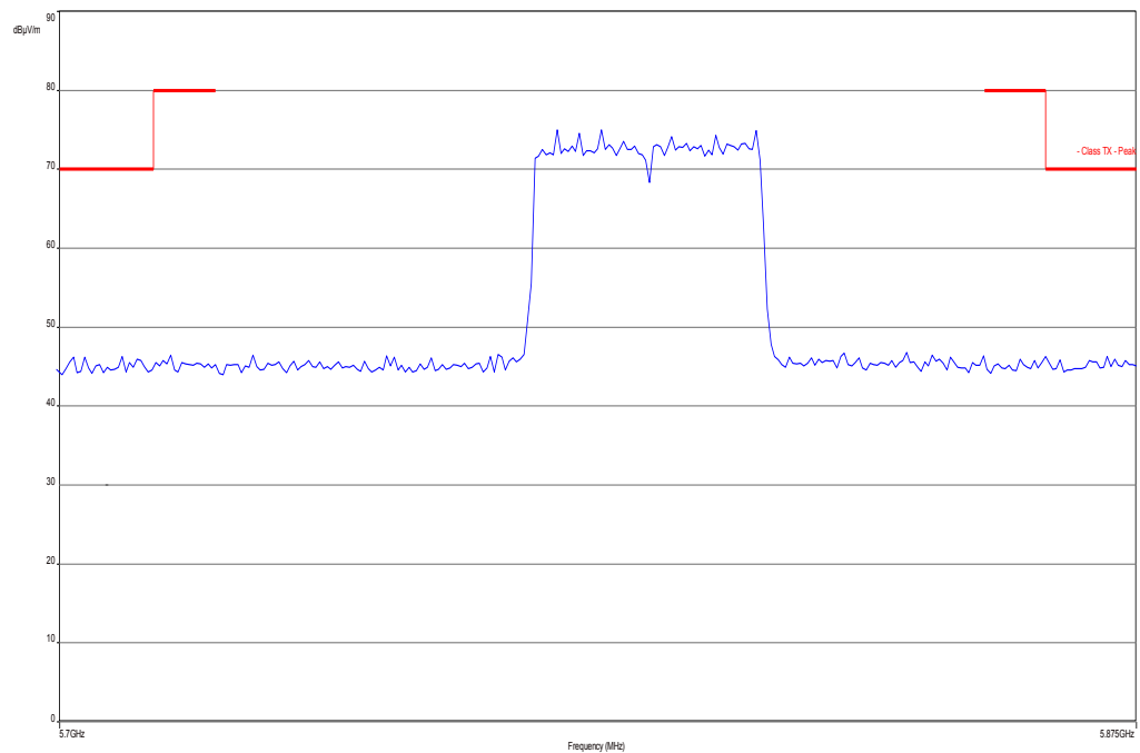
Plot 9: Highest channel, vertical & horizontal polarization, mask
