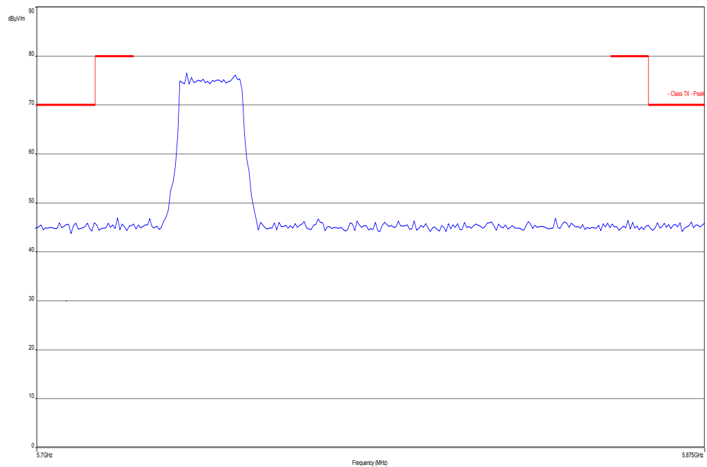
Plot 3: Lowest channel, vertical & horizontal polarization, mask
