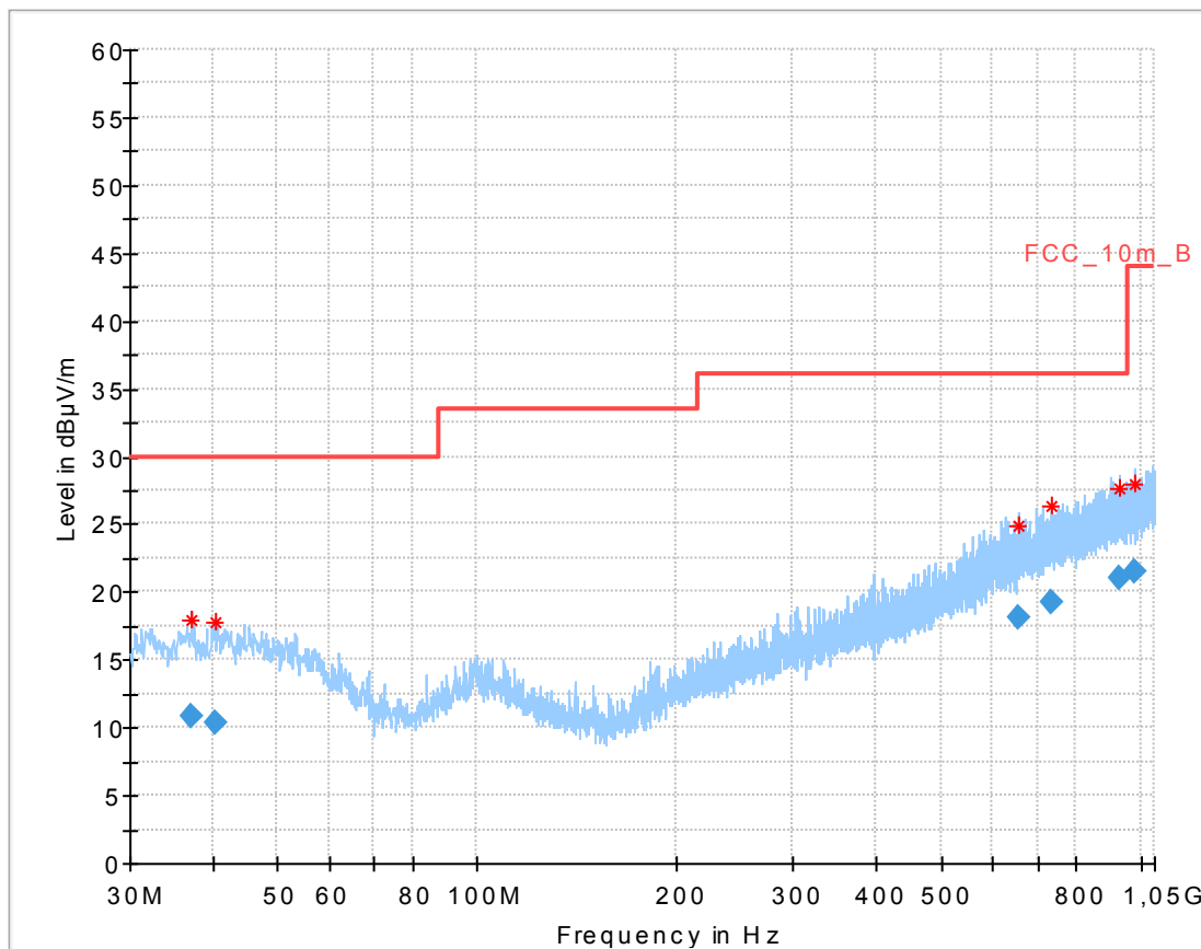
Plot 7: Highest channel, 30 MHz to 1 GHz, vertical & horizontal polarization
