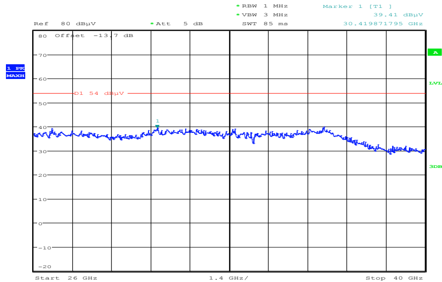
Plot 6: Lowest channel, 26 GHz to 40 GHz, vertical & horizontal polarization
