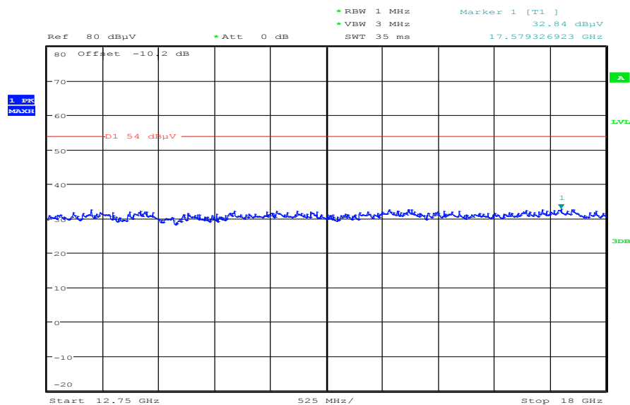
Plot 10: Middle channel, 12.75 GHz to 18 GHz, vertical & horizontal polarization
