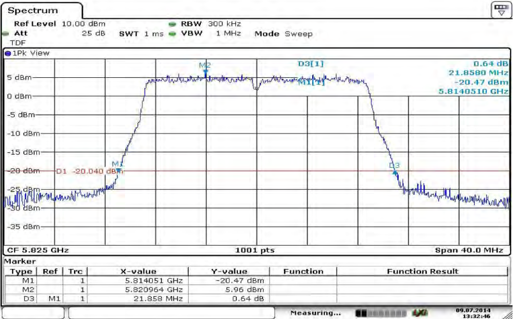
Plot 3: 5825 MHz
