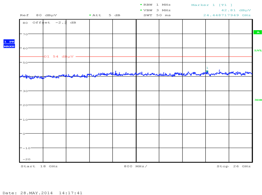
Plot 11: Middle channel, 18 GHz to 26 GHz, vertical & horizontal polarization
