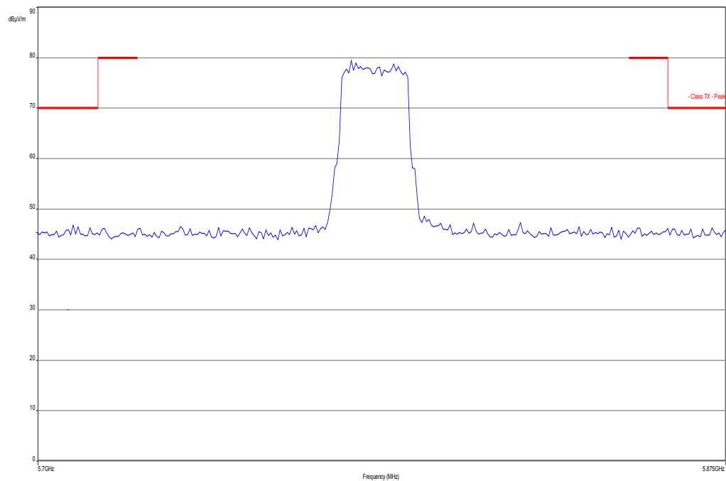
Plot 9: Middle channel, vertical & horizontal polarization, mask
