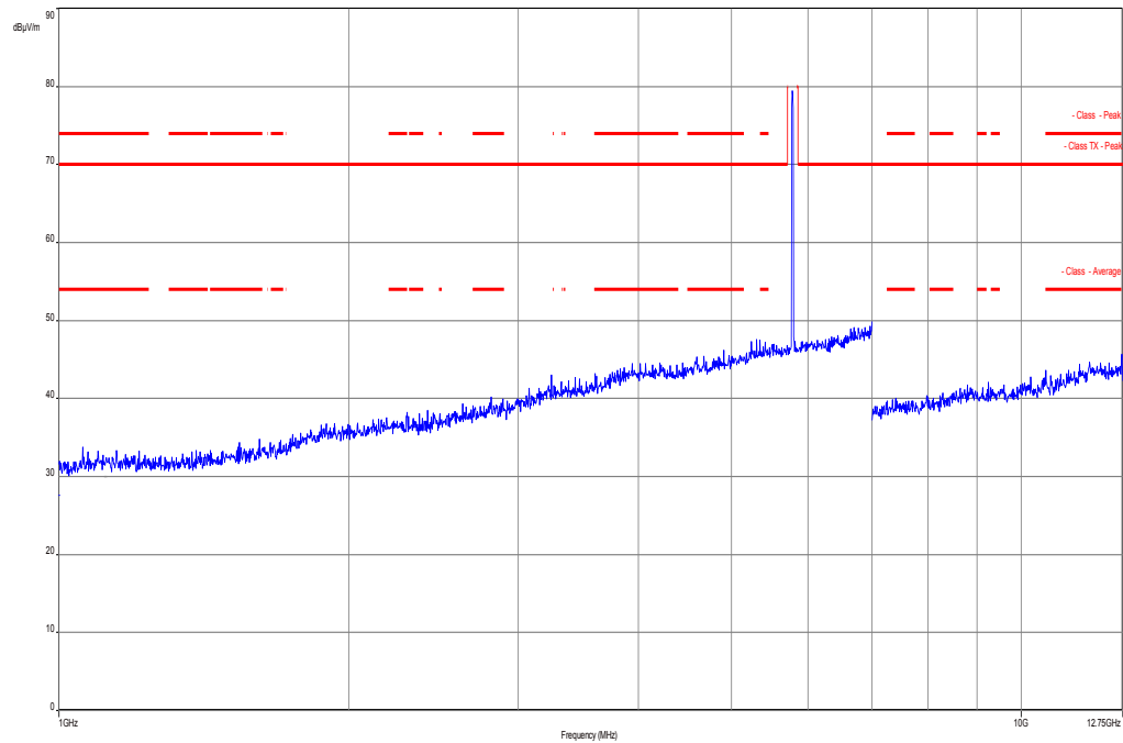
Plot 8: Middle channel, 1 GHz to 12.75 GHz, vertical & horizontal polarization
