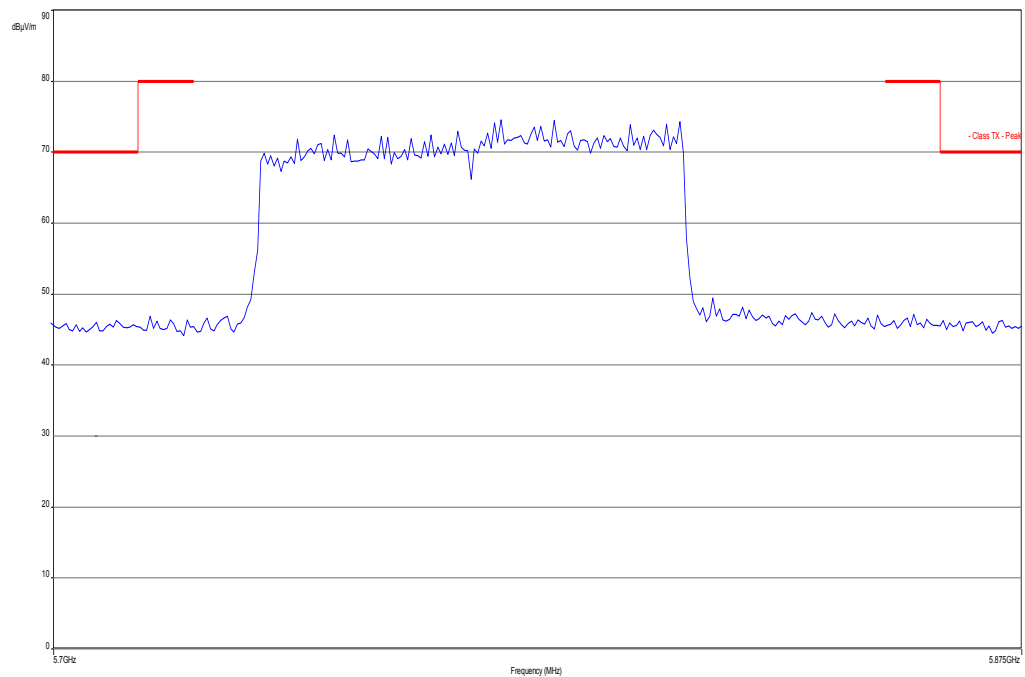
Plot 3: vertical & horizontal polarization, mask
