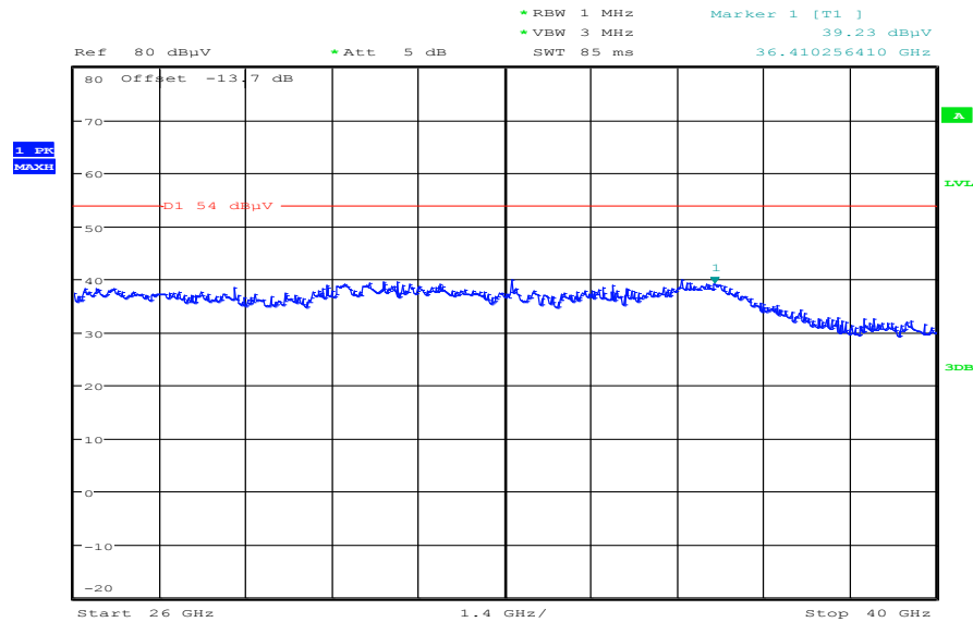
Plot 18: Highest channel, 26 GHz to 40 GHz, vertical & horizontal polarization
