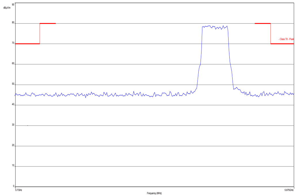
Plot 15: Highest channel, vertical & horizontal polarization, mask
