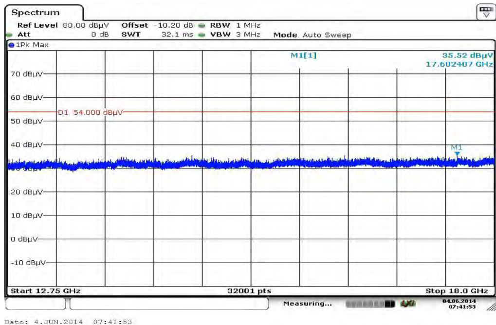
Plot 16: Highest channel, 12.75 GHz to 18 GHz, vertical & horizontal polarization
