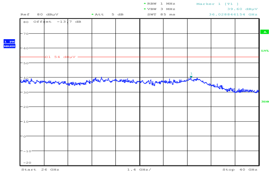
Plot 12: Middle channel, 26 GHz to 40 GHz, vertical & horizontal polarization
