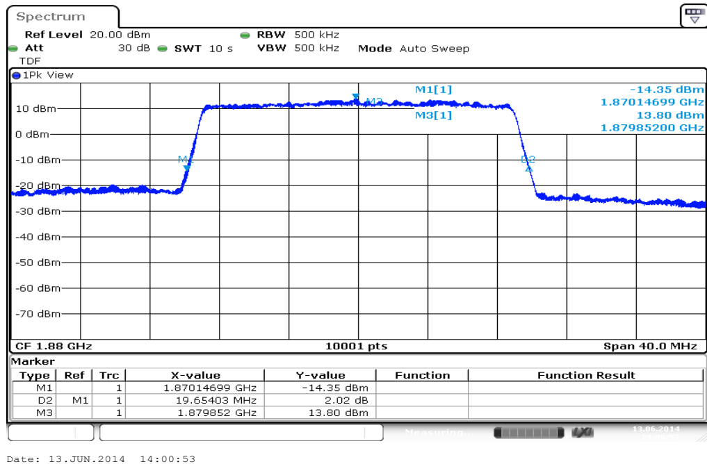
Plot 12: 20 MHz (-26 dBc BW)
