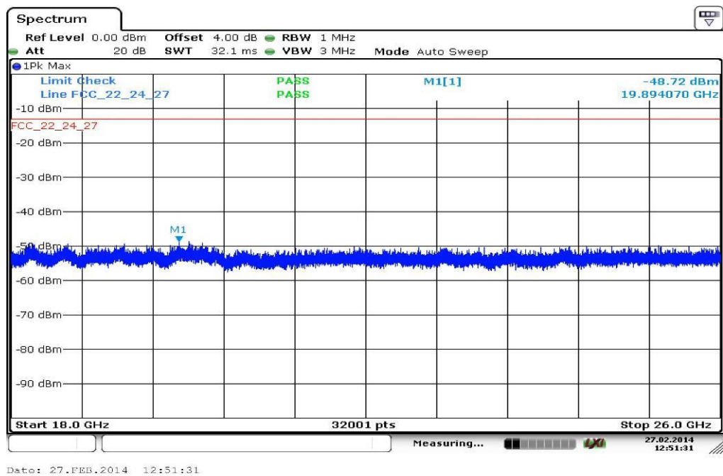
Plot 4: Channel 9400 (18 GHz - 26 GHz)
