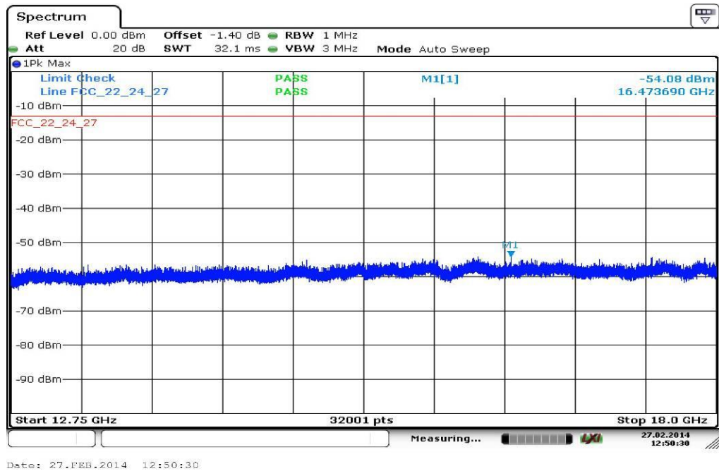
Plot 3: Channel 9400 (12.75 GHz - 18 GHz)
