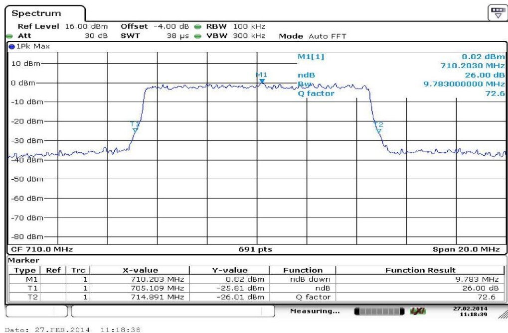
Plot 4: 10 MHz, -26 dBc OBW
