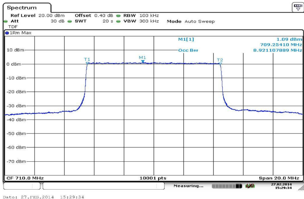
Plot 3: 10 MHz, 99% OBW
