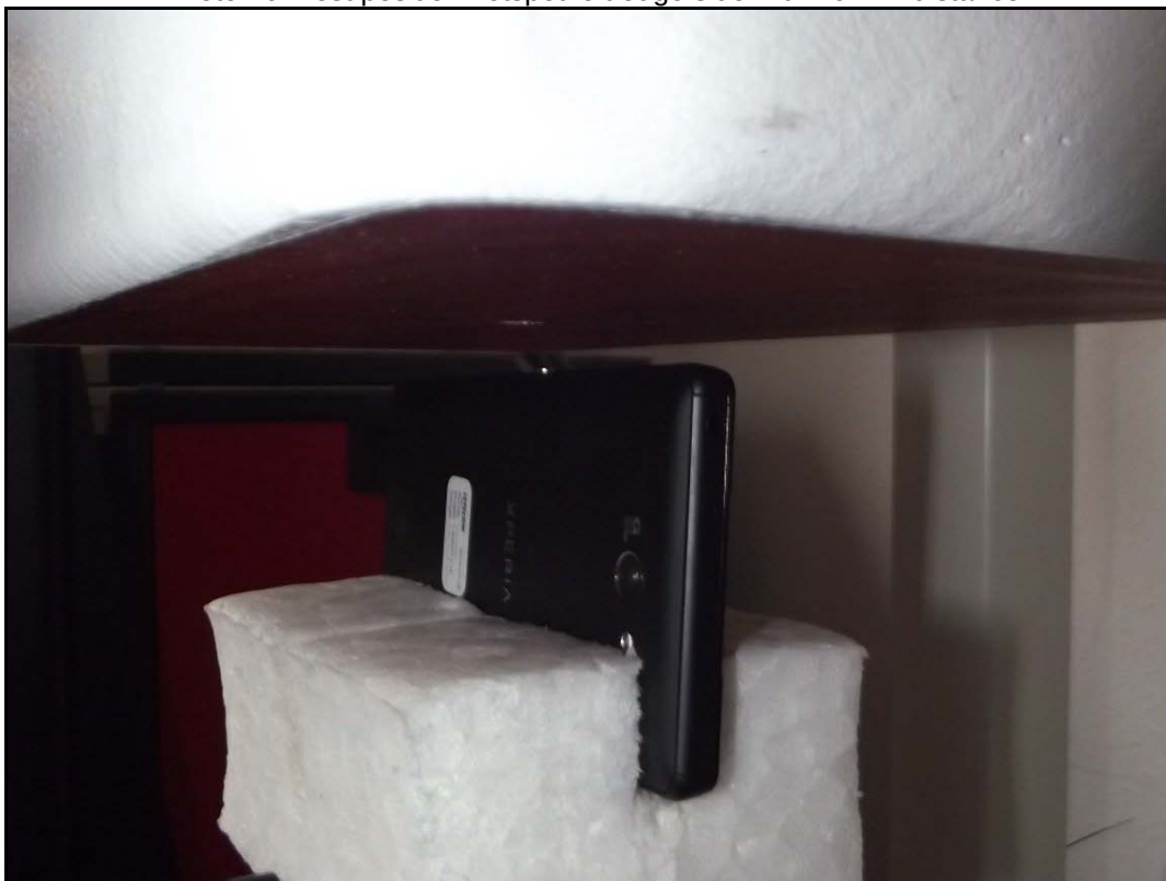
Photo 20: Test position hotspot left edge side with 10 mm distance
