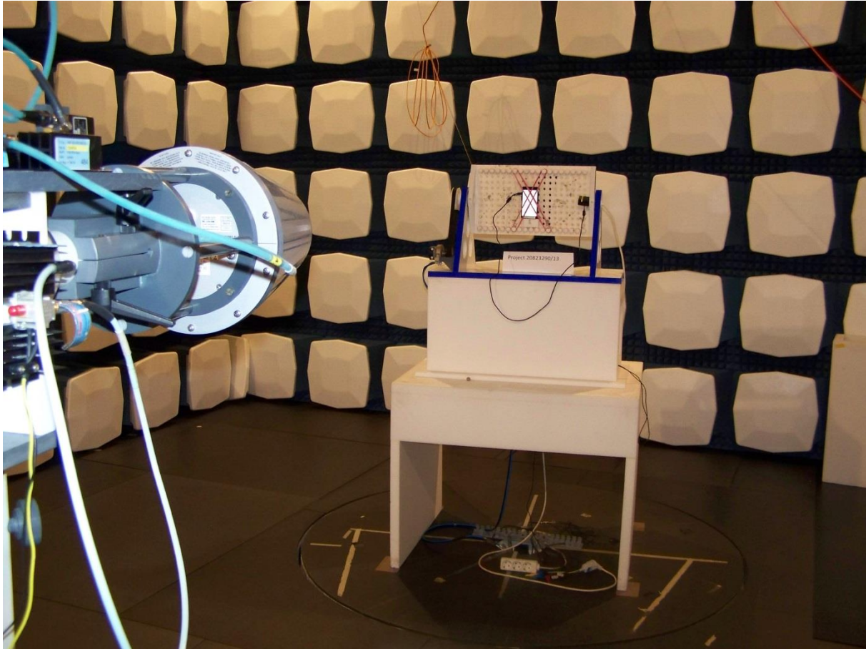
Photograph 3: Electrical field measurements above 1GHz
