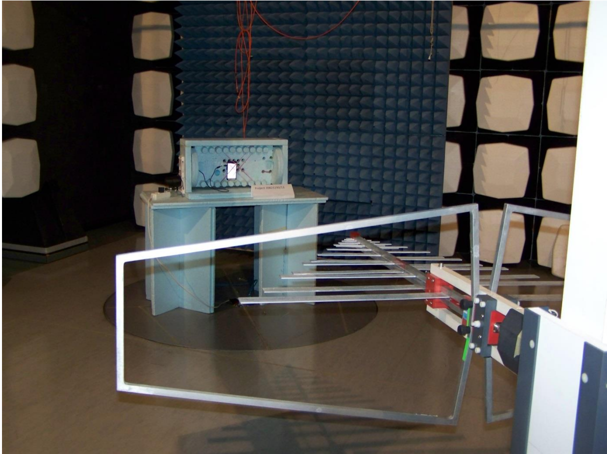
Photograph 2: Electrical field measurements up to 1GHz
