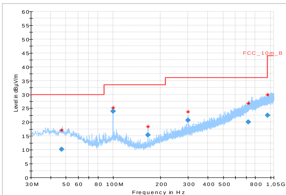
Plot 2: Receiver mode 30 MHz to 1 GHz
