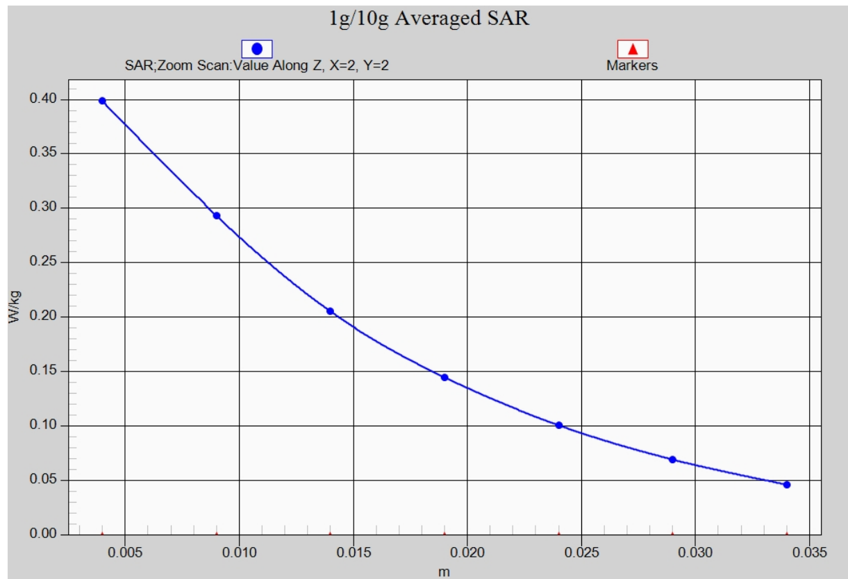
Fig. 7-1 Z-Scan at power reference point (1700 MHz CH1312)
