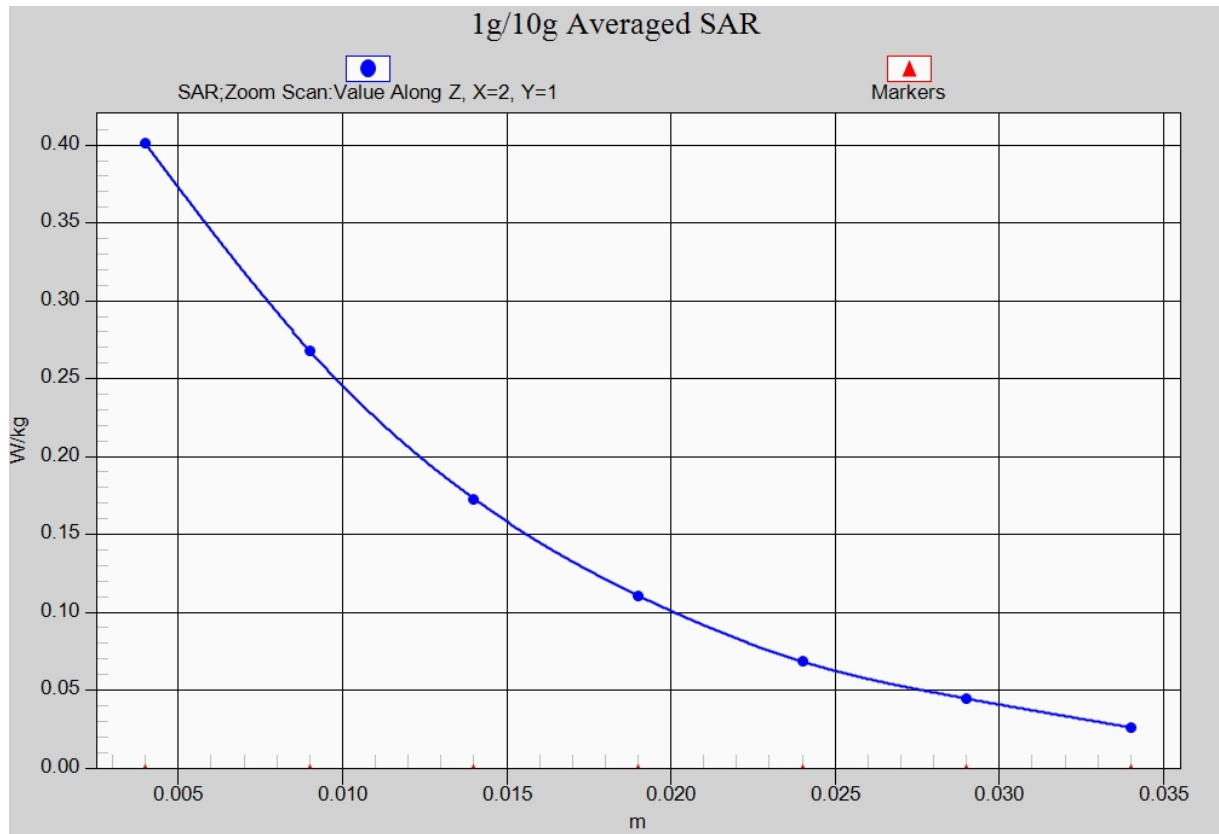
Fig. 8-1 Z-Scan at power reference point (1700 MHz CH1312)
