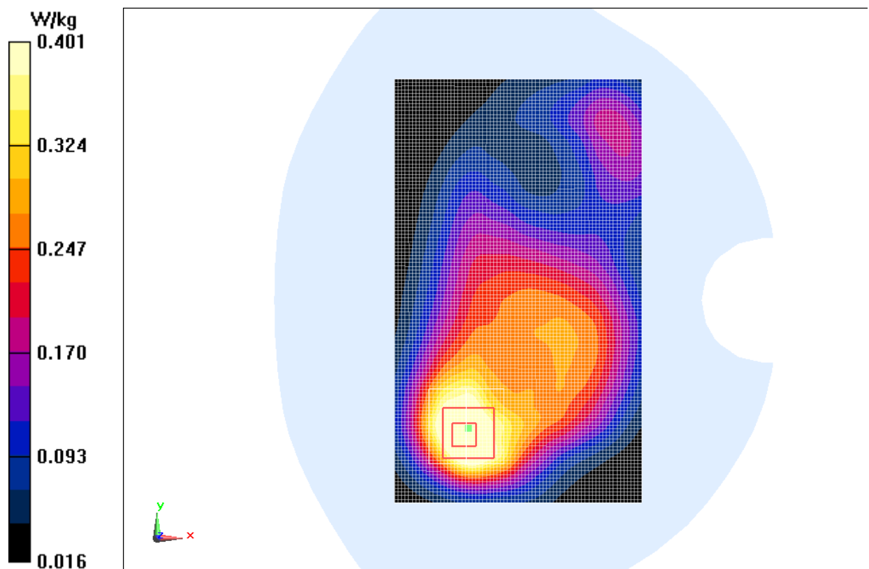
Fig.8 1700 MHz CH1312
