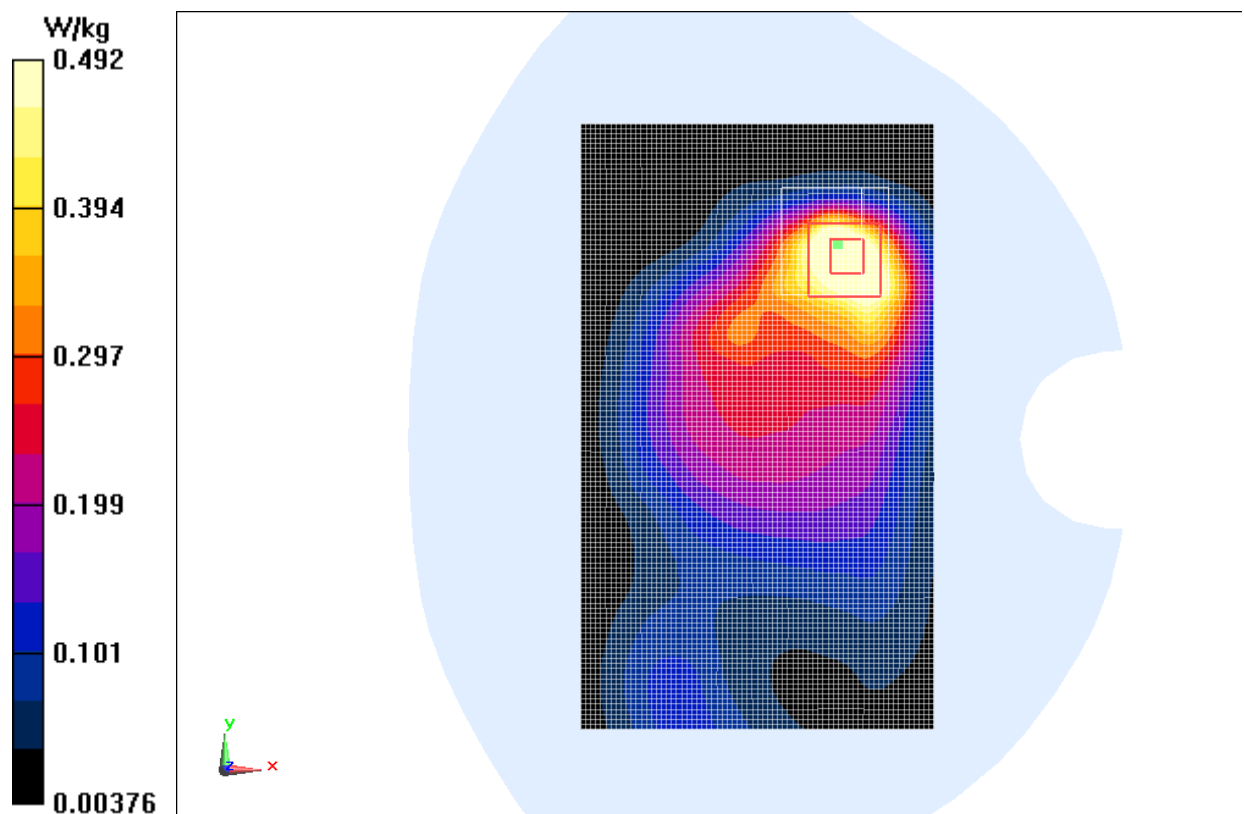
Fig.9 1700 MHz CH1312
