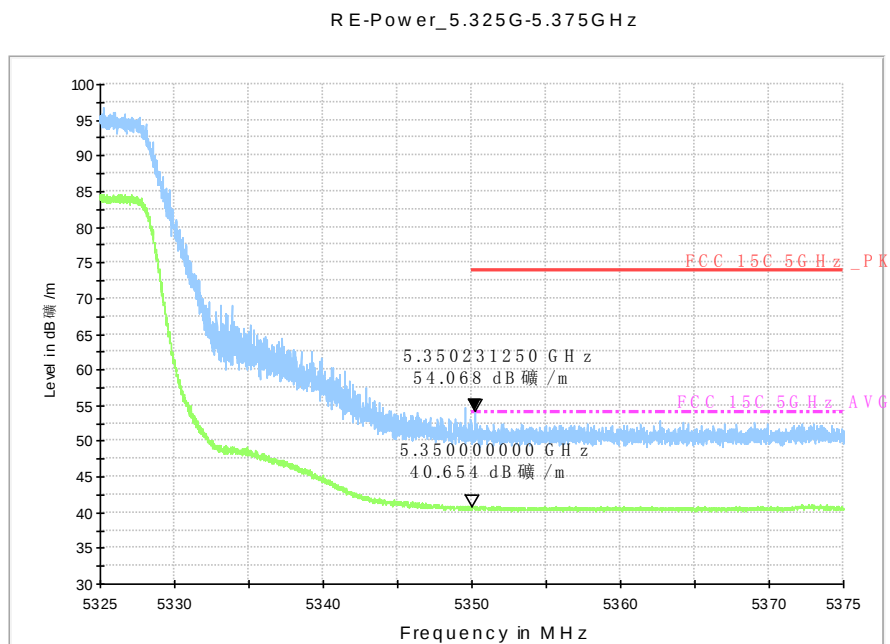
Fig. 36 Band Edges (802.11a, 5320MHz)
