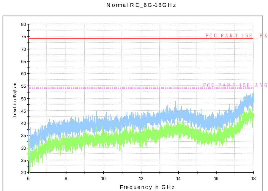
Fig. 131 Radiated Spurious Emission (802.11n-HT40, ch110, 6 GHz-18 GHz)
