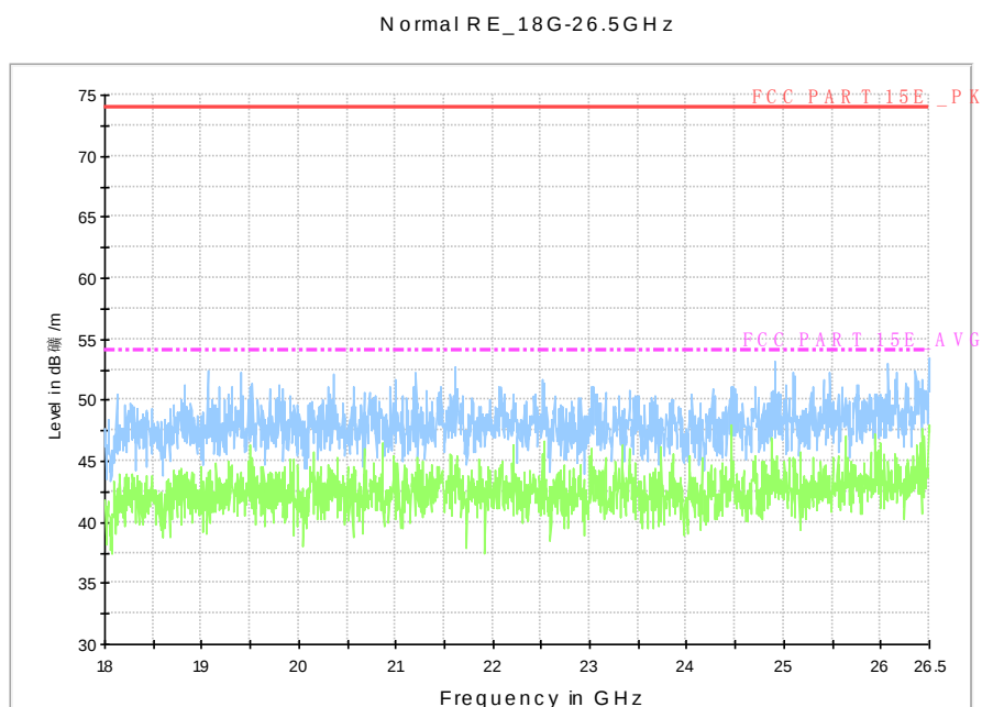
Fig. 116 Radiated Spurious Emission (802.11n-HT40, U-NII 1, 18 GHz-26.5 GHz)
