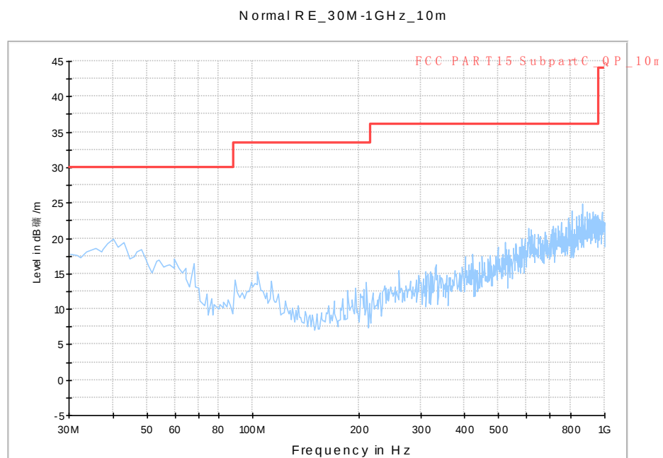
Fig. 72 Radiated Spurious Emission (802.11a, ch140, 30 MHz-1 GHz)
