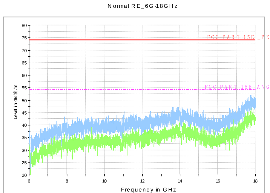
Fig. 74 Radiated Spurious Emission (802.11a, ch140, 6 GHz-18 GHz)
