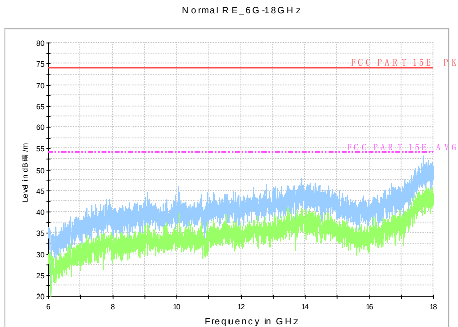
Fig. 63 Radiated Spurious Emission (802.11a, ch64, 6 GHz-18 GHz)
