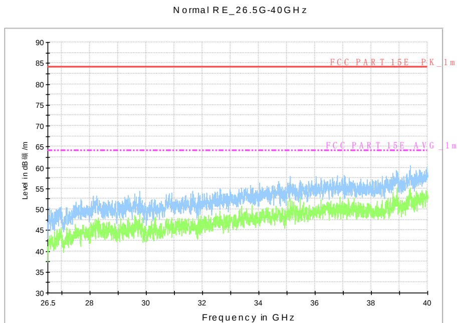
Fig. 76 Radiated Spurious Emission (802.11a, U-NII 3, 26.5 GHz-40 GHz)
