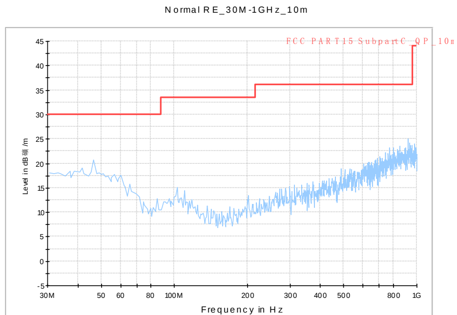
Fig. 58 Radiated Spurious Emission (802.11a, ch56, 30 MHz-1 GHz)
