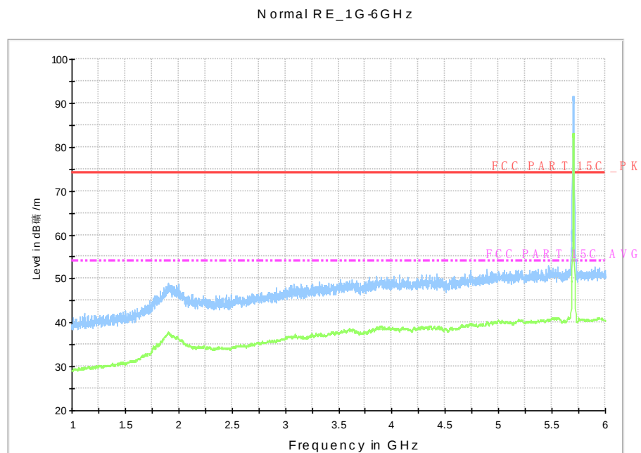
Fig. 73 Radiated Spurious Emission (802.11a, ch140, 1 GHz-6 GHz)
