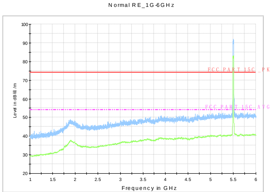
Fig. 67 Radiated Spurious Emission (802.11a, ch100, 1 GHz-6 GHz)
