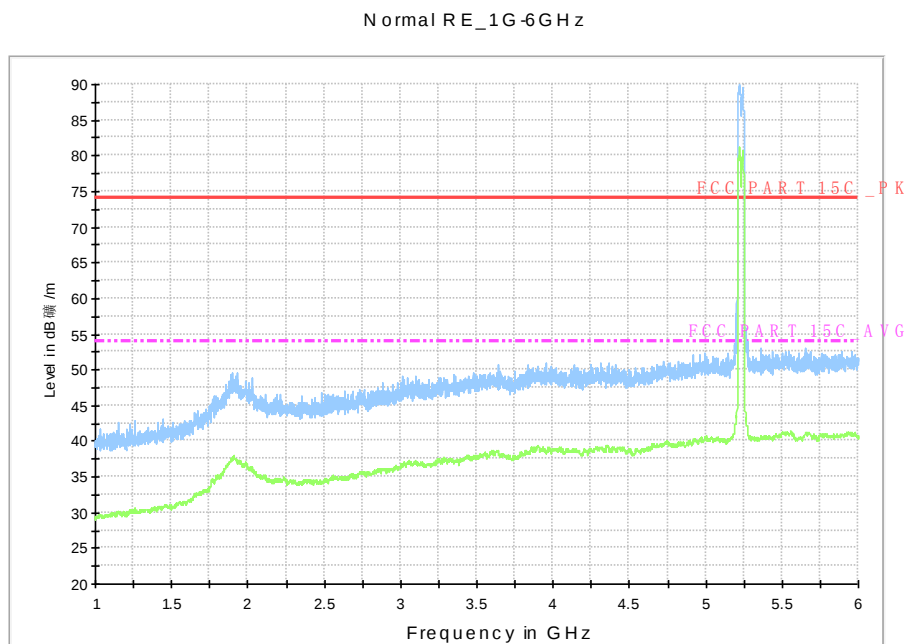
Fig. 114 Radiated Spurious Emission (802.11n-HT40, ch46, 1 GHz-6 GHz)
