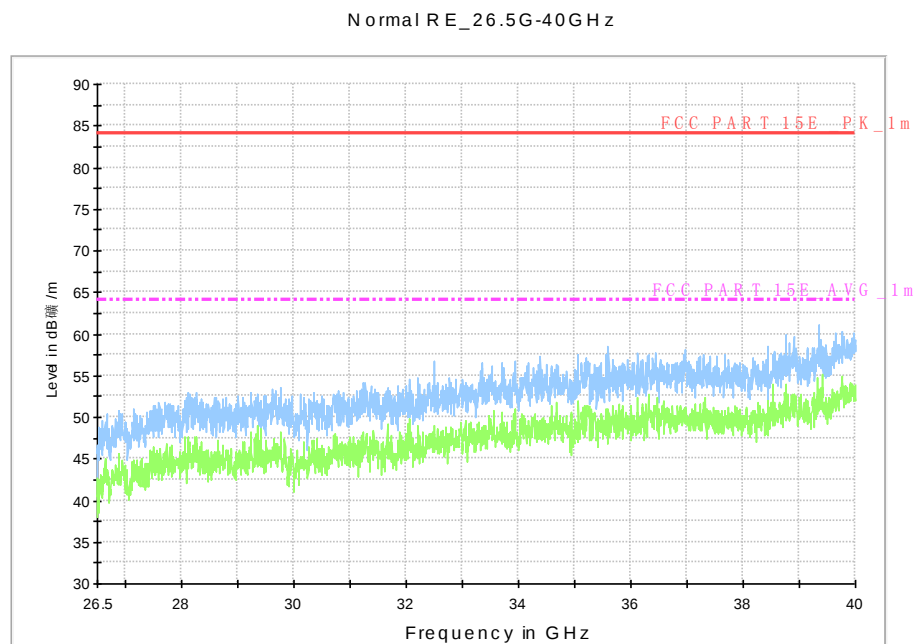
Fig. 125 Radiated Spurious Emission (802.11n-HT40, U-NII 2, 26.5 GHz-40 GHz)
