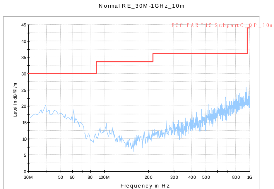
Fig. 110 Radiated Spurious Emission (802.11n-HT40, ch38, 30 MHz-1 GHz)
