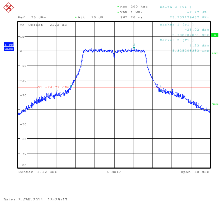
Fig. 6 Occupied 26dB Bandwidth (802.11a, 5320MHz)
