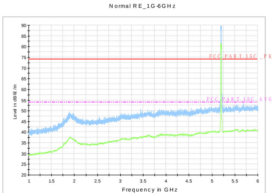
Fig. 81 Radiated Spurious Emission (802.11n-HT20, ch40, 1 GHz-6 GHz)
