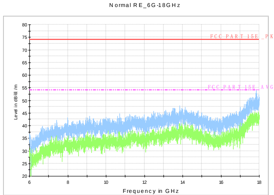
Fig. 49 Radiated Spurious Emission (802.11a, ch40, 6 GHz-18 GHz)
