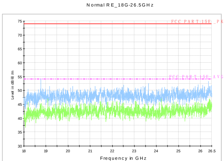
Fig. 64 Radiated Spurious Emission (802.11a, U-NII 2, 18 GHz-26.5 GHz)
