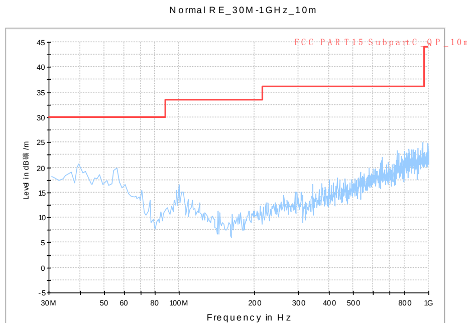
Fig. 77 Radiated Spurious Emission (802.11n-HT20, ch36, 30 MHz-1 GHz)
