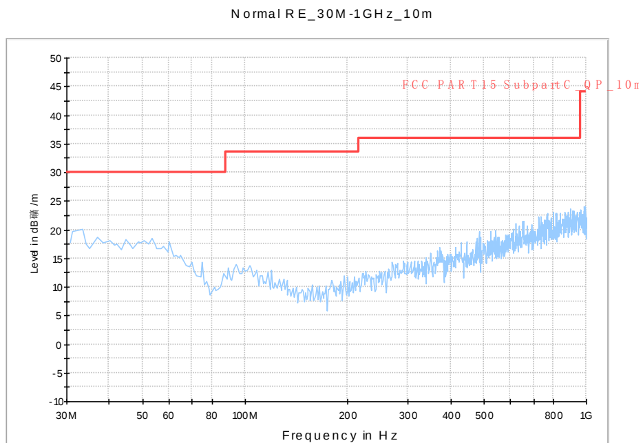
Fig. 99 Radiated Spurious Emission (802.11n-HT20, ch100, 30 MHz-1 GHz)
