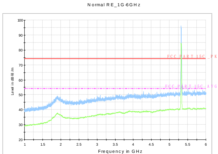
Fig. 62 Radiated Spurious Emission (802.11a, ch64, 1 GHz-6 GHz)
