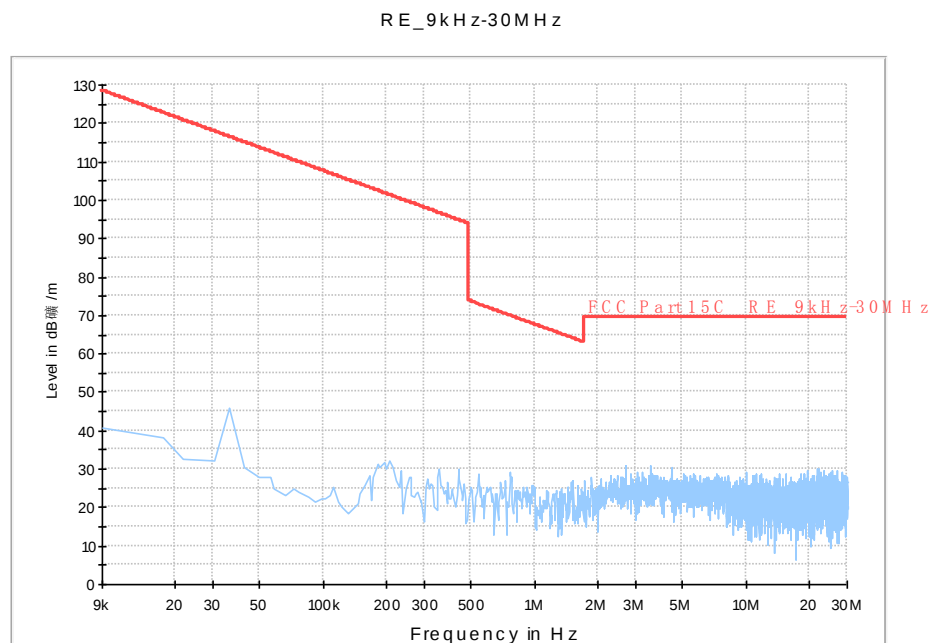
Fig. 137 Radiated Spurious Emission (802.11a, ch40, 9 kHz ~30 MHz)
