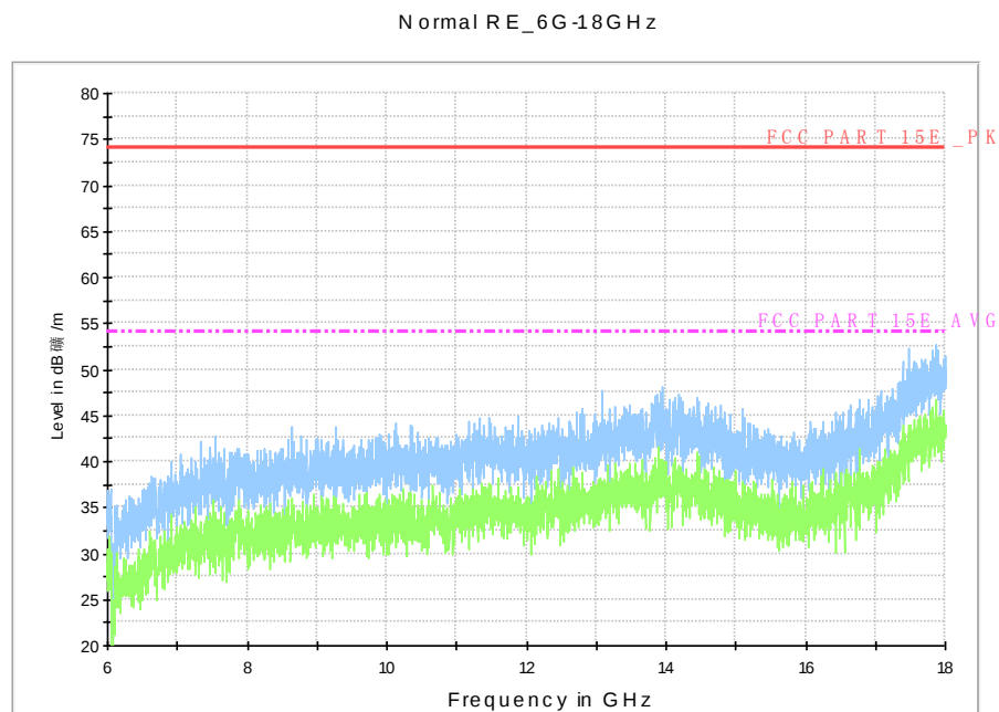
Fig. 112 Radiated Spurious Emission (802.11n-HT40, ch38, 6 GHz-18 GHz)
