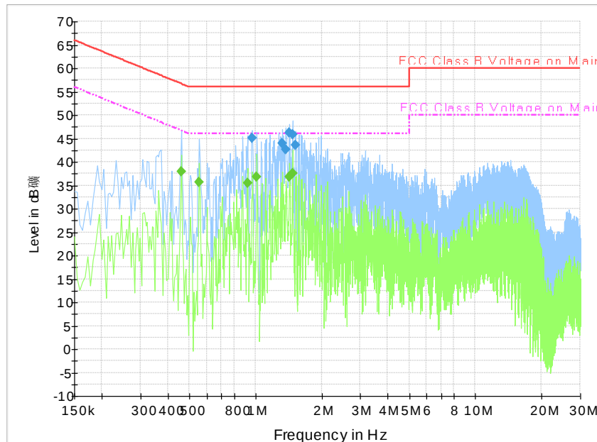
Fig. 139 Conducted Emission(802.11a, IDLE)
