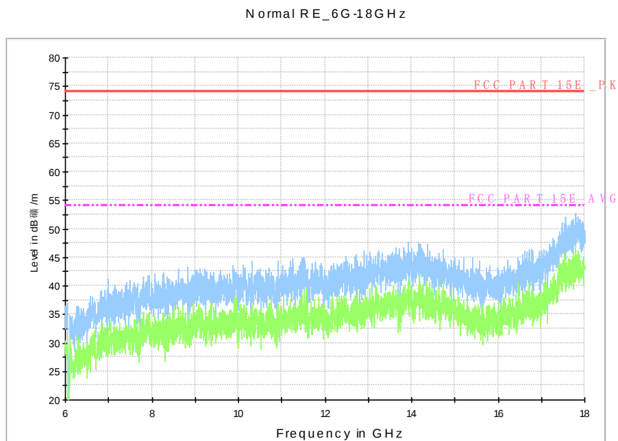
Fig. 104 Radiated Spurious Emission (802.11n-HT20, ch116, 6 GHz-18 GHz)
