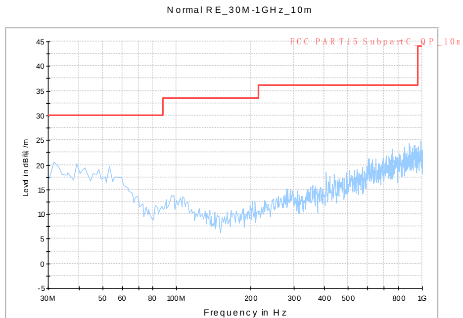
Fig. 55 Radiated Spurious Emission (802.11a, ch52, 30 MHz-1 GHz)
