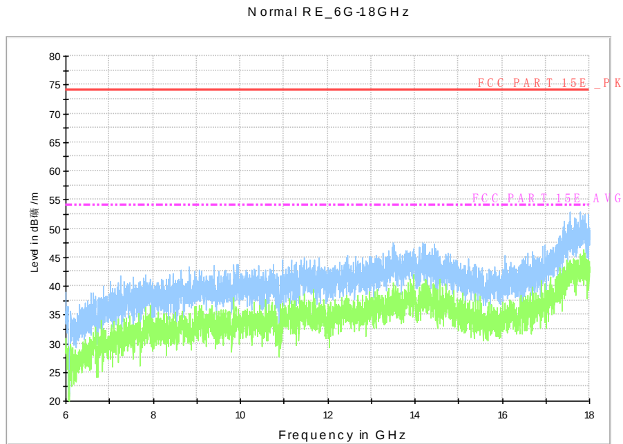
Fig. 107 Radiated Spurious Emission (802.11n-HT20, ch140, 6 GHz-18 GHz)
