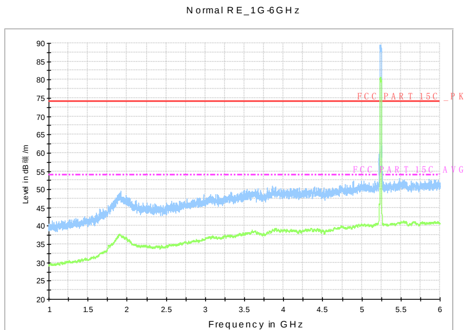
Fig. 84 Radiated Spurious Emission (802.11n-HT20, ch48, 1 GHz-6 GHz)
