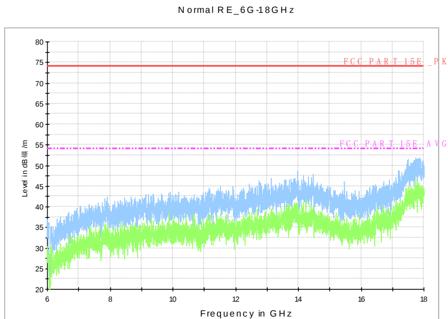
Fig. 128 Radiated Spurious Emission (802.11n-HT40, ch102, 6 GHz-18 GHz)
