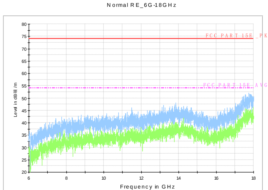
Fig. 57 Radiated Spurious Emission (802.11a, ch52, 6 GHz-18 GHz)
