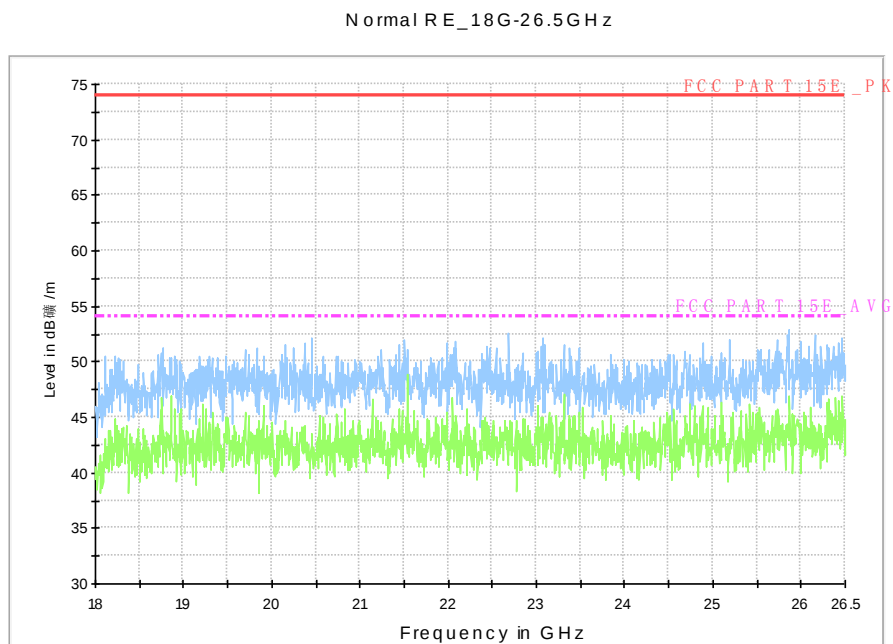
Fig. 97 Radiated Spurious Emission (802.11n-HT20, U-NII 2, 18 GHz-26.5 GHz)
