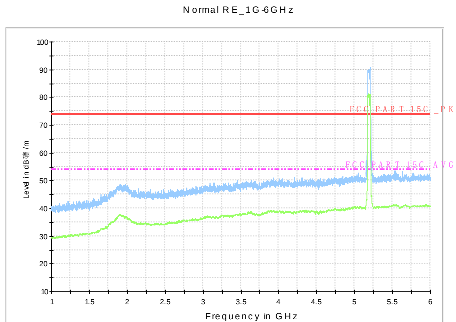
Fig. 111 Radiated Spurious Emission (802.11n-HT40, ch38, 1 GHz-6 GHz)
