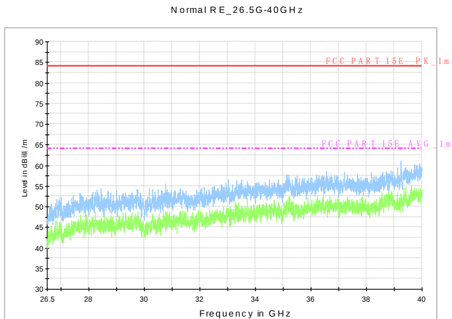
Fig. 117 Radiated Spurious Emission (802.11n-HT40, U-NII 1, 26.5 GHz-40 GHz)
