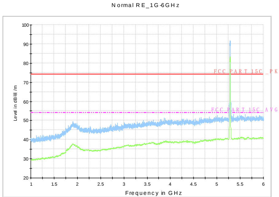
Fig. 59 Radiated Spurious Emission (802.11a, ch56, 1 GHz-6 GHz)
