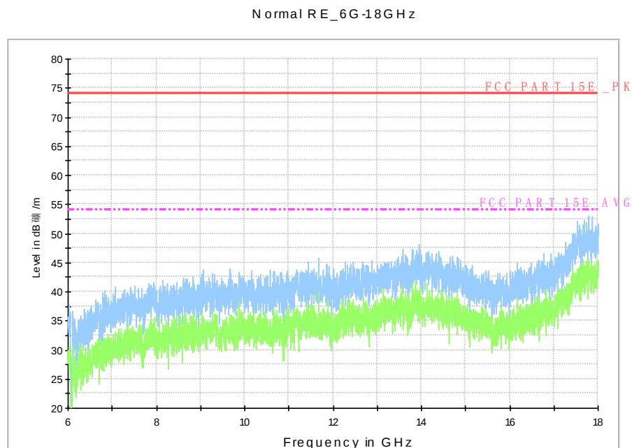
Fig. 46 Radiated Spurious Emission (802.11a, ch36, 6 GHz-18 GHz)
