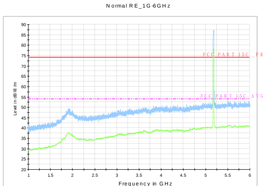
Fig. 78 Radiated Spurious Emission (802.11n-HT20, ch36, 1 GHz-6 GHz)
