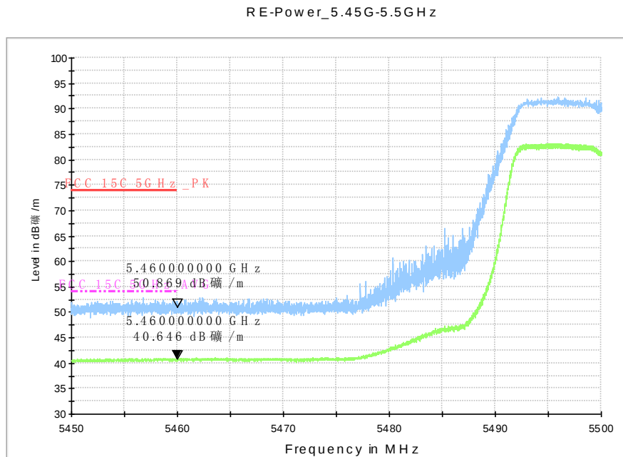
Fig. 37 Band Edges (802.11a, 5500MHz)
