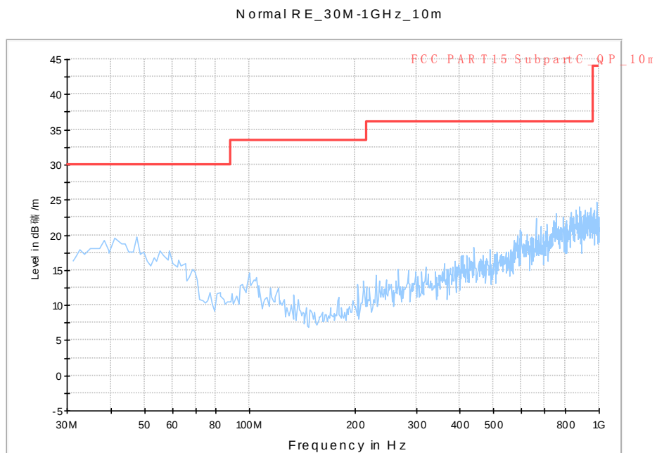
Fig. 102 Radiated Spurious Emission (802.11n-HT20, ch116, 30 MHz-1 GHz)
