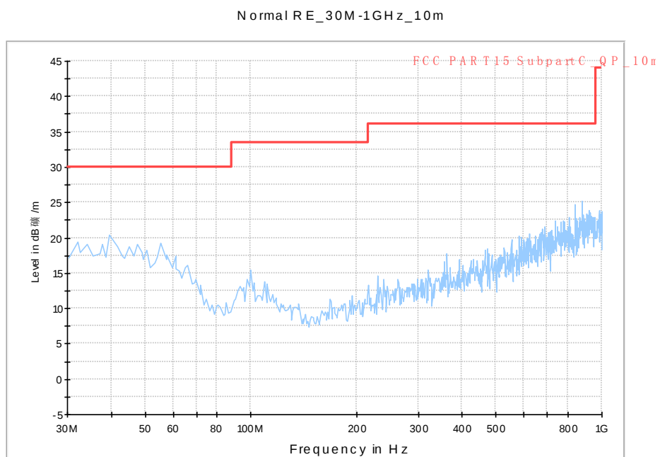
Fig. 118 Radiated Spurious Emission (802.11n-HT40, ch54, 30 MHz-1 GHz)
