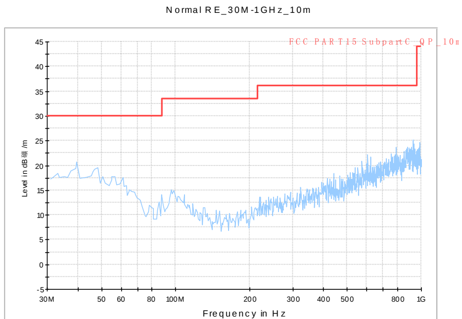
Fig. 132 Radiated Spurious Emission (802.11n-HT40, ch134, 30 MHz-1 GHz)
