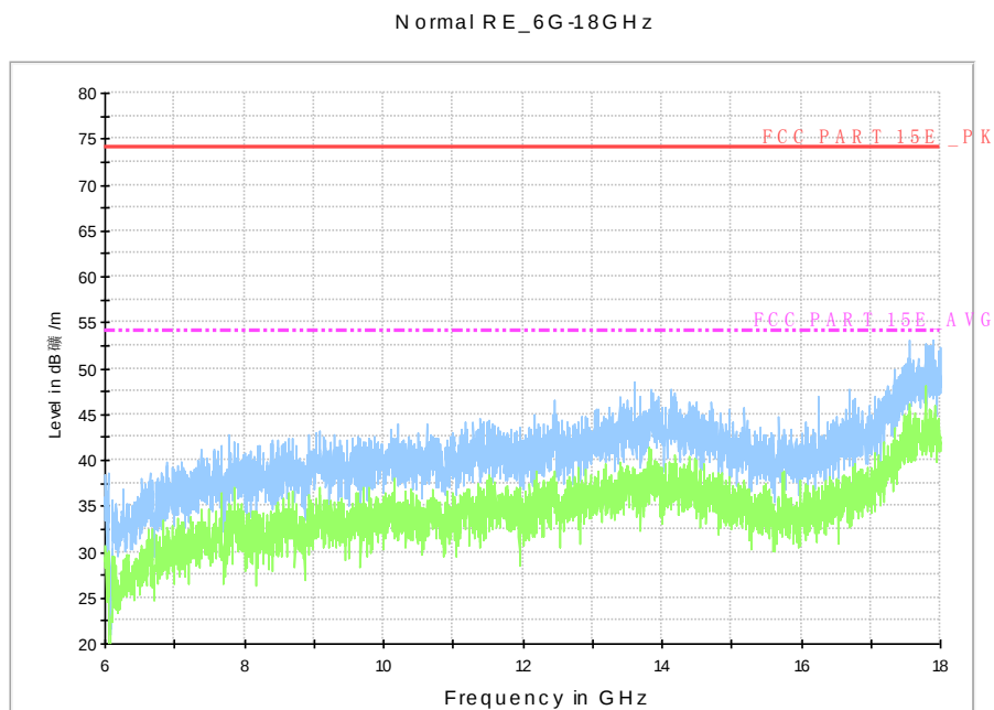
Fig. 96 Radiated Spurious Emission (802.11n-HT20, ch64, 6 GHz-18 GHz)
