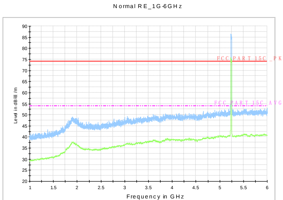
Fig. 51 Radiated Spurious Emission (802.11a, ch48, 1 GHz-6 GHz)
