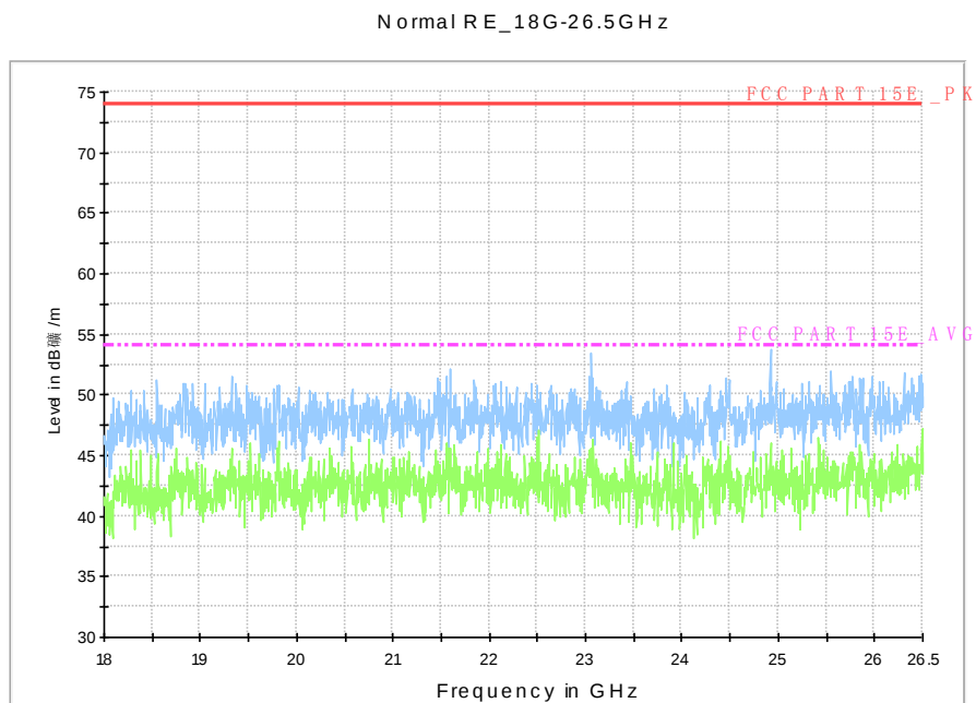
Fig. 53 Radiated Spurious Emission (802.11a, U-NII 1, 18 GHz-26.5 GHz)
