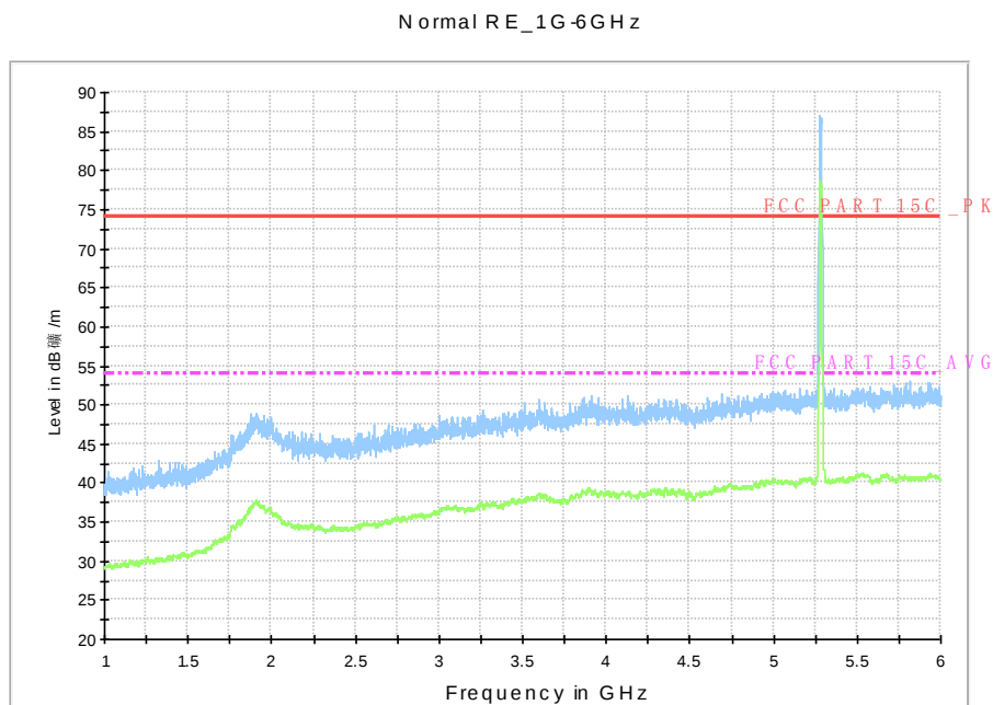
Fig. 92 Radiated Spurious Emission (802.11n-HT20, ch56, 1 GHz-6 GHz)
