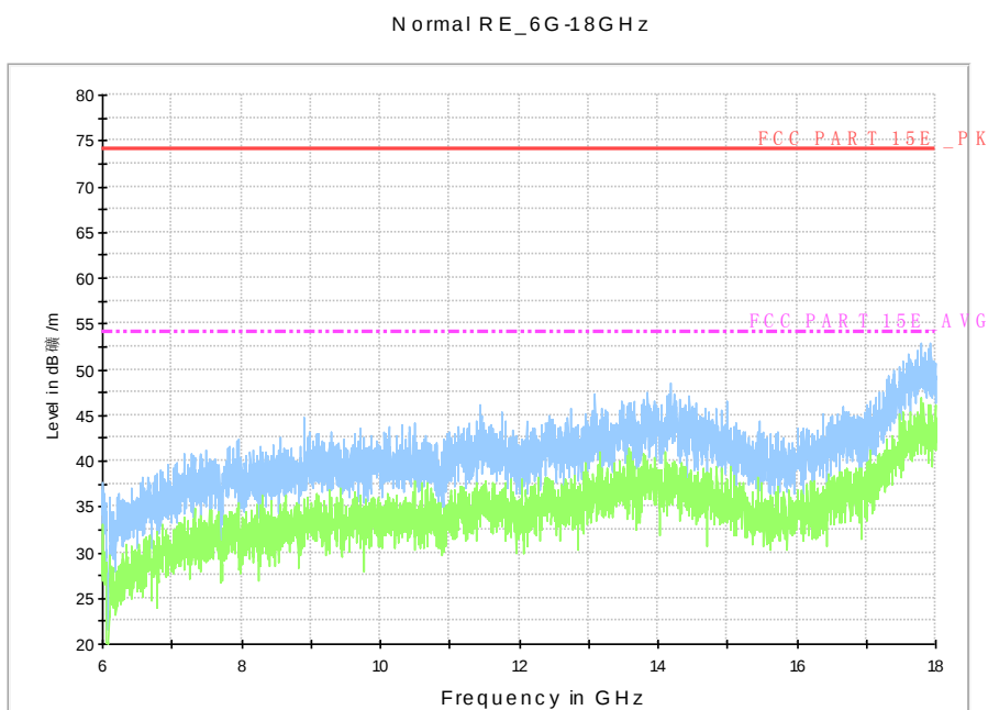
Fig. 134 Radiated Spurious Emission (802.11n-HT40, ch134, 6 GHz-18 GHz)
