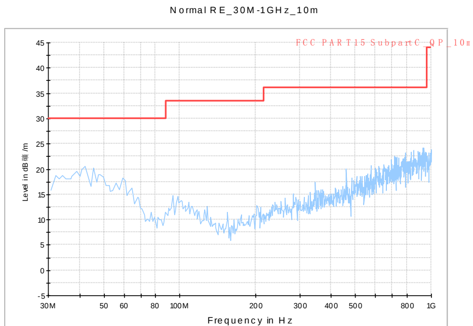
Fig. 94 Radiated Spurious Emission (802.11n-HT20, ch64, 30 MHz-1 GHz)
