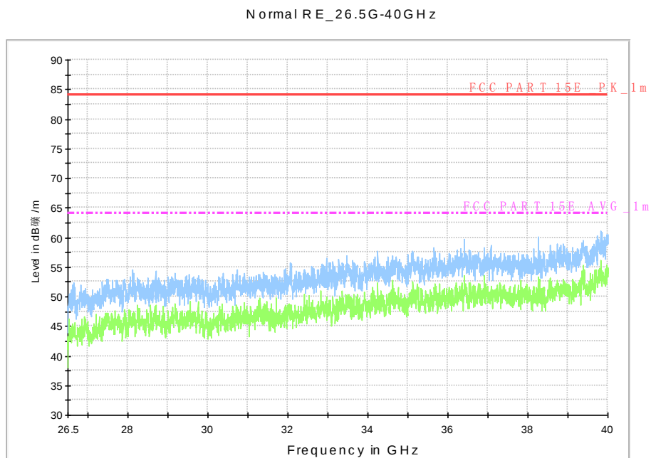
Fig. 87 Radiated Spurious Emission (802.11n-HT20, U-NII 1, 26.5 GHz-40 GHz)
