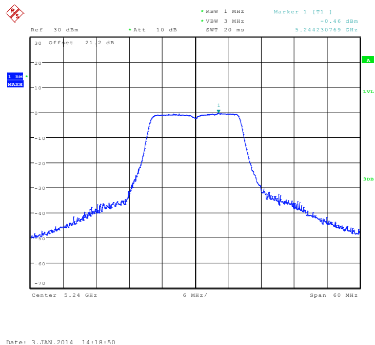
Fig. 145 Peak Excursions (802.11a, ch48, average)
