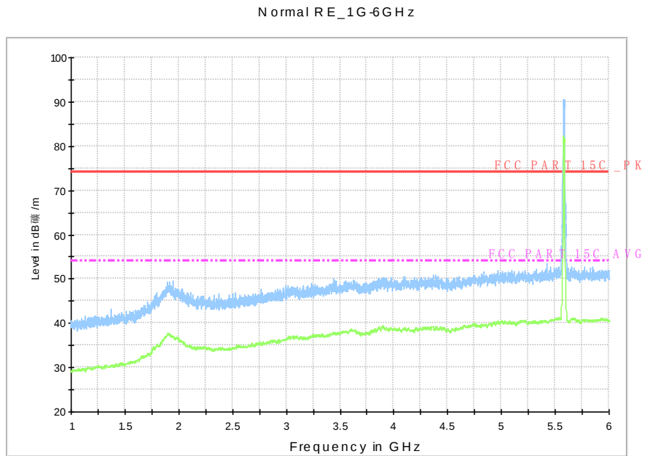
Fig. 103 Radiated Spurious Emission (802.11n-HT20, ch116, 1 GHz-6 GHz)
