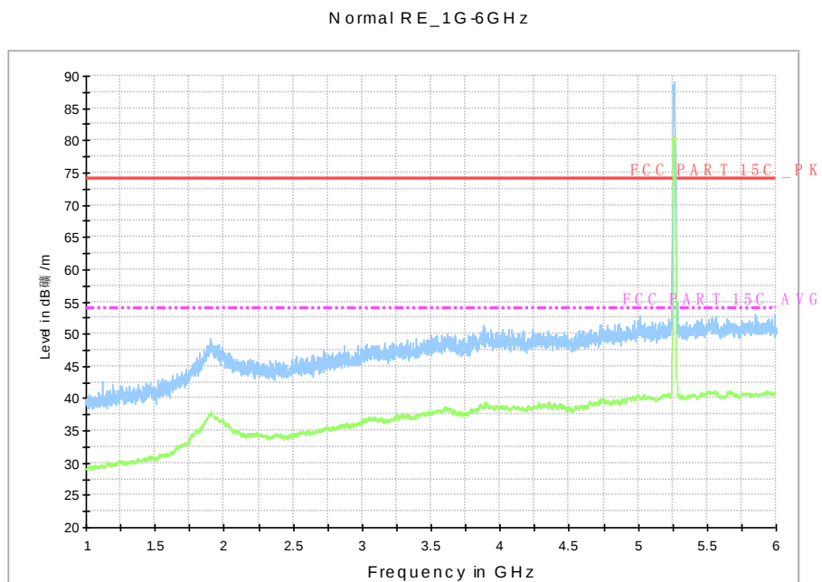
Fig. 89 Radiated Spurious Emission (802.11n-HT20, ch52, 1 GHz-6 GHz)
