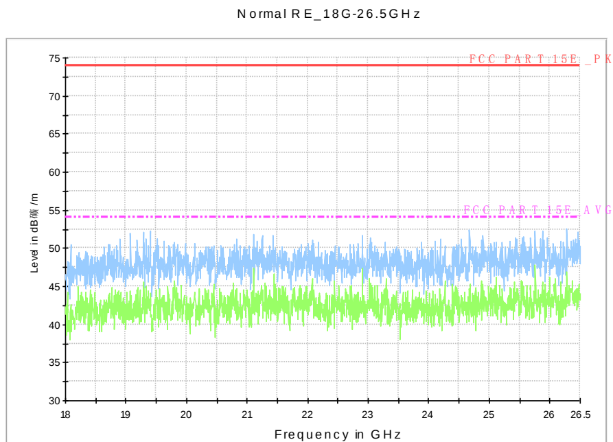
Fig. 135 Radiated Spurious Emission (802.11n-HT40, U-NII 3, 18 GHz-26.5 GHz)
