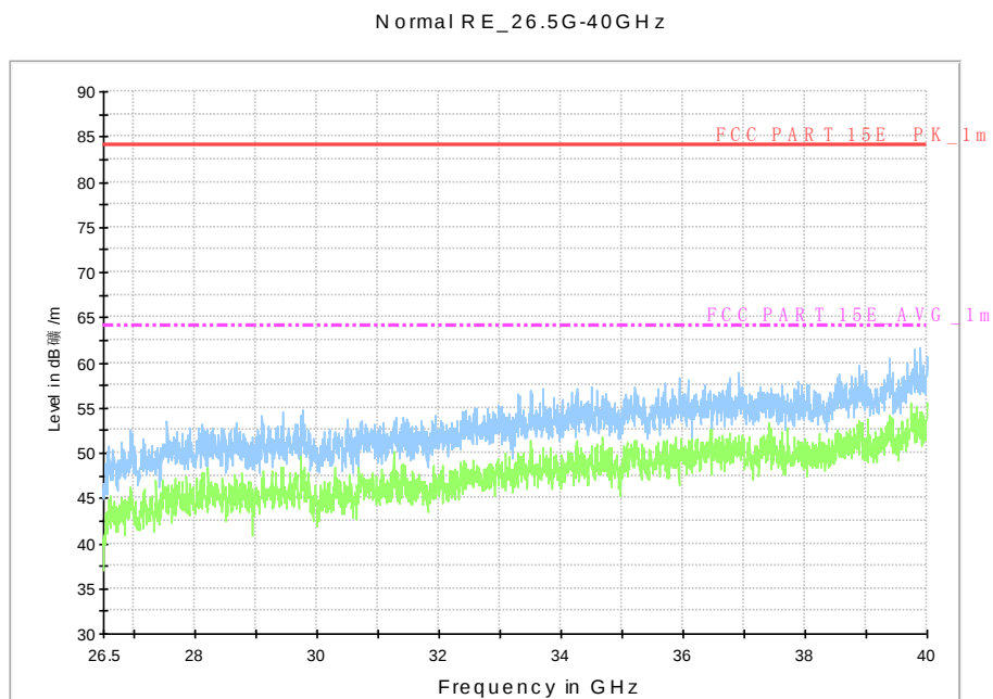
Fig. 54 Radiated Spurious Emission (802.11a, U-NII 1, 26.5 GHz-40 GHz)
