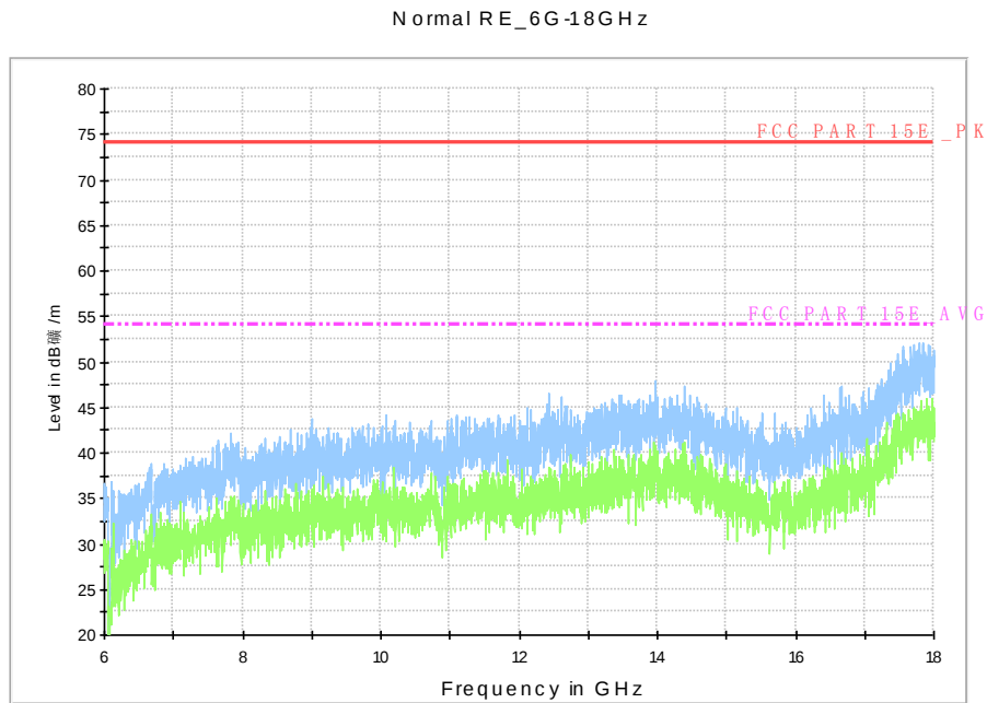
Fig. 101 Radiated Spurious Emission (802.11n-HT20, ch100, 6 GHz-18 GHz)
