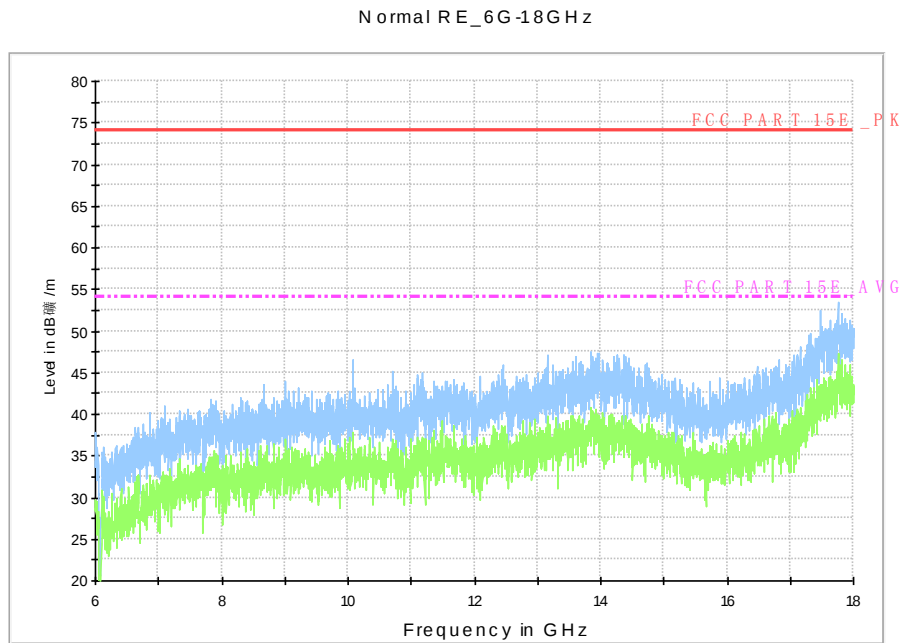
Fig. 79 Radiated Spurious Emission (802.11n-HT20, ch36, 6 GHz-18 GHz)
