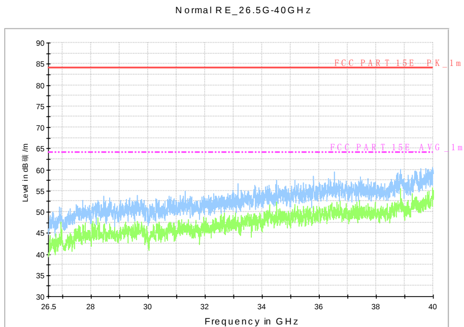
Fig. 98 Radiated Spurious Emission (802.11n-HT20, U-NII 2, 26.5 GHz-40 GHz)
