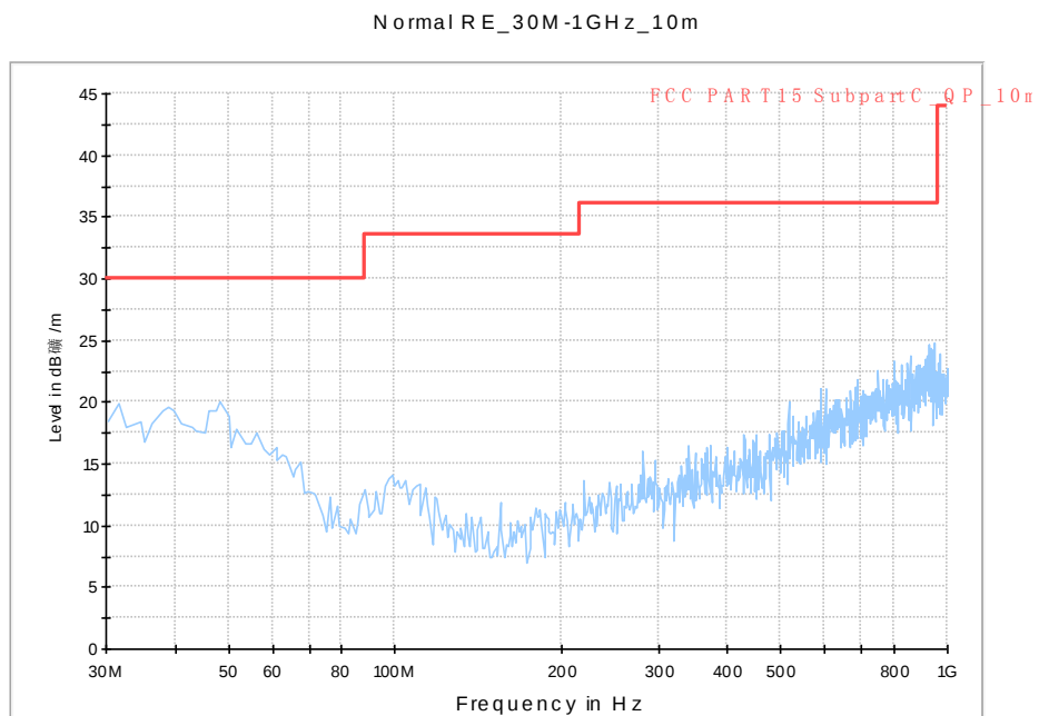
Fig. 105 Radiated Spurious Emission (802.11n-HT20, ch140, 30 MHz-1 GHz)
