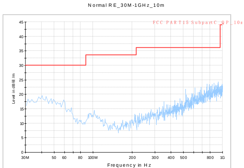
Fig. 47 Radiated Spurious Emission (802.11a, ch40, 30 MHz-1 GHz)
