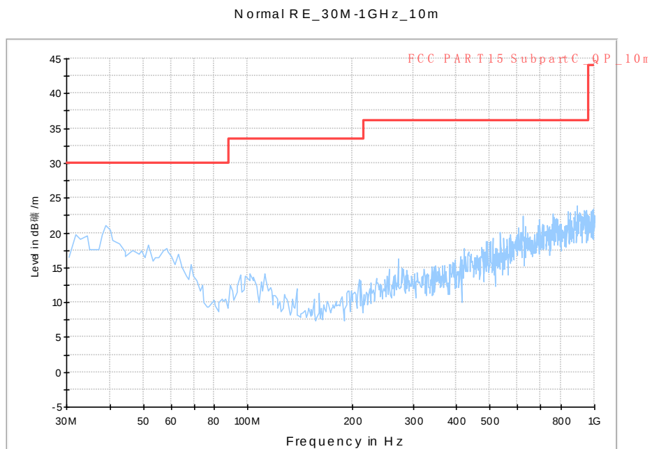
Fig. 69 Radiated Spurious Emission (802.11a, ch116, 30 MHz-1 GHz)
