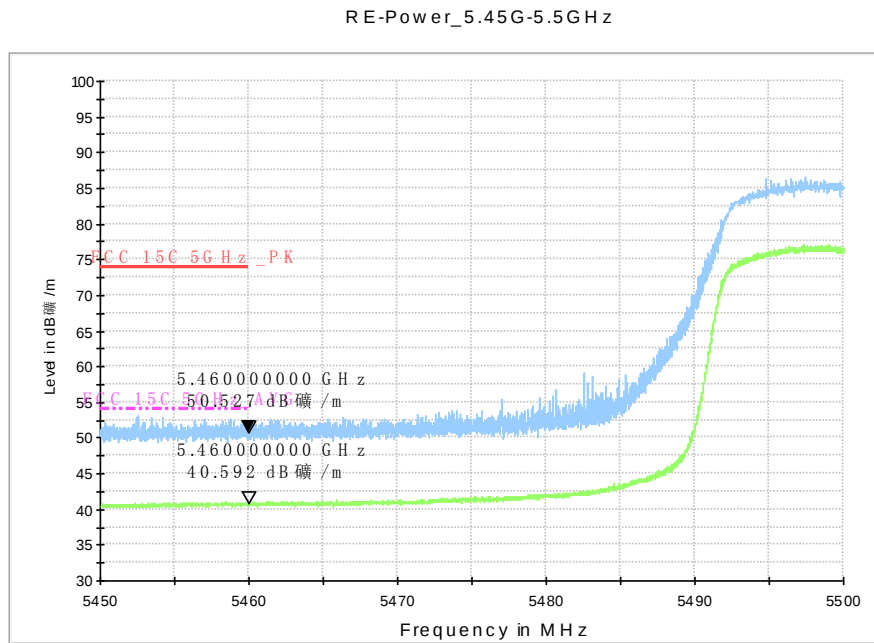
Fig. 43 Band Edges (802.11n-HT40, 5510MHz)
