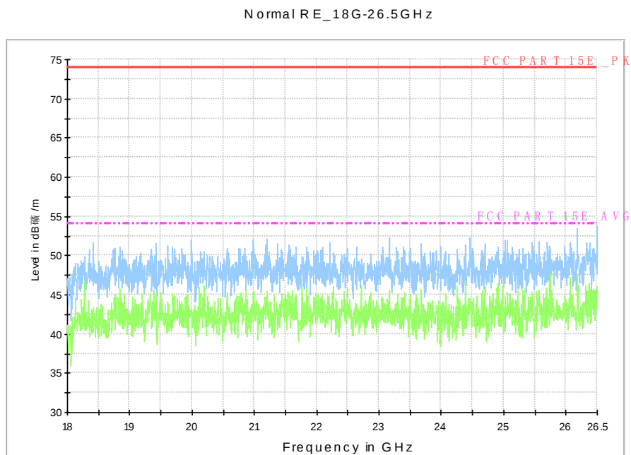
Fig. 75 Radiated Spurious Emission (802.11a, U-NII 3, 18 GHz-26.5 GHz)
