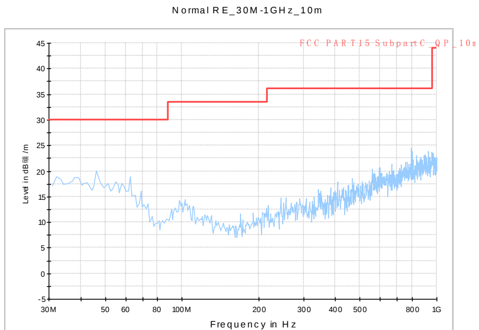
Fig. 129 Radiated Spurious Emission (802.11n-HT40, ch110, 30 MHz-1 GHz)
