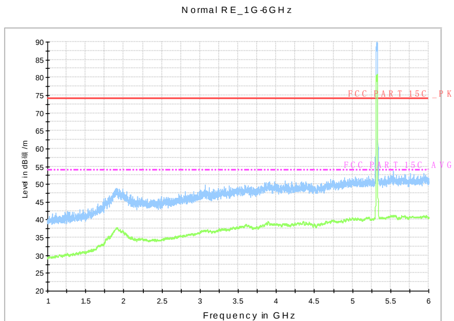
Fig. 95 Radiated Spurious Emission (802.11n-HT20, ch64, 1 GHz-6 GHz)
