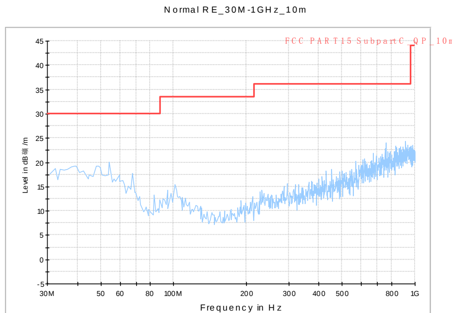
Fig. 50 Radiated Spurious Emission (802.11a, ch48, 30 MHz-1 GHz)
