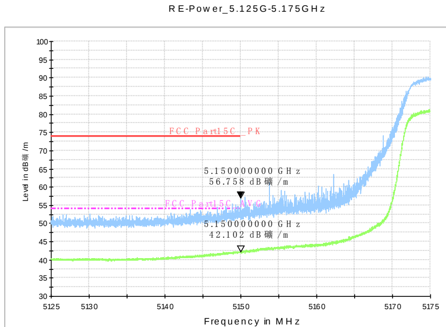
Fig. 41 Band Edges (802.11n-HT40, 5190MHz)
