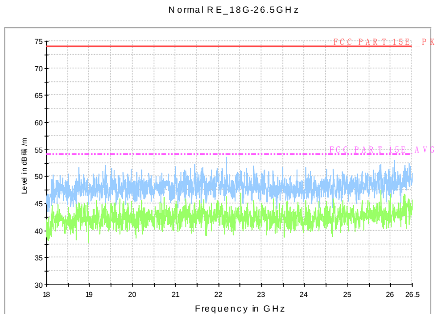
Fig. 108 Radiated Spurious Emission (802.11n-HT20, U-NII 3, 18 GHz-26.5 GHz)
