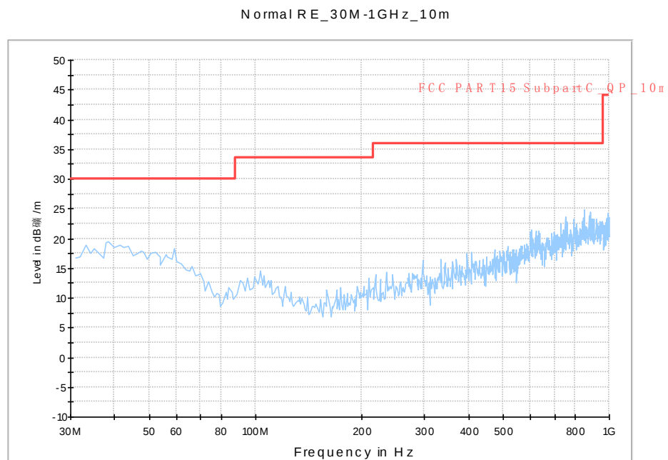
Fig. 61 Radiated Spurious Emission (802.11a, ch64, 30 MHz-1 GHz)
