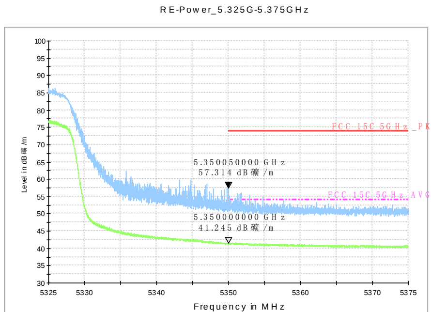
Fig. 42 Band Edges (802.11n-HT40, 5310MHz)
