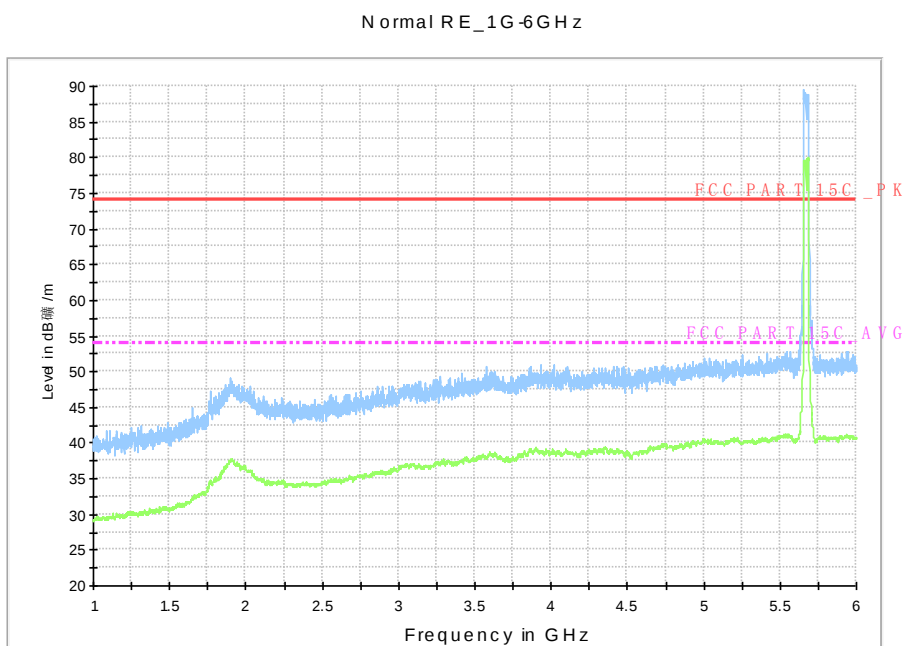
Fig. 133 Radiated Spurious Emission (802.11n-HT40, ch134, 1 GHz-6 GHz)
