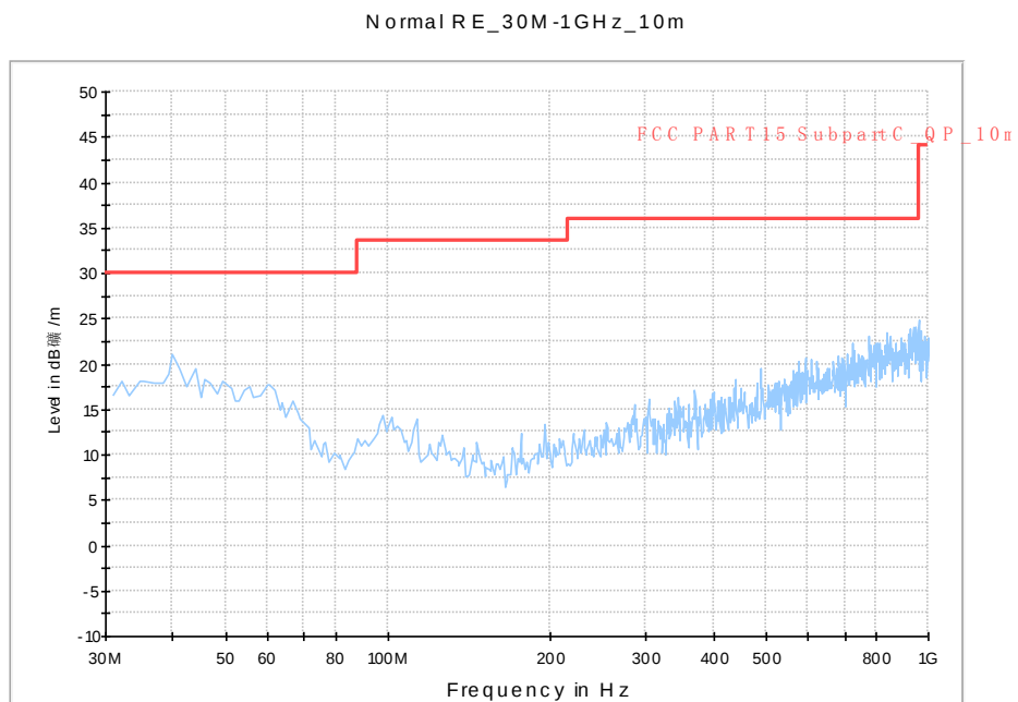
Fig. 83 Radiated Spurious Emission (802.11n-HT20, ch48, 30 MHz-1 GHz)
