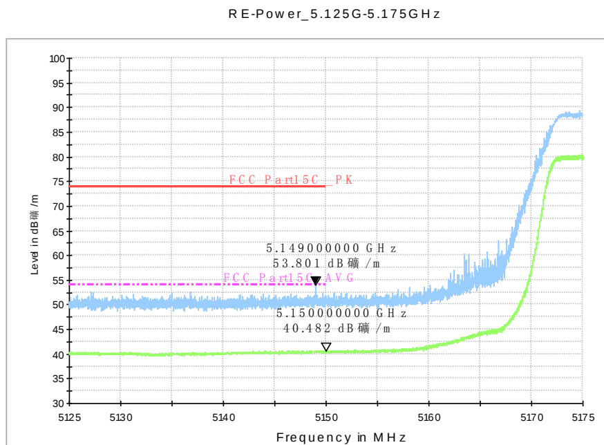
Fig. 35 Band Edges (802.11a, 5180MHz)
