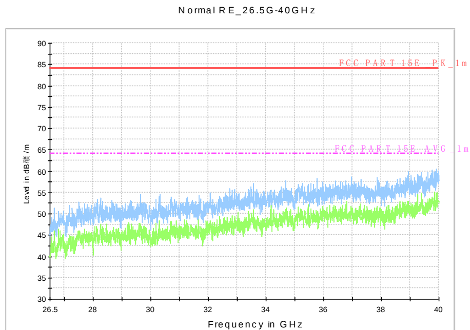
Fig. 109 Radiated Spurious Emission (802.11n-HT20, U-NII 3, 26.5 GHz-40 GHz)
