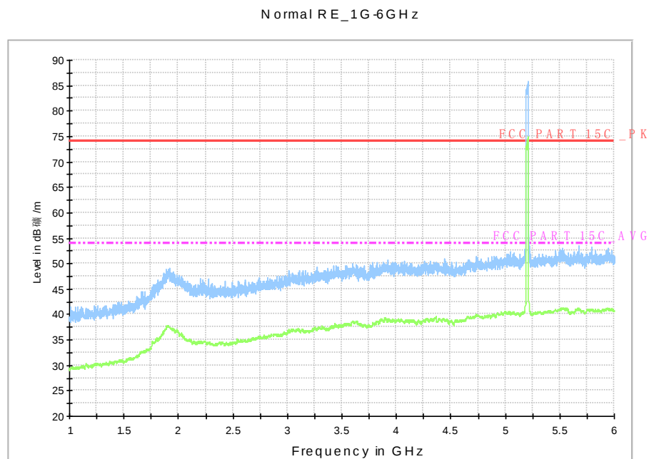
Fig. 48 Radiated Spurious Emission (802.11a, ch40, 1 GHz-6 GHz)
