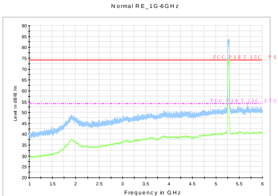
Fig. 119 Radiated Spurious Emission (802.11n-HT40, ch54, 1 GHz-6 GHz)
