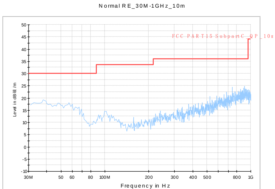
Fig. 113 Radiated Spurious Emission (802.11n-HT40, ch46, 30 MHz-1 GHz)
