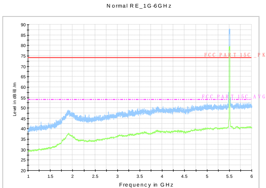
Fig. 100 Radiated Spurious Emission (802.11n-HT20, ch100, 1 GHz-6 GHz)
