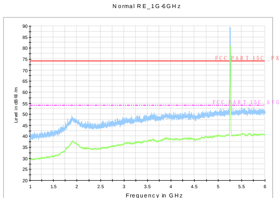
Fig. 56 Radiated Spurious Emission (802.11a, ch52, 1 GHz-6 GHz)
