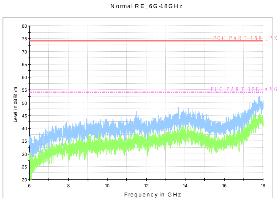
Fig. 60 Radiated Spurious Emission (802.11a, ch56, 6 GHz-18 GHz)
