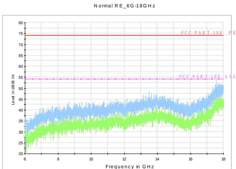
Fig. 115 Radiated Spurious Emission (802.11n-HT40, ch46, 6 GHz-18 GHz)
