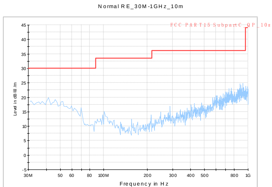
Fig. 126 Radiated Spurious Emission (802.11n-HT40, ch102, 30 MHz-1 GHz)
