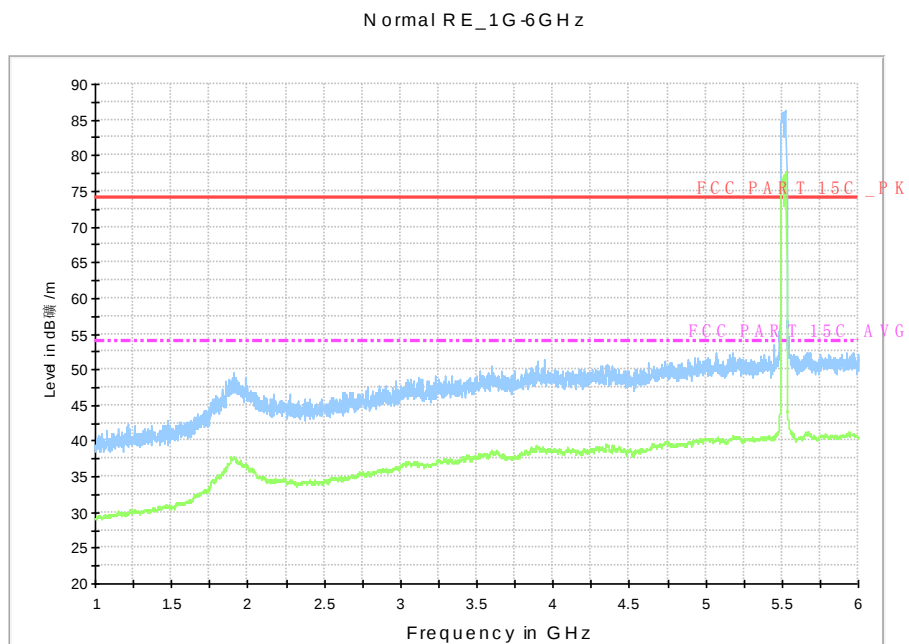
Fig. 127 Radiated Spurious Emission (802.11n-HT40, ch102, 1 GHz-6 GHz)
