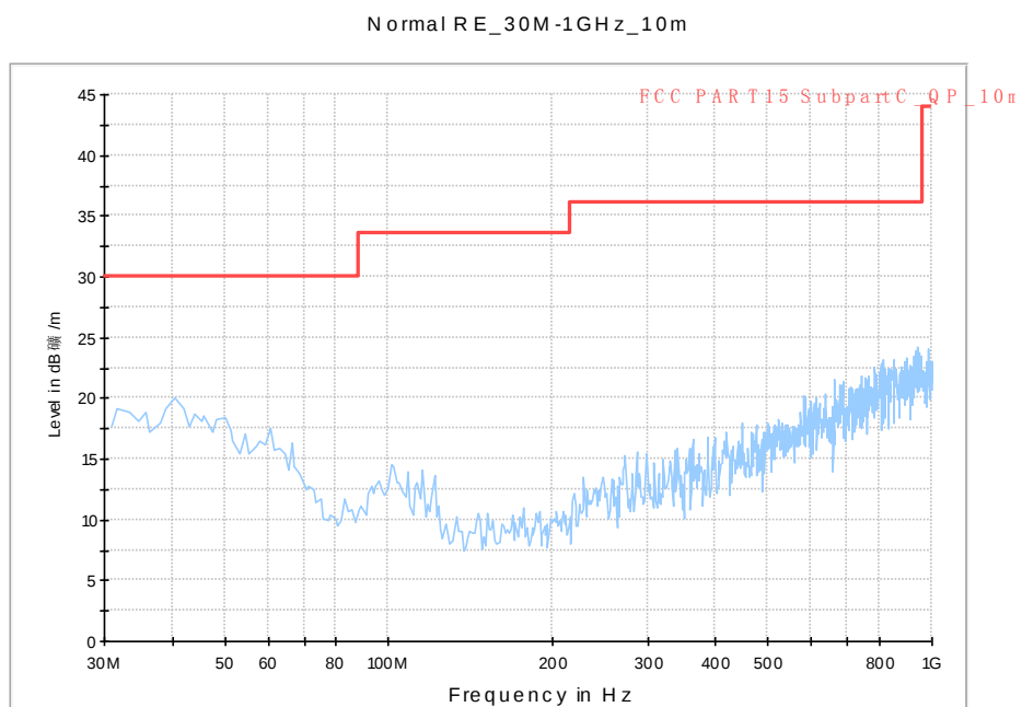
Fig. 88 Radiated Spurious Emission (802.11n-HT20, ch52, 30 MHz-1 GHz)
