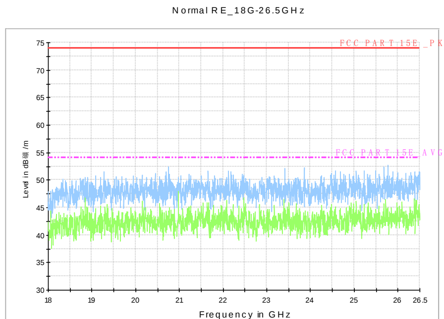
Fig. 86 Radiated Spurious Emission (802.11n-HT20, U-NII 1, 18 GHz-26.5 GHz)
