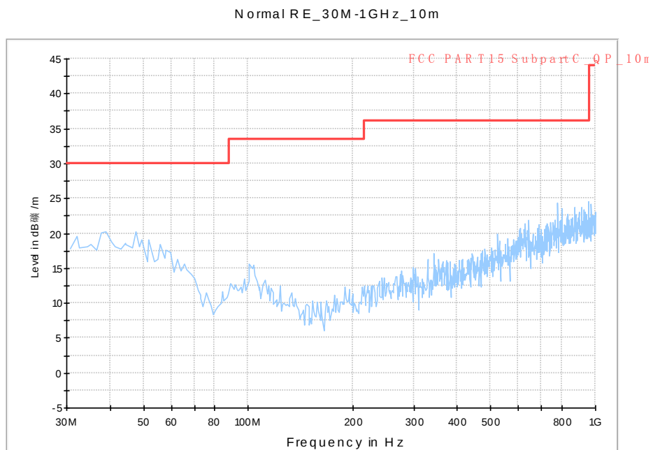
Fig. 121 Radiated Spurious Emission (802.11n-HT40, ch62, 30 MHz-1 GHz)
