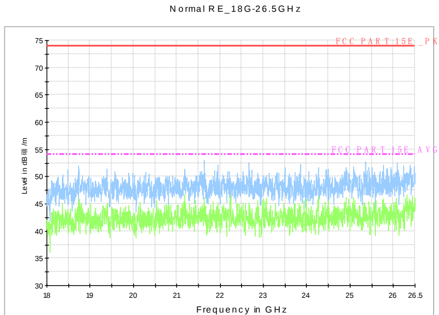
Fig. 124 Radiated Spurious Emission (802.11n-HT40, U-NII 2, 18 GHz-26.5 GHz)
