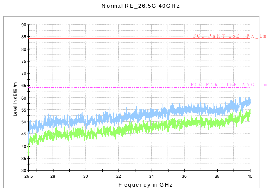
Fig. 65 Radiated Spurious Emission (802.11a, U-NII 2, 26.5 GHz-40 GHz)
