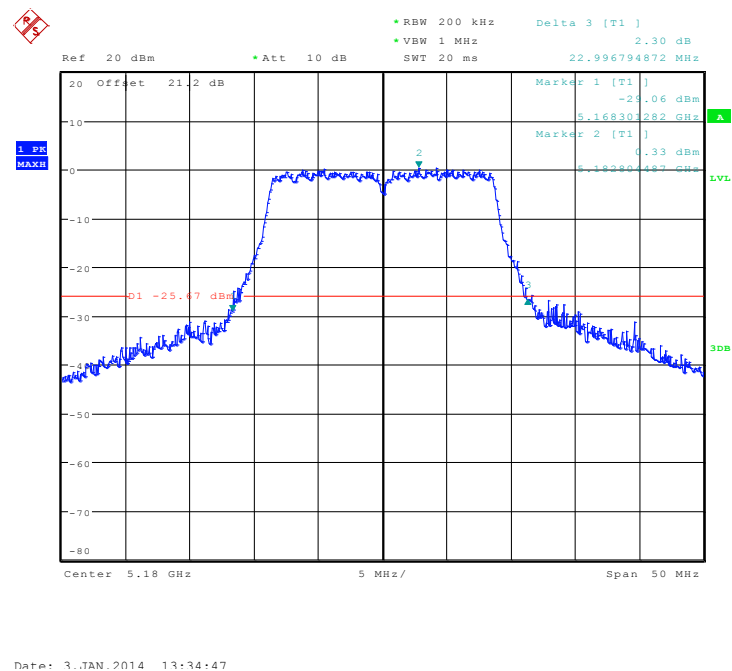
Fig. 10 Occupied 26dB Bandwidth (802.11n-HT20, 5180MHz)
