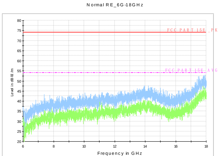
Fig. 82 Radiated Spurious Emission (802.11n-HT20, ch40, 6 GHz-18 GHz)
