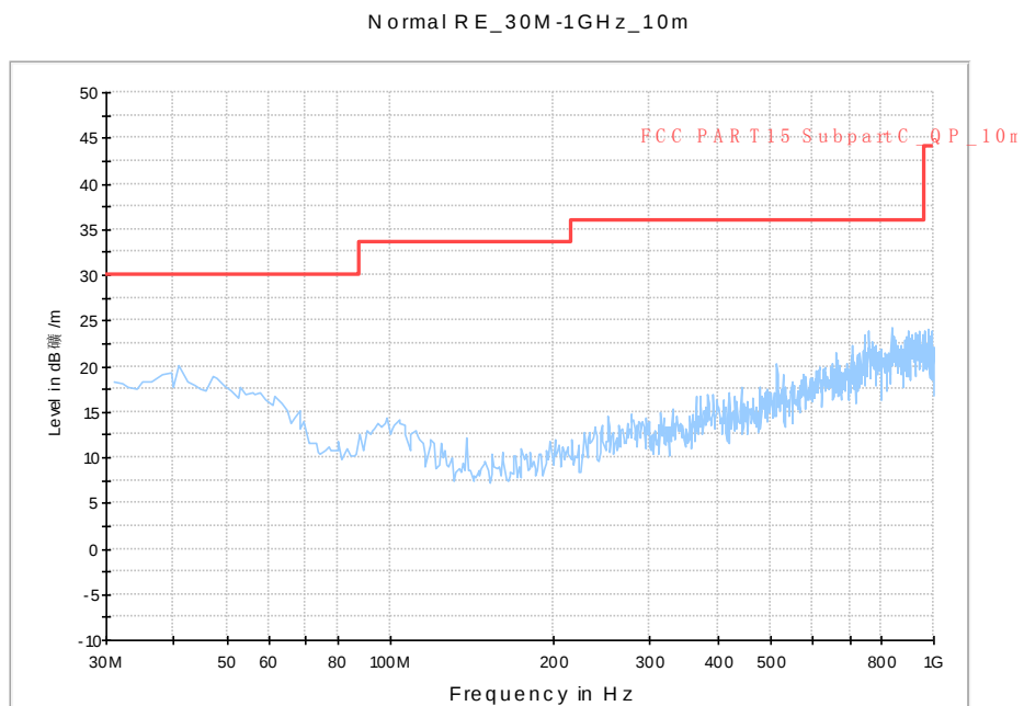
Fig. 80 Radiated Spurious Emission (802.11n-HT20, ch40, 30 MHz-1 GHz)
