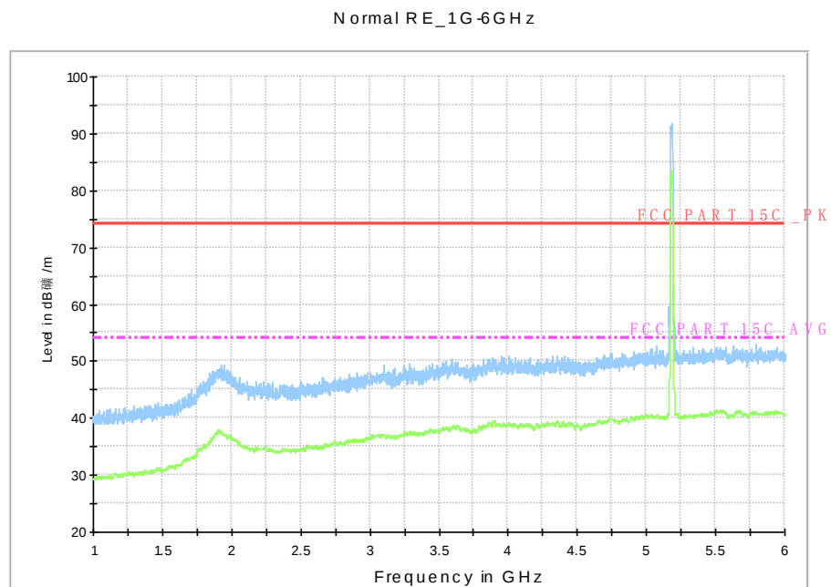
Fig. 45 Radiated Spurious Emission (802.11a, ch36, 1 GHz-6 GHz)
