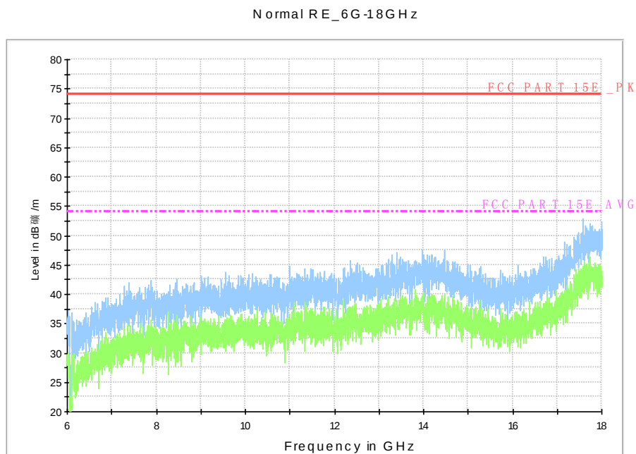
Fig. 120 Radiated Spurious Emission (802.11n-HT40, ch54, 6 GHz-18 GHz)
