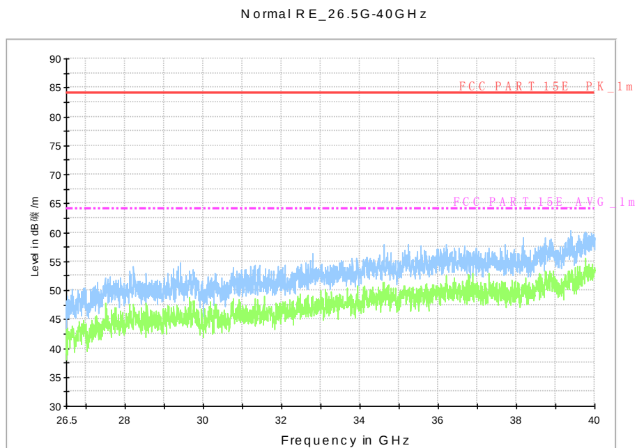
Fig. 136 Radiated Spurious Emission (802.11n-HT40, U-NII 3, 26.5 GHz-40 GHz)
