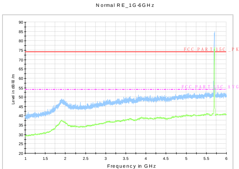
Fig. 106 Radiated Spurious Emission (802.11n-HT20, ch140, 1 GHz-6 GHz)
