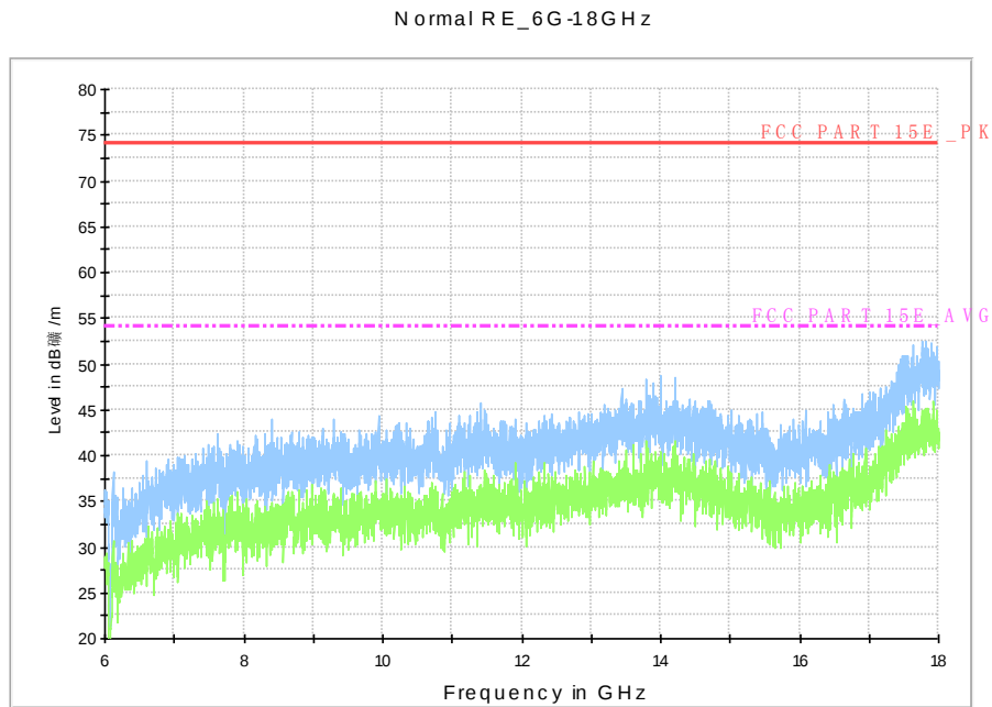
Fig. 123 Radiated Spurious Emission (802.11n-HT40, ch62, 6 GHz-18 GHz)
