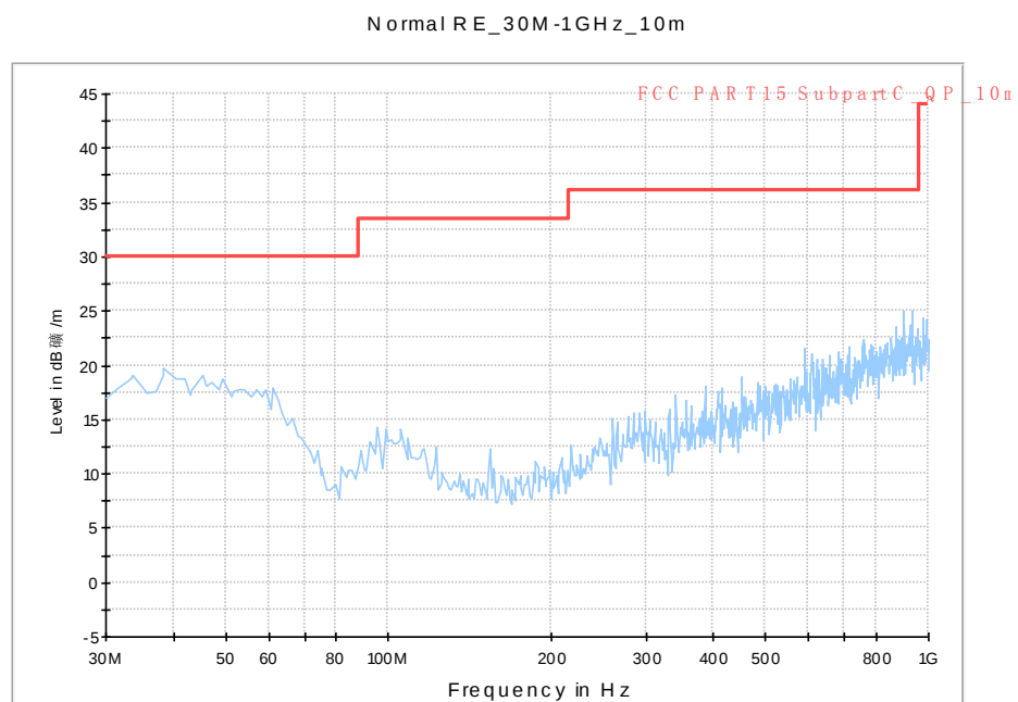
Fig. 66 Radiated Spurious Emission (802.11a, ch100, 30 MHz-1 GHz)
