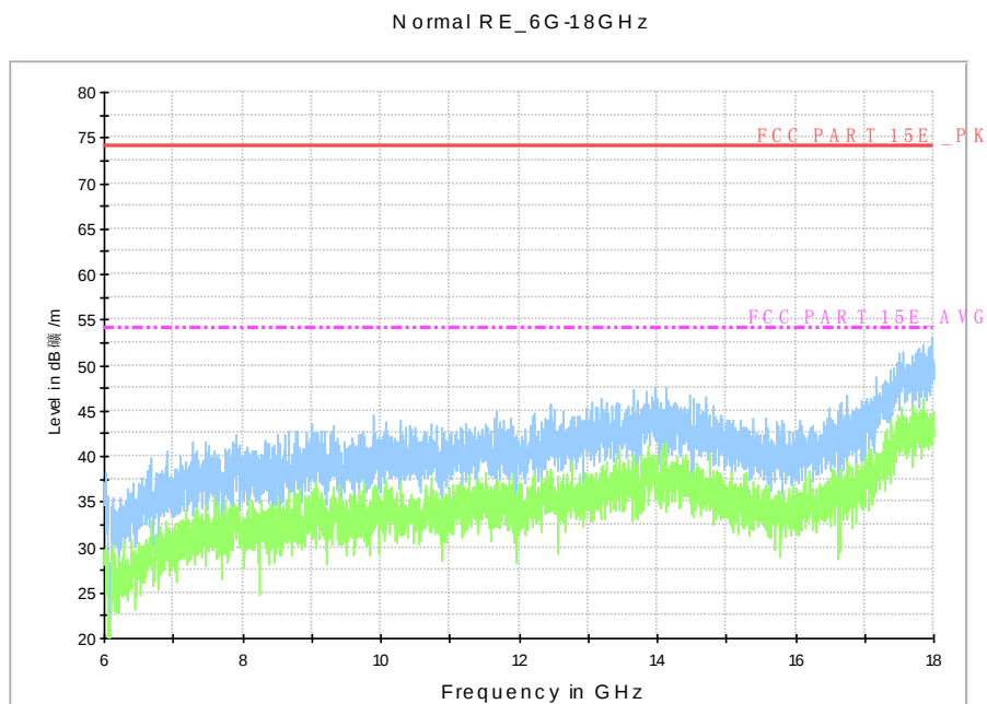
Fig. 68 Radiated Spurious Emission (802.11a, ch100, 6 GHz-18 GHz)
