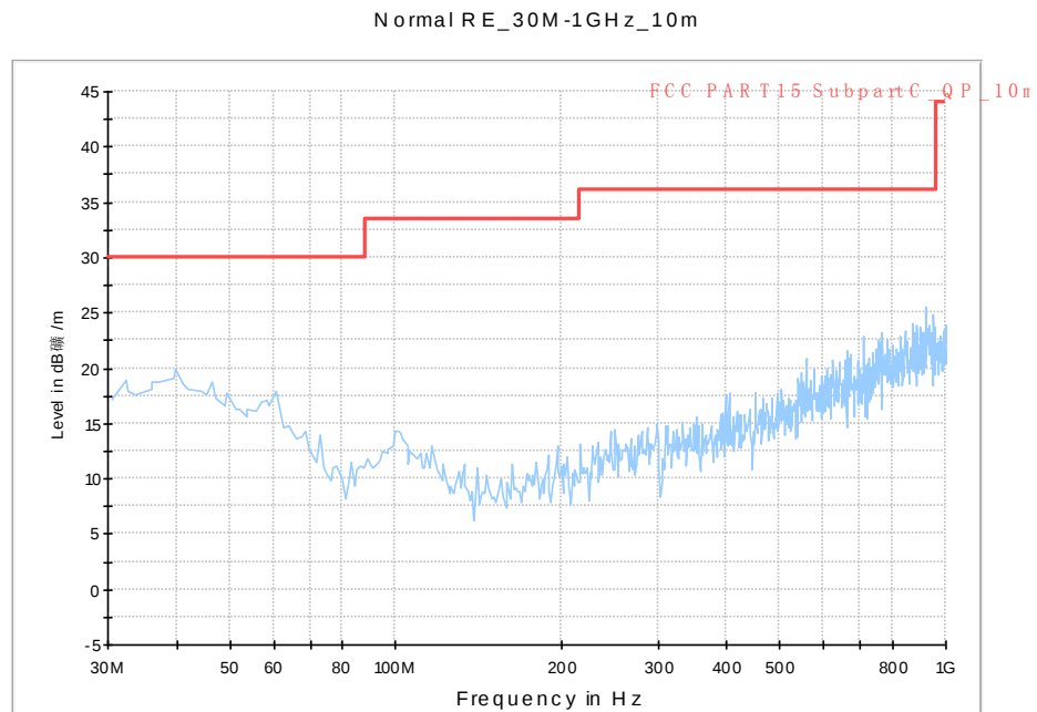
Fig. 44 Radiated Spurious Emission (802.11a, ch36, 30 MHz-1 GHz)
