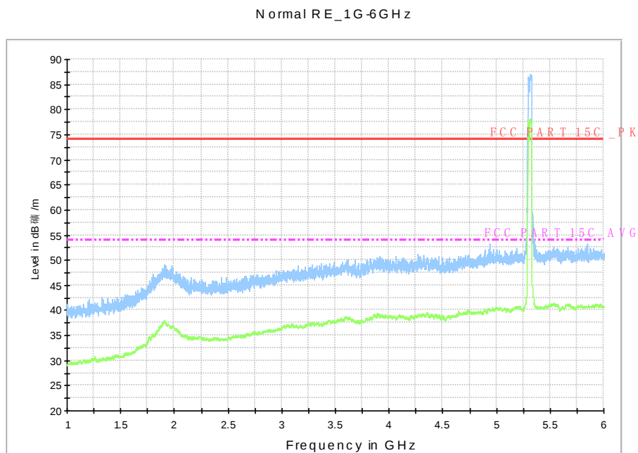
Fig. 122 Radiated Spurious Emission (802.11n-HT40, ch62, 1 GHz-6 GHz)
