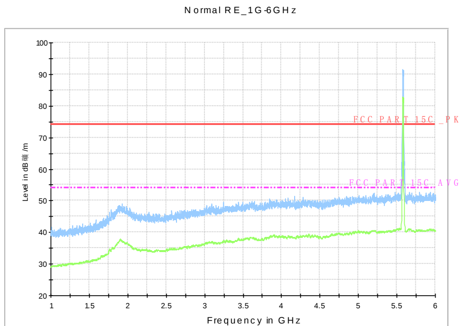
Fig. 70 Radiated Spurious Emission (802.11a, ch116, 1 GHz-6 GHz)
